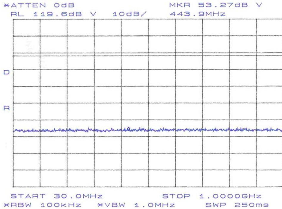
Figure 7. Conducted Spurious Emissions; Ch 1, 30MHz - 1GHz
