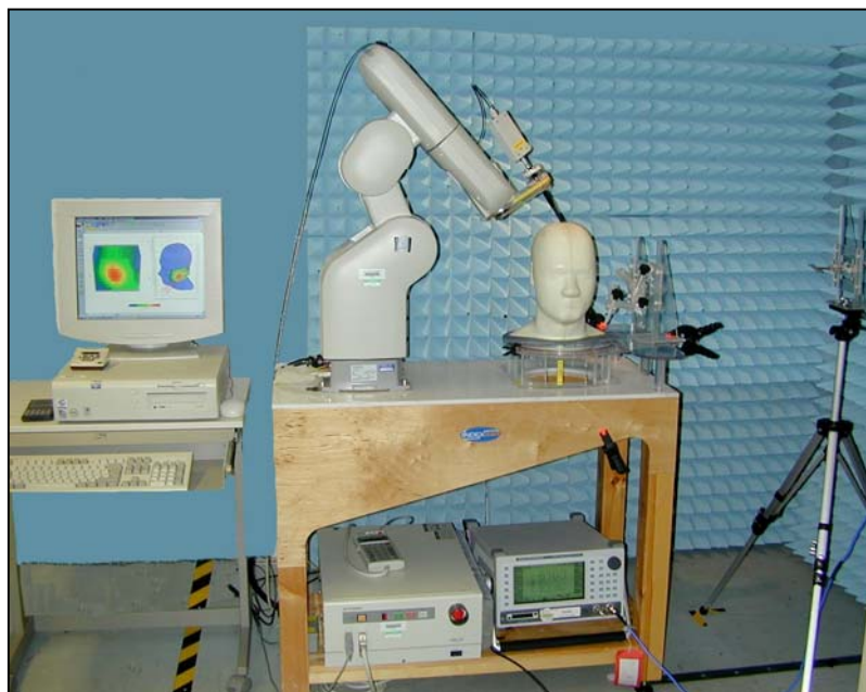
Figure 13: Principal components of the SAR measurement test bench
