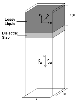
Figure 5. Geometry used for waveguide calibration (after Ref [2]. Section A.3.2.2)
