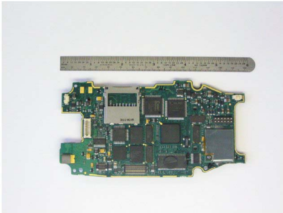
MAIN BOARD TOP SIDE (WITHOUT 802.11b ANTENNA, SOCKET RADIO)
