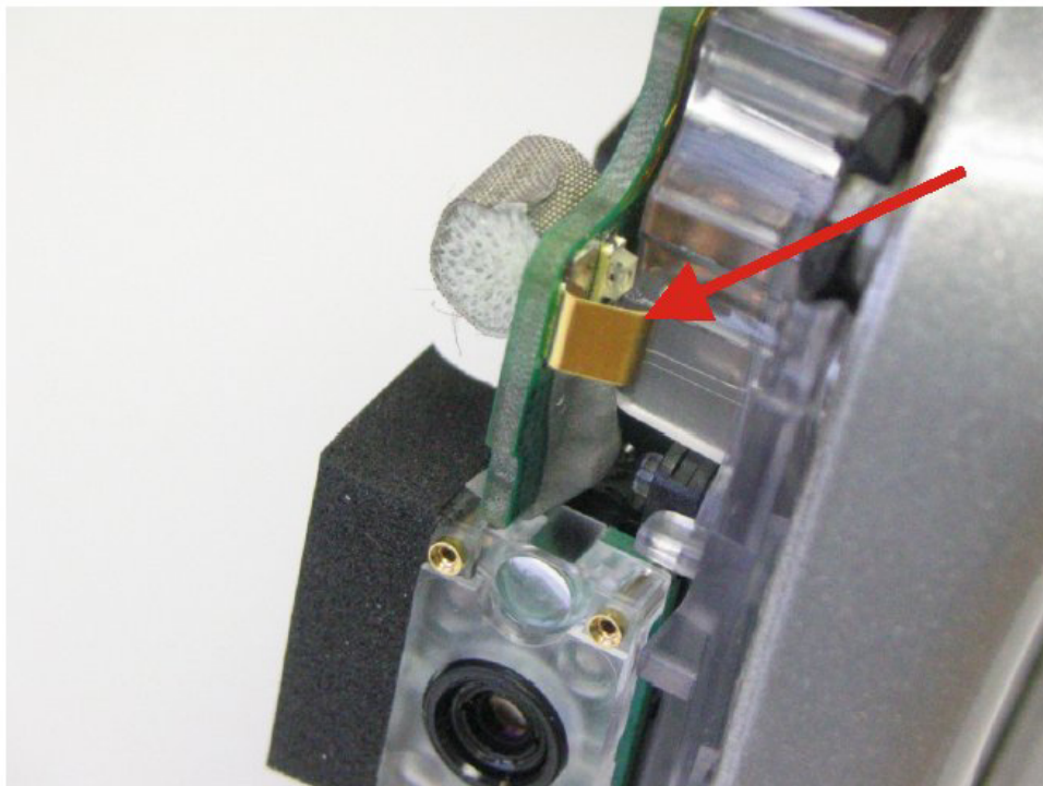
CONTACT FOR GSM ANTENNA
