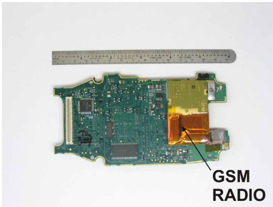
MAIN BOARD BOTTOM SIDE
