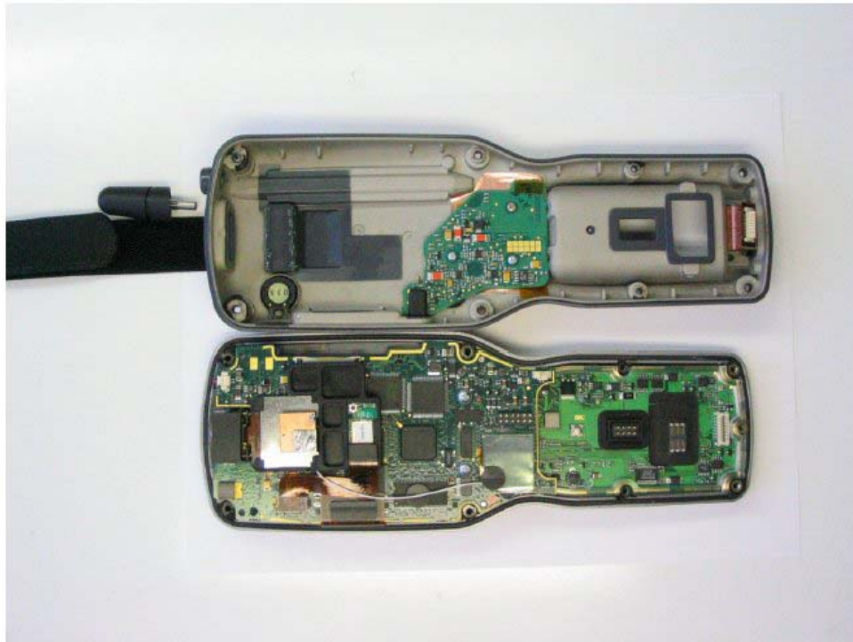
DISASSEMBLED HOUSINGS (WITH GSM ANTENNA)
