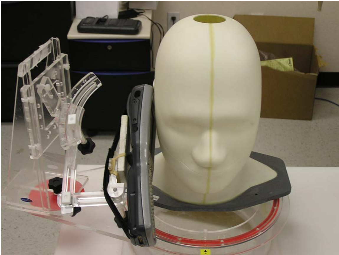
Photo 6 Right tilt
