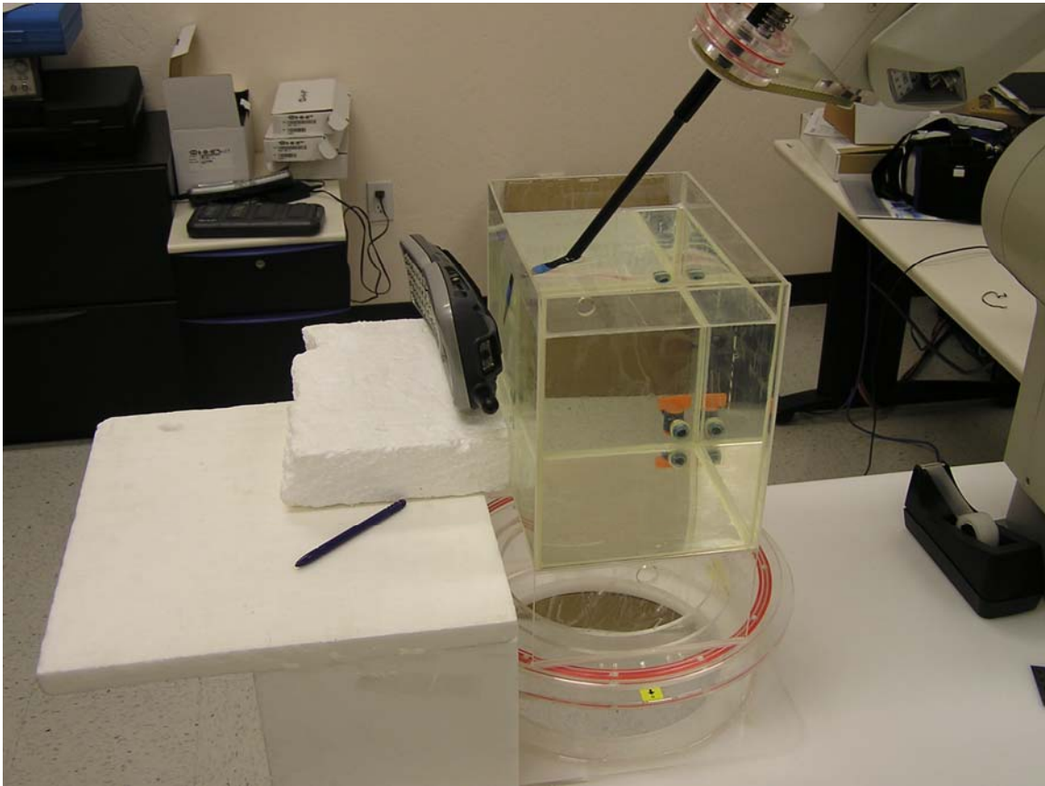
Photo 7 Body SAR
