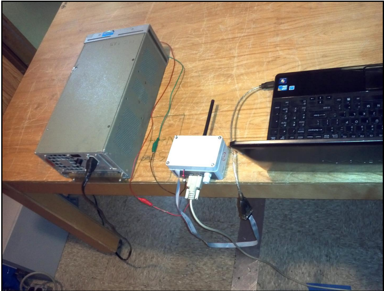
Photograph 6: Conducted AC Testing – Rear View
