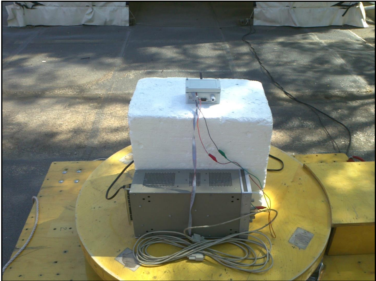
Photograph 4: Radiated Testing – Rear View
