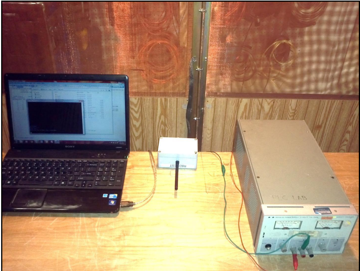
Photograph 5: Conducted AC Testing – Front View
