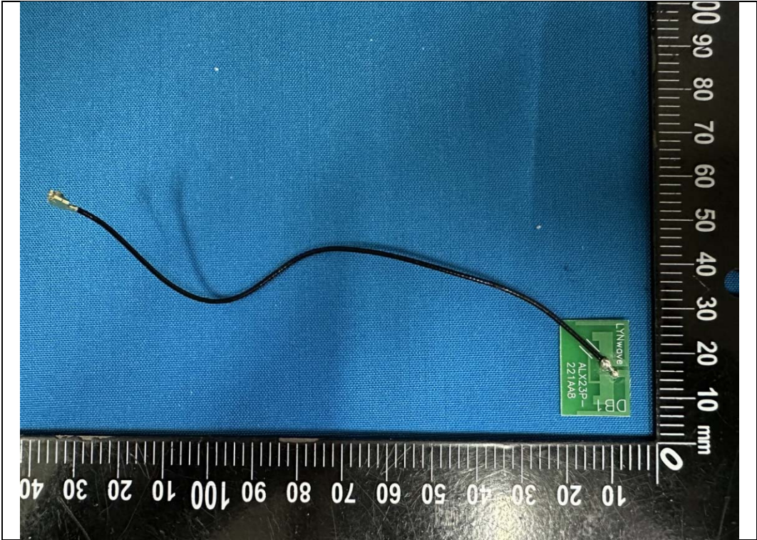
2.4G+5G Antenna 0
