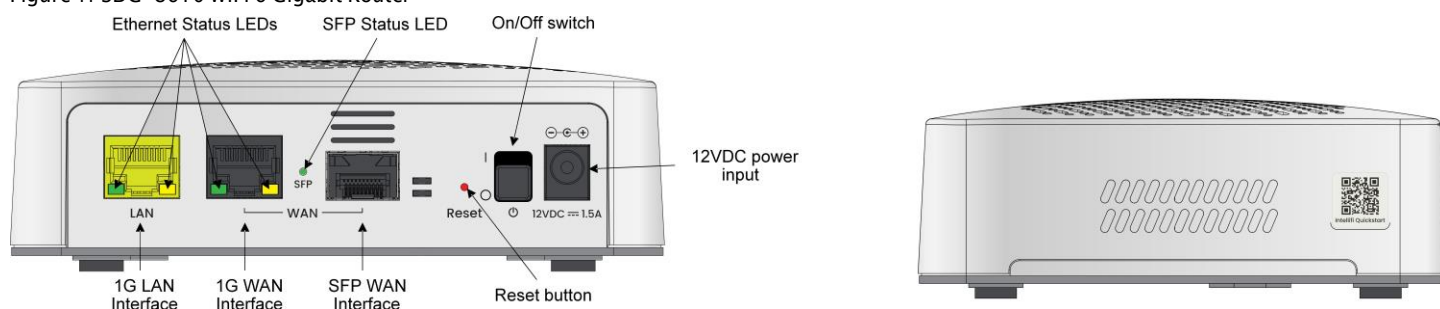
Figure 1: SDG-8610 WiFi 6 Gigabit Router
