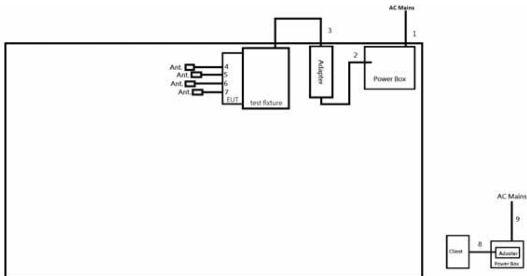
Test Setup Diagram – AC Line Conducted Emission Test (Beamforming)
