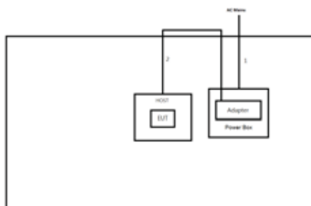
Test Setup Diagram - Radiated Test Below 1GHz
