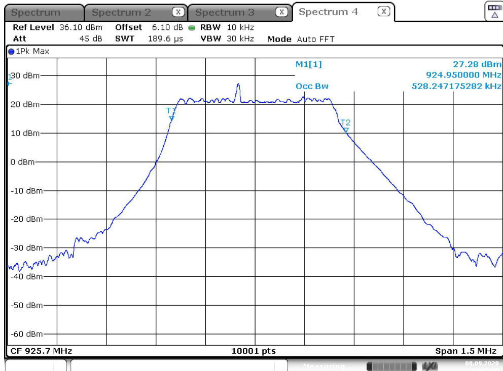
Sample Plot – 99% OBW (SF8 MCH)
