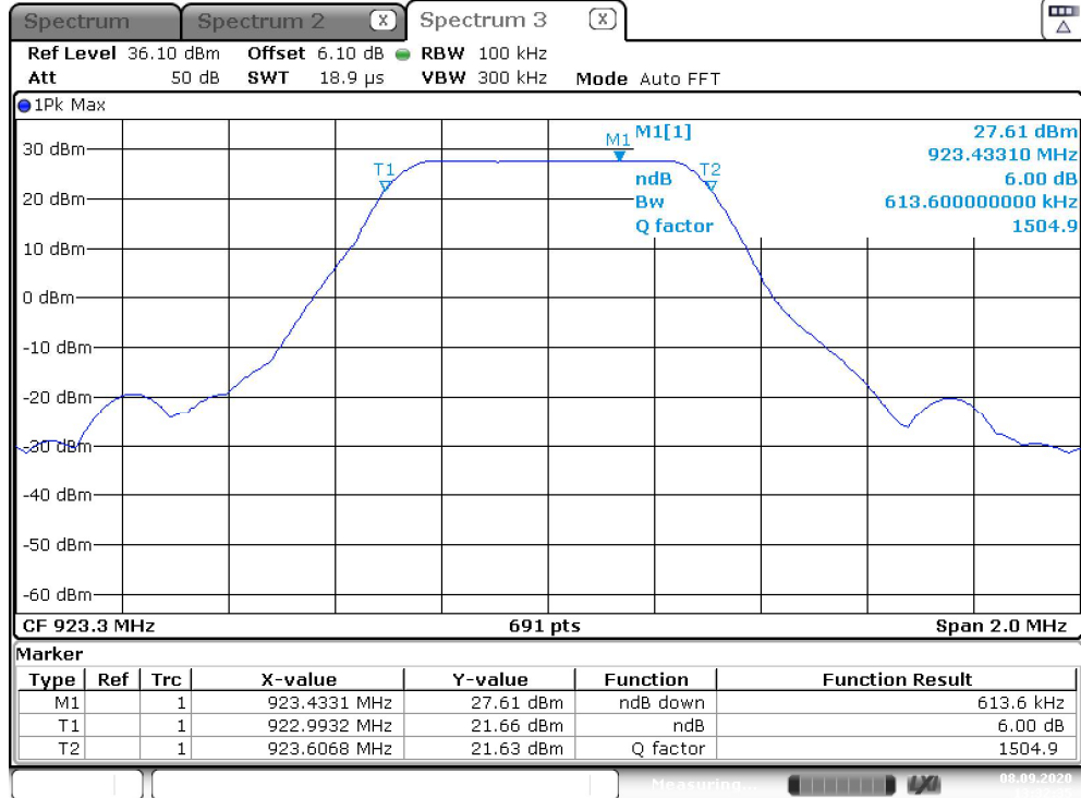
Sample Plot – 6dB BW (SF7 LCH)
