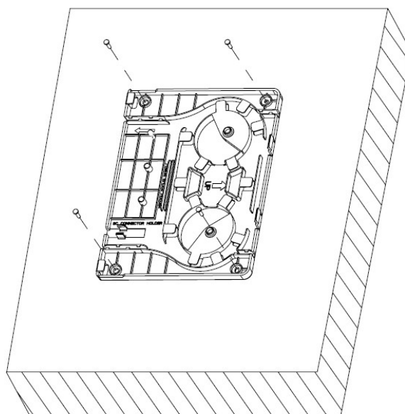
Figure 5 Mount the bracket into the wall
