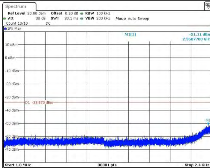
11N20SISO_Ant3_2462_1~2400
