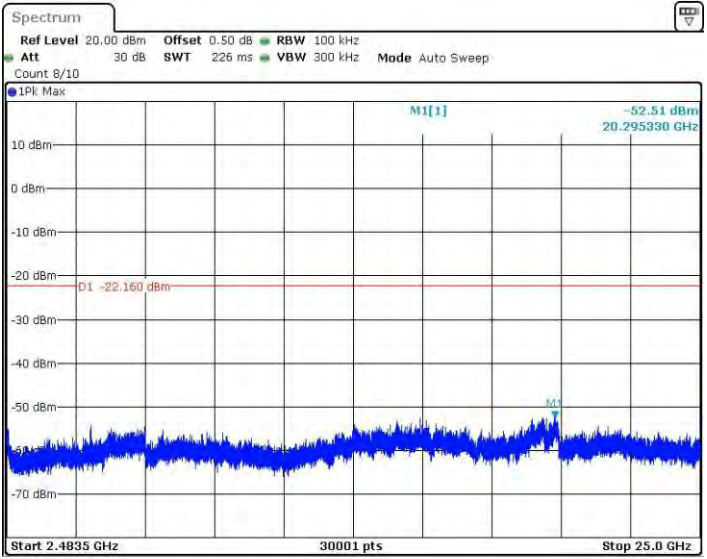
11GMINO_Ant3_2412_2483.5~25000
