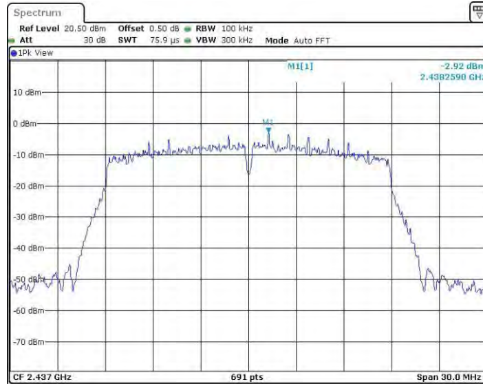
11N20SISO_Ant4_2437_0~Reference
