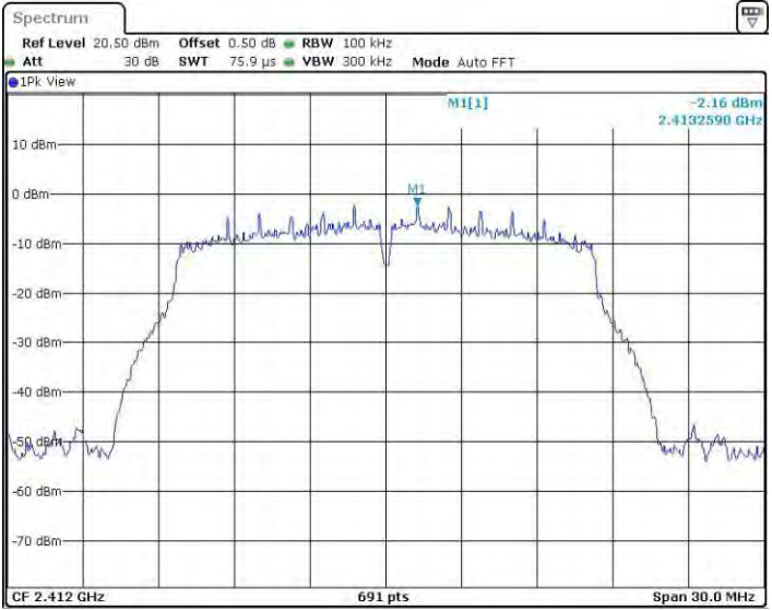
11GMINO_Ant3_2412_0~Reference
