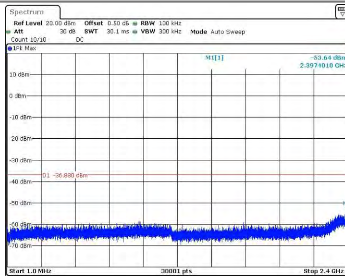
11N40SISO_Ant2_2437_0~Reference
