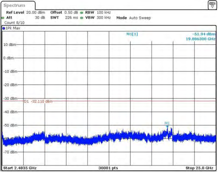
11G_Ant4_2437_2483.5~25000
