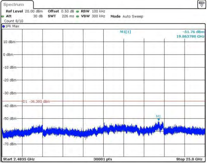
11N40SISO_Ant4_2422_2483.5~25000
