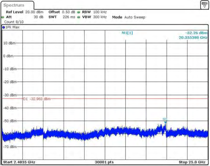
11N20SISO_Ant1_2412_2483.5~25000
