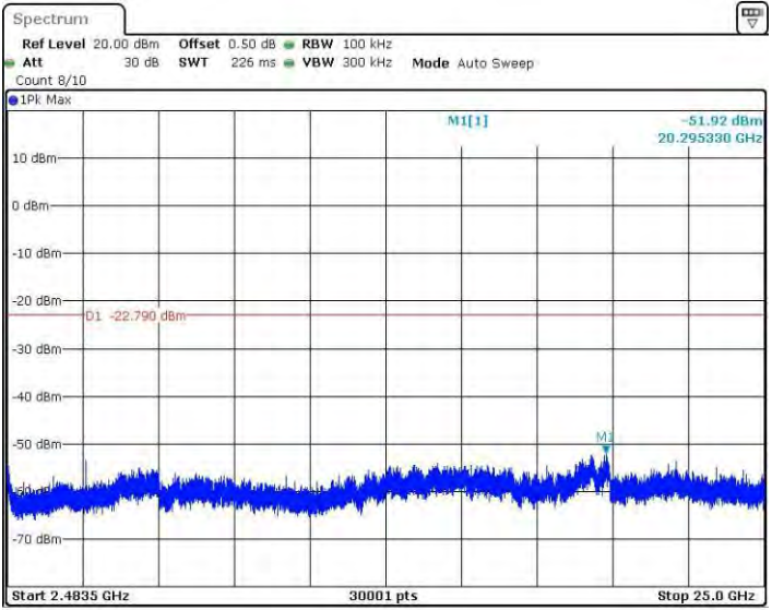
11B_Ant4_2412_2483.5~25000
