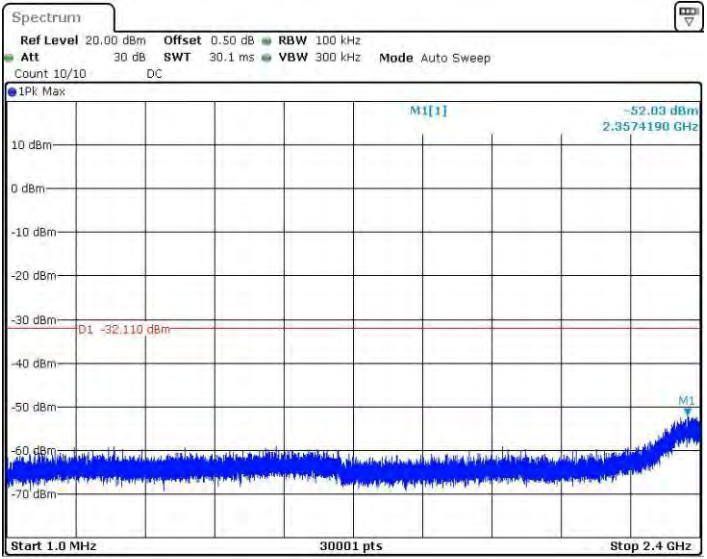
11G_Ant4_2437_1~2400
