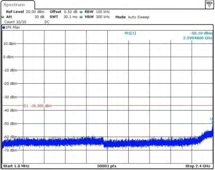
11N40SISO_Ant4_2422_1~2400
