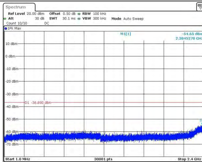
11N40SISO_Ant4_2452_0~Reference
