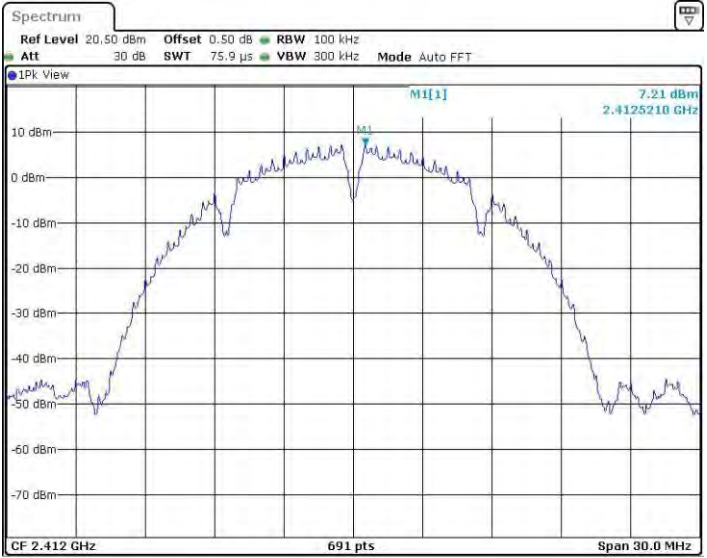
11B_Ant4_2412_0~Reference
