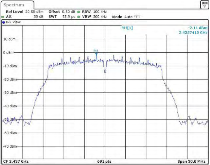
11G_Ant4_2437_0~Reference
