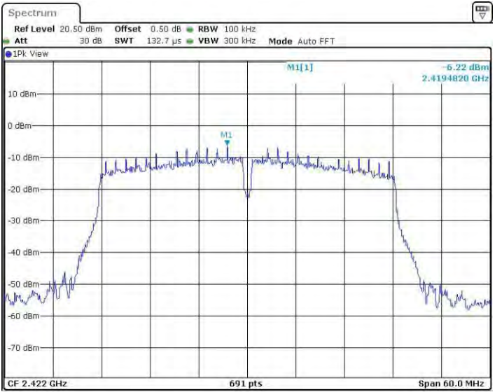
11N40SISO_Ant2_2422_0~Reference
