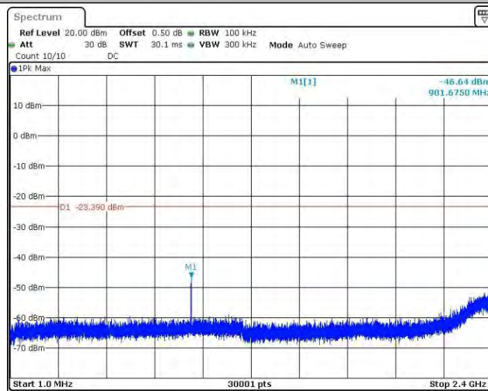
11GMINO_Ant3_2437_0-Reference
