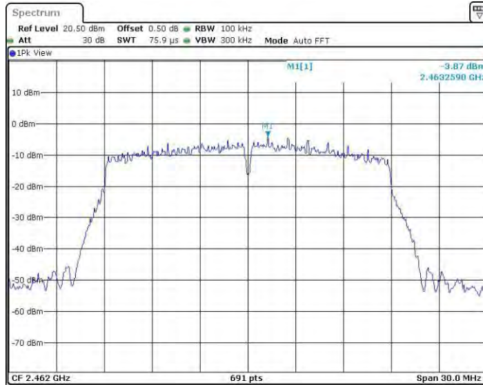
11N20SISO_Ant3_2462_0~Reference
