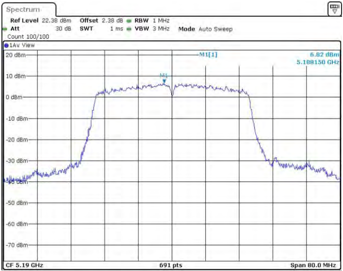
11AC40SISO_Ant4_5190
