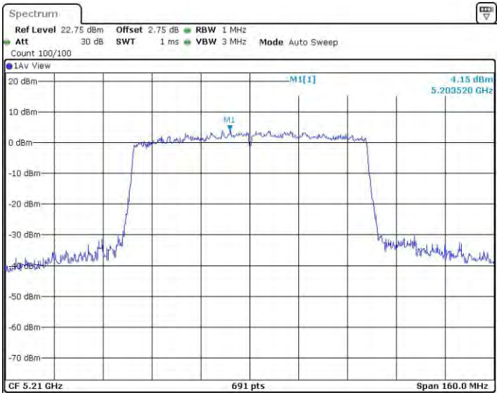
11AC80SISO_Ant3_5210
