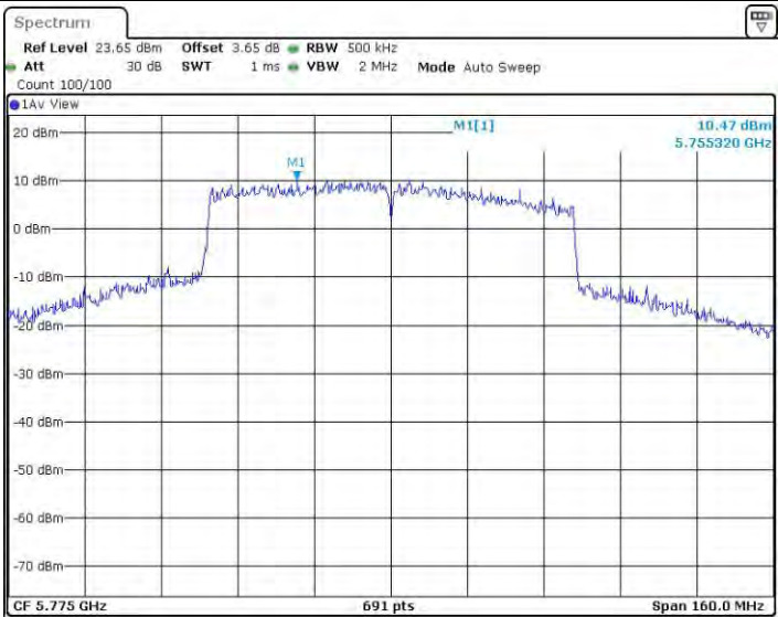
11AC80SISO_Ant3_5775
