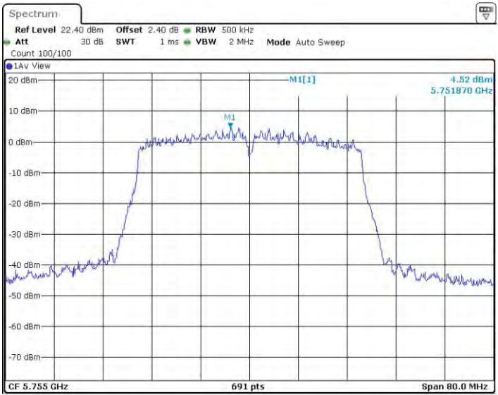
11N40BF_Ant3_5755
