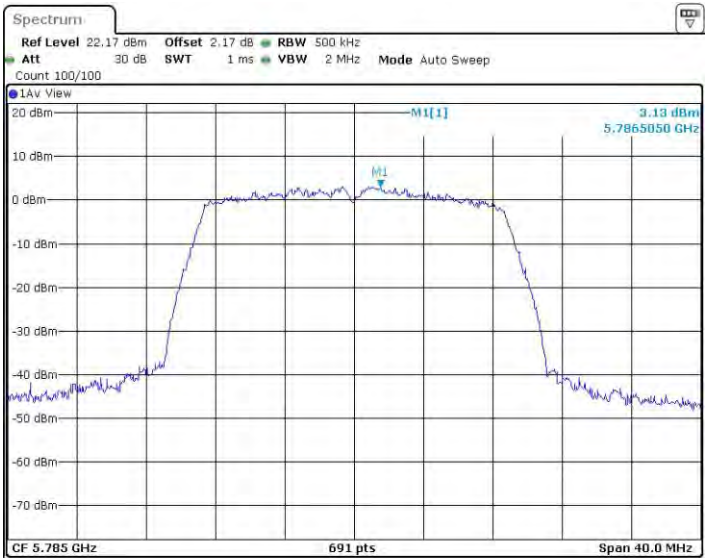
11N20BF_Ant4_5785
