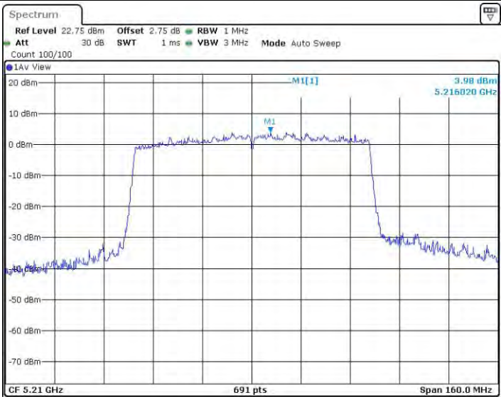
11AC80SISO_Ant4_5210
