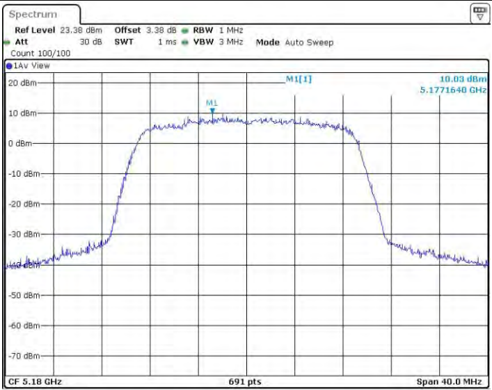
11AC20MIMO_Ant4_5180
