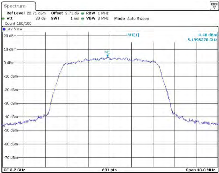
11N20BF_Ant4_5200
