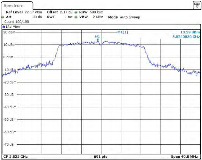
11N20SISO_Ant3_5825
