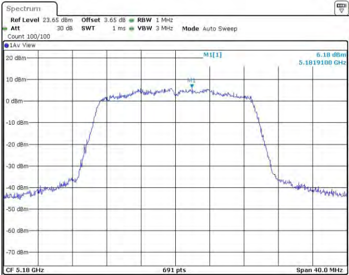
11AC20BF_Ant2_5180
