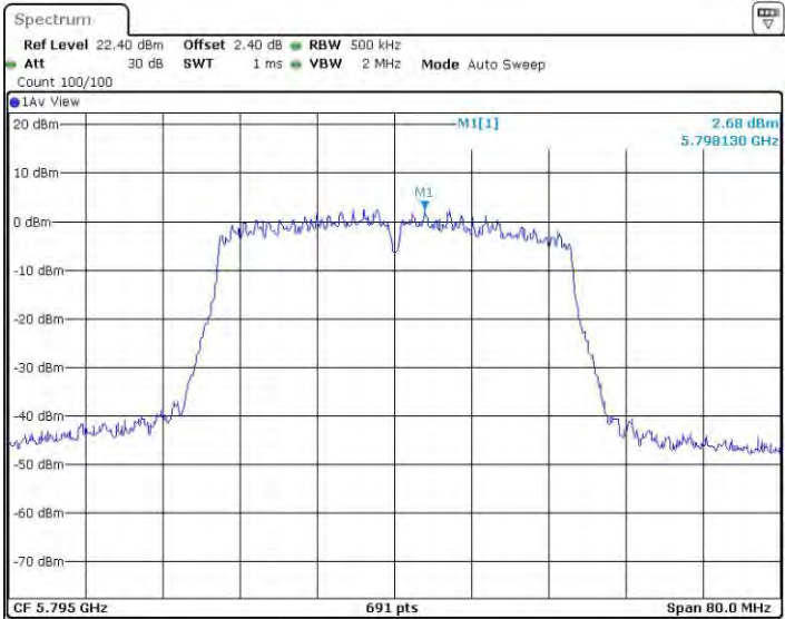
11N40BF_Ant3_5795
