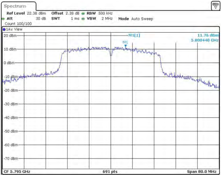
11AC40SISO_Ant3_5795
