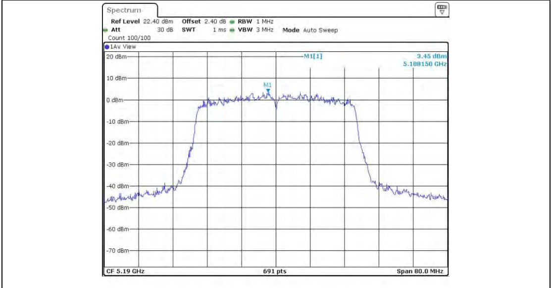
11N40BF_Ant3_5190
