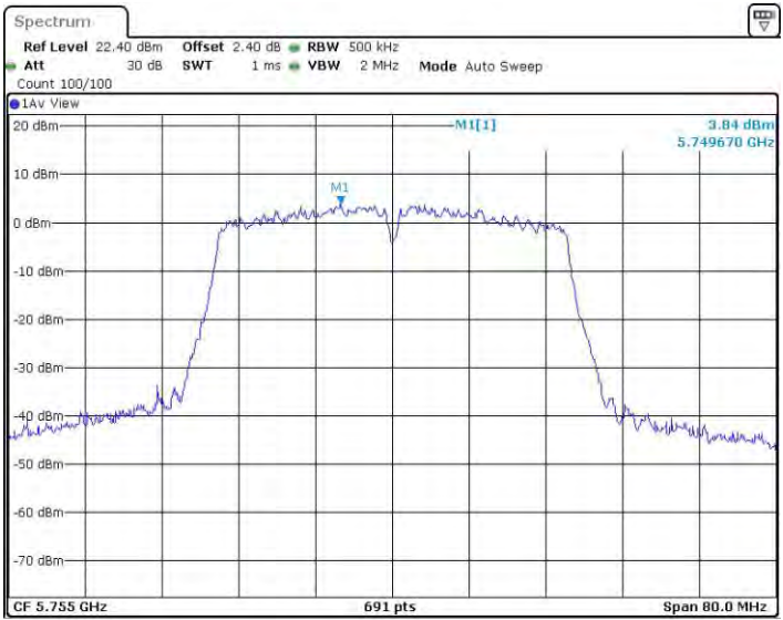
11N40SISO_Ant3_5755
