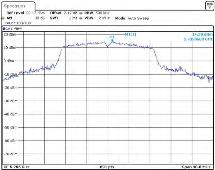
11N20SISO_Ant4_5785
