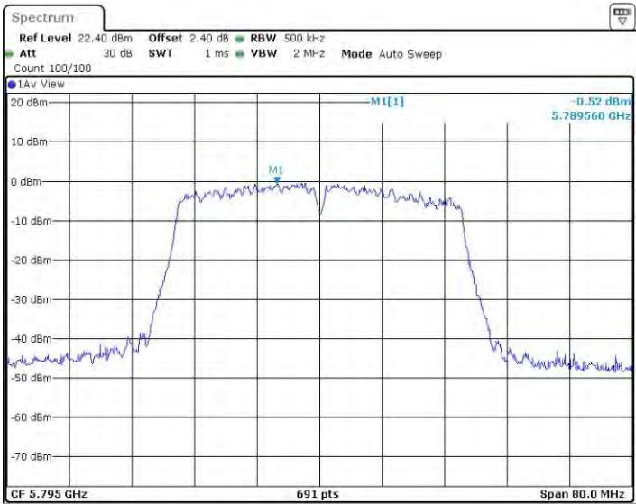
11N40BF_Ant4_5795
