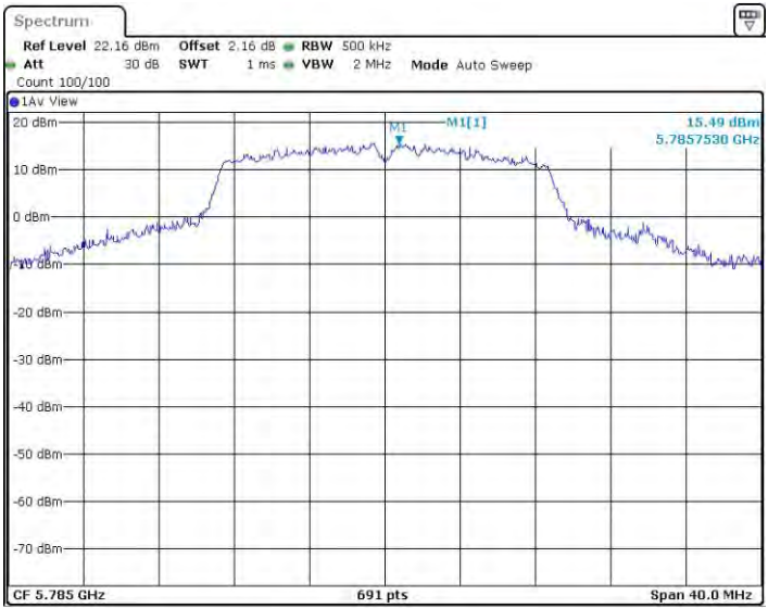
11AC20SISO_Ant3_5785
