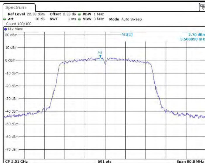
11AC40SISO_Ant4_5510
