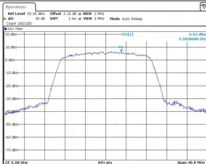
11AC20SISO_Ant4_5580
