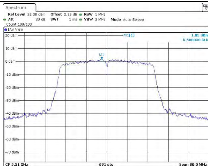
11AC40SISO_Ant3_5510
