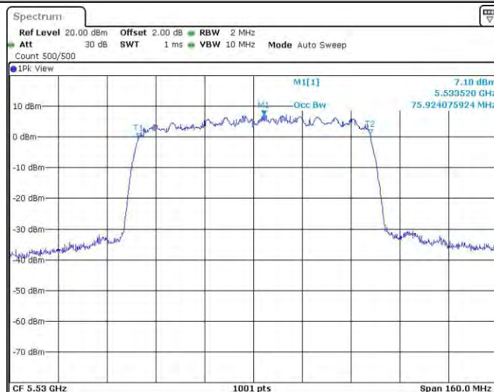
11AC80SISO_Ant3_5530
