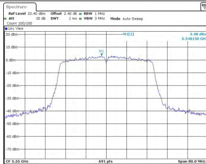
11N40SISO_Ant4_5550
