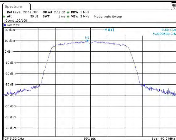
11N20SISO_Ant3_5320
