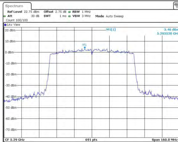
11AC80SISO_Ant3_5290
