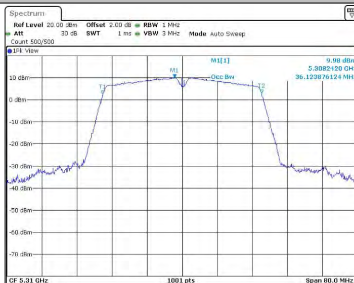
11AC40SISO_Ant3_5310
