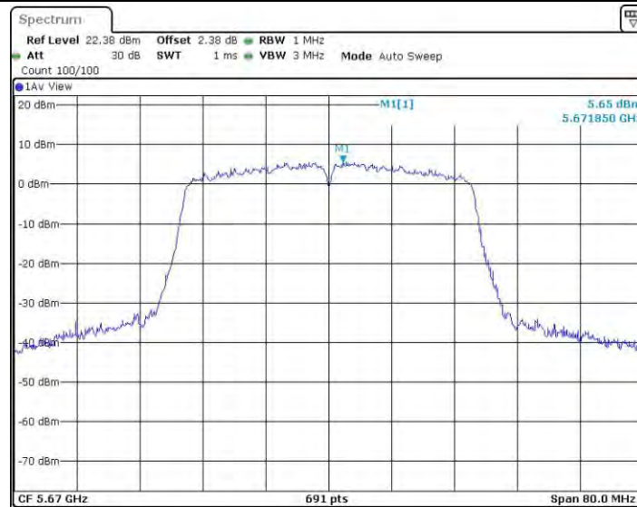
11AC40SISO_Ant4_5670
