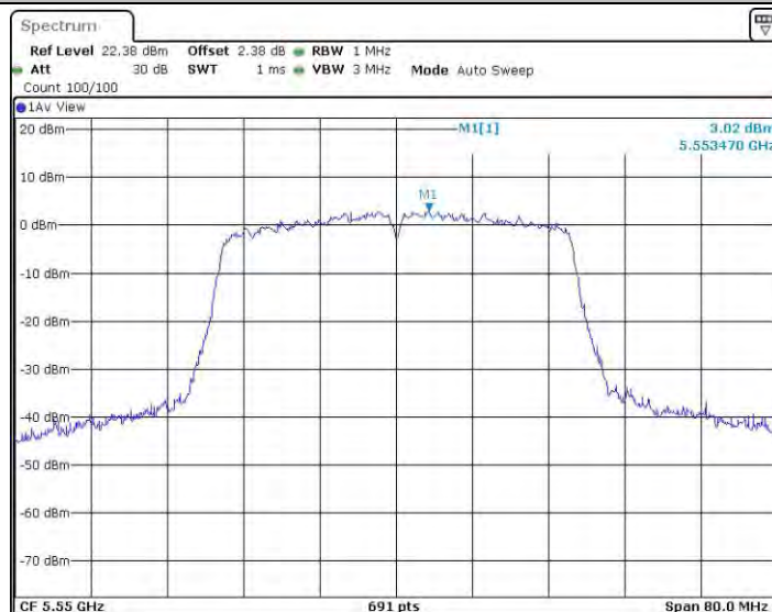
11AC40SISO_Ant3_5550
