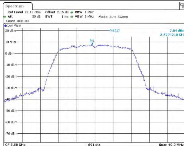
11A_Ant3_5580
