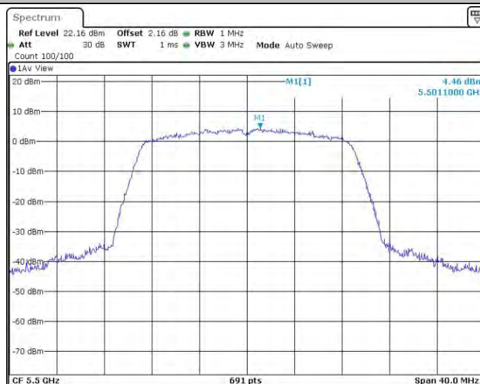
11AC20SISO_Ant3_5500
