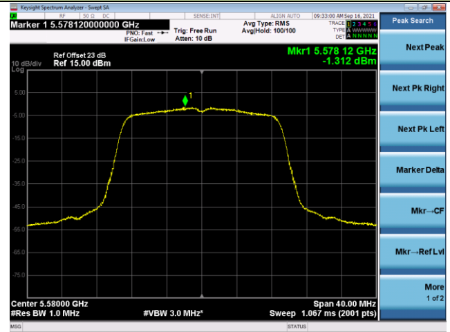
Channel 116 (5580MHz)
