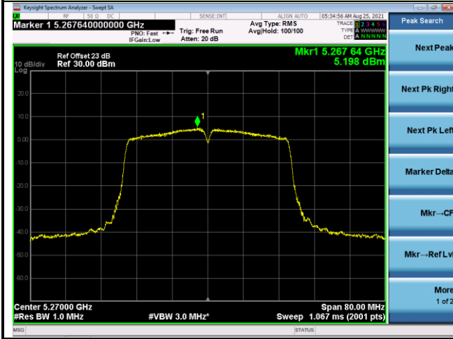
Channel 54 (5270MHz)
