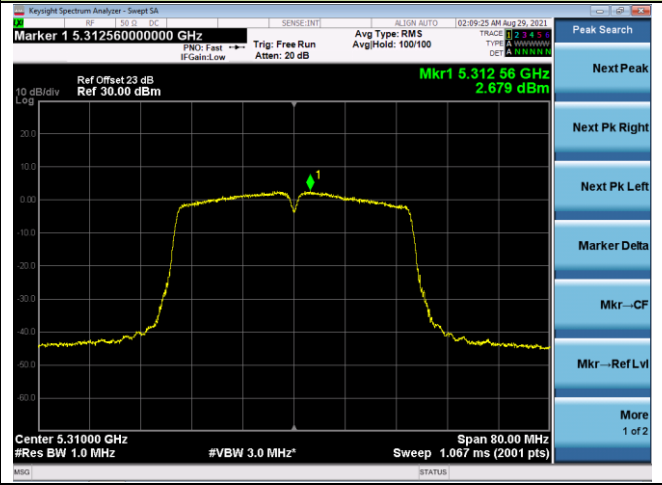
Channel 62 (5310MHz)
