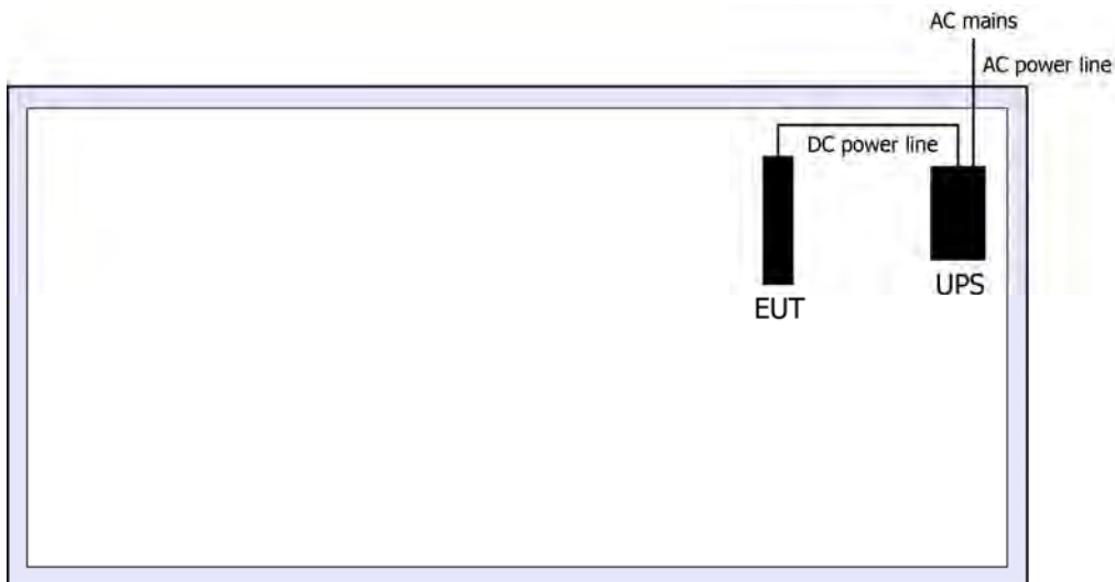
Test Setup Diagram – AC Line Conducted Emission Test (Mode 2)
