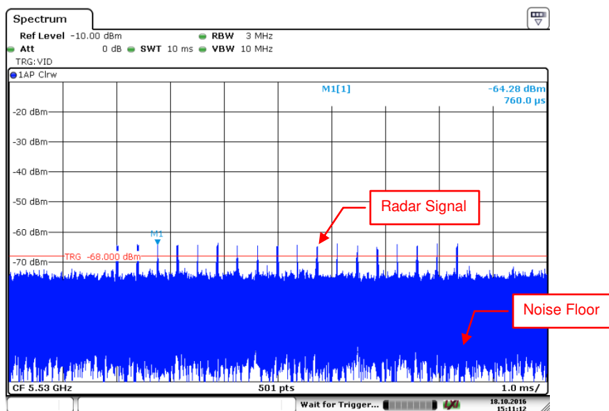
Radar Signal 2
