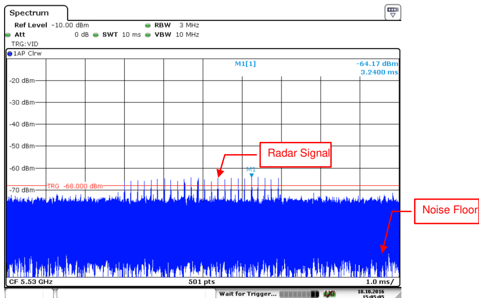
Radar Signal 2
