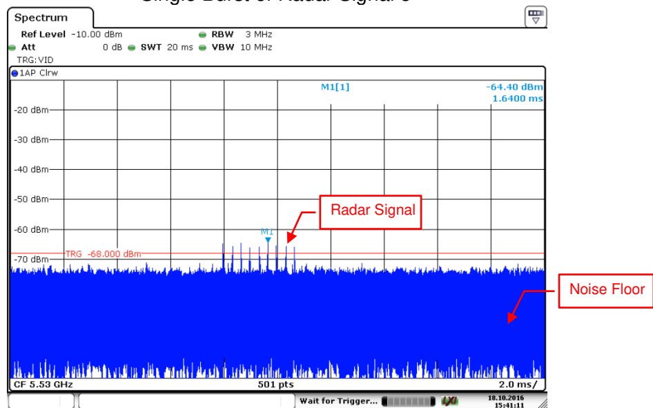
Radar Signal 6
