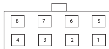
Figure 4. 8-Pin Molex Connector
