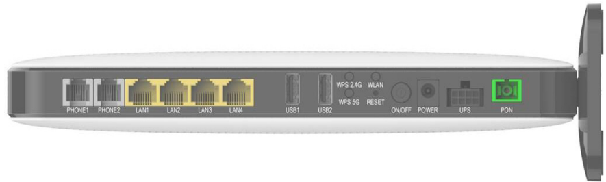
FIGURE 1-1. Rear View
