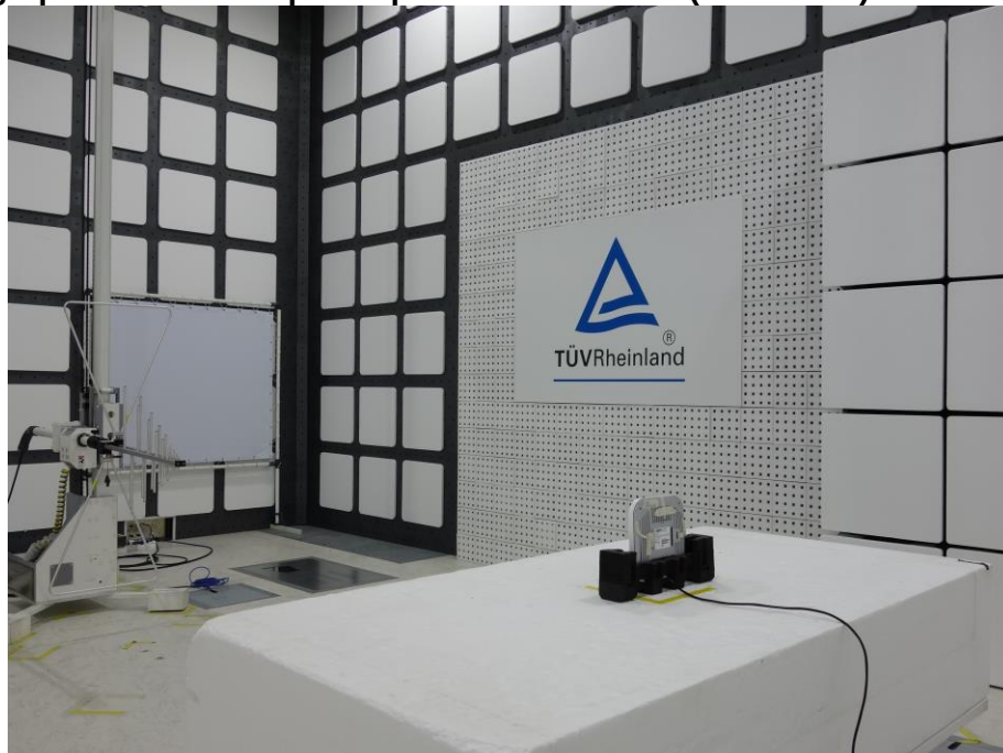
Photograph 16: Test Setup for Spurious Emissions (Back View)
