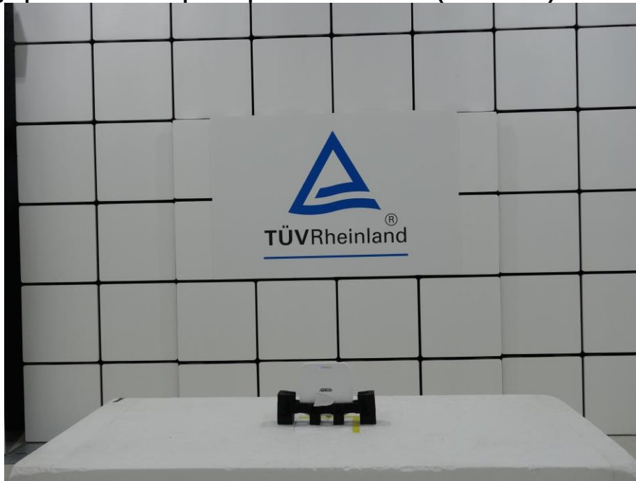
Photograph 17: Test Setup for Spurious Emissions (Front View)
