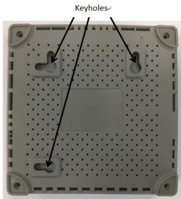
Figure 4. Wall Mount Keyholes
