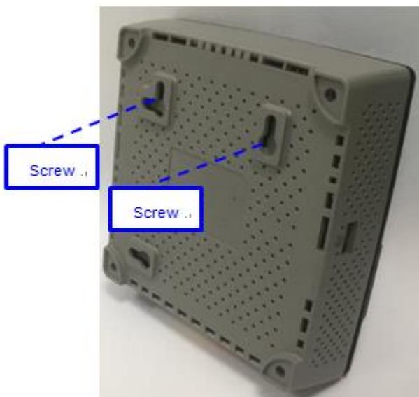
Figure 5. Place Ø3.5*30L Screws
