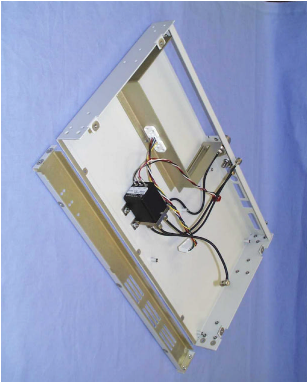
Photograph 2.8 Tracer Monitored Protection Switch Inside Chassis – Boards Removed
