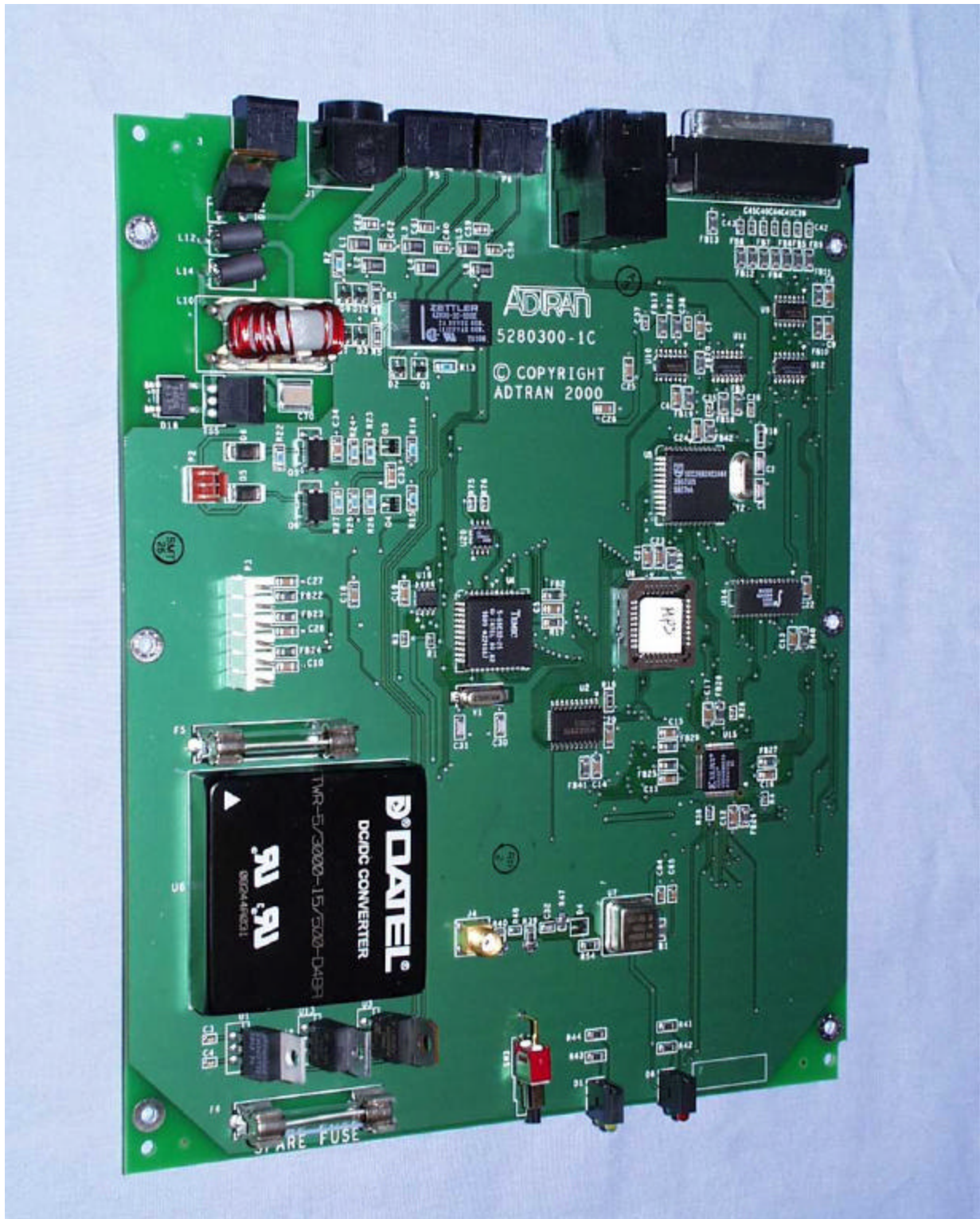
Photograph 2.6 Tracer Monitored Protection Switch Main PCB – Component Side
