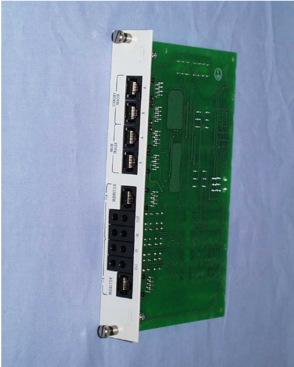
Photograph 2.4 Tracer Monitored Protection Switch T1 Interface Card – Solder Side
