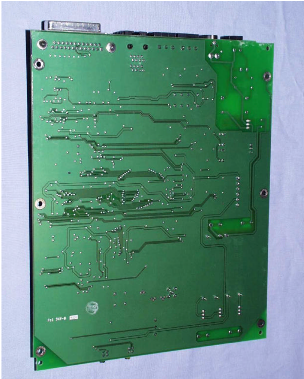
Photograph 2.7 Tracer Monitored Protection Switch Main PCB – Solder Side
