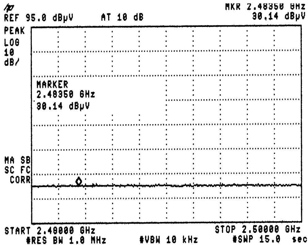
Figure 3.5 - 6: Comsat RSI Grid Parabolic (M/N: P-24A36GN-U) 24.8 dBi – Restricted Band, Horizontal
