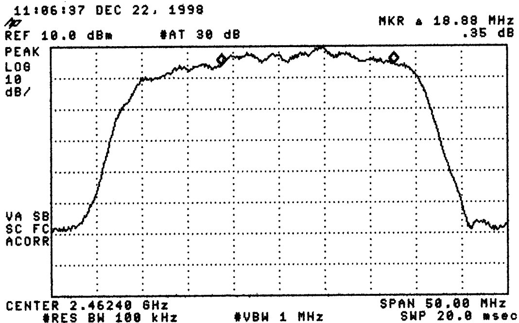
Figure 3.1 - 1: Emission Bandwidth Plot
