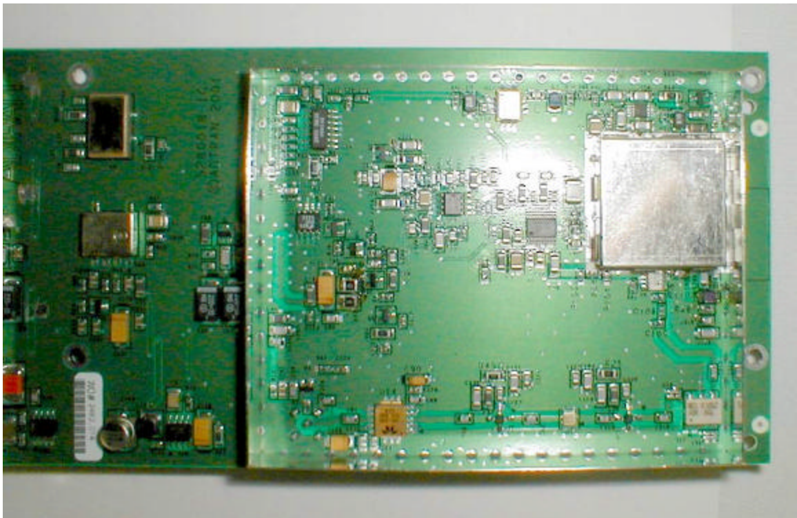
RF Converter Detail B
