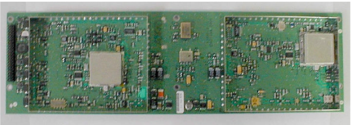
RF Converter Shields Removed
