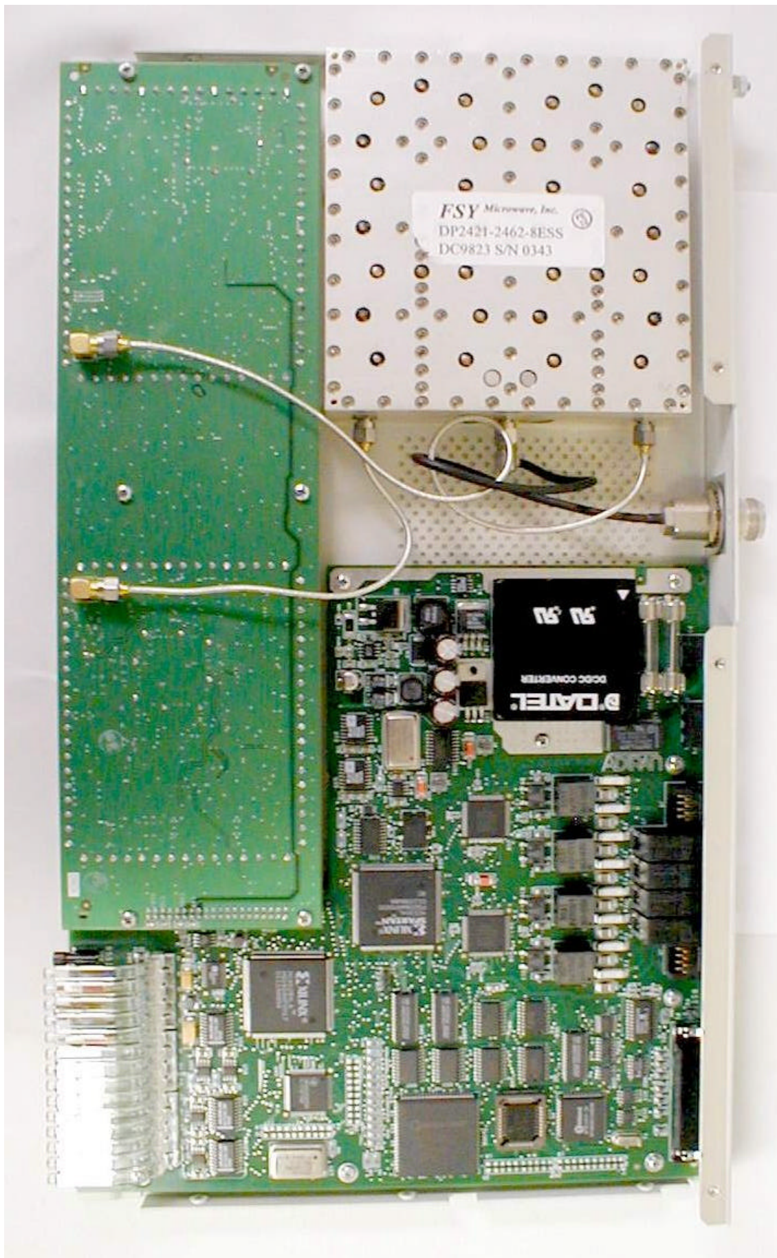
Top Cover Removed
