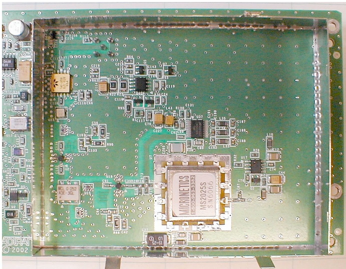
RFC Board Bottom Right Detail
