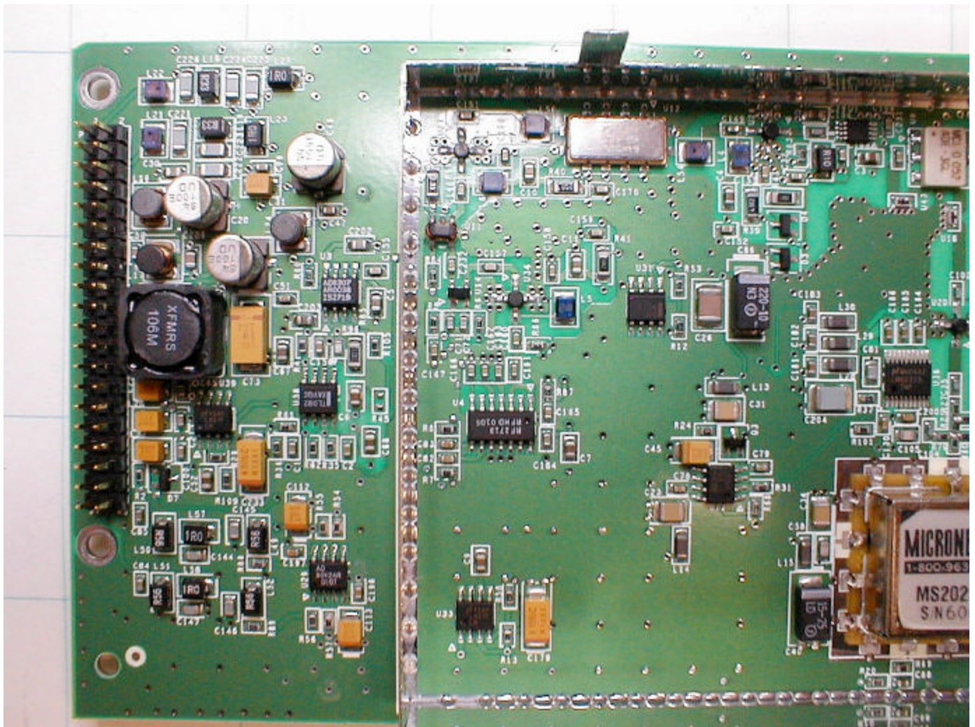
RFC Board Bottom Left Detail
