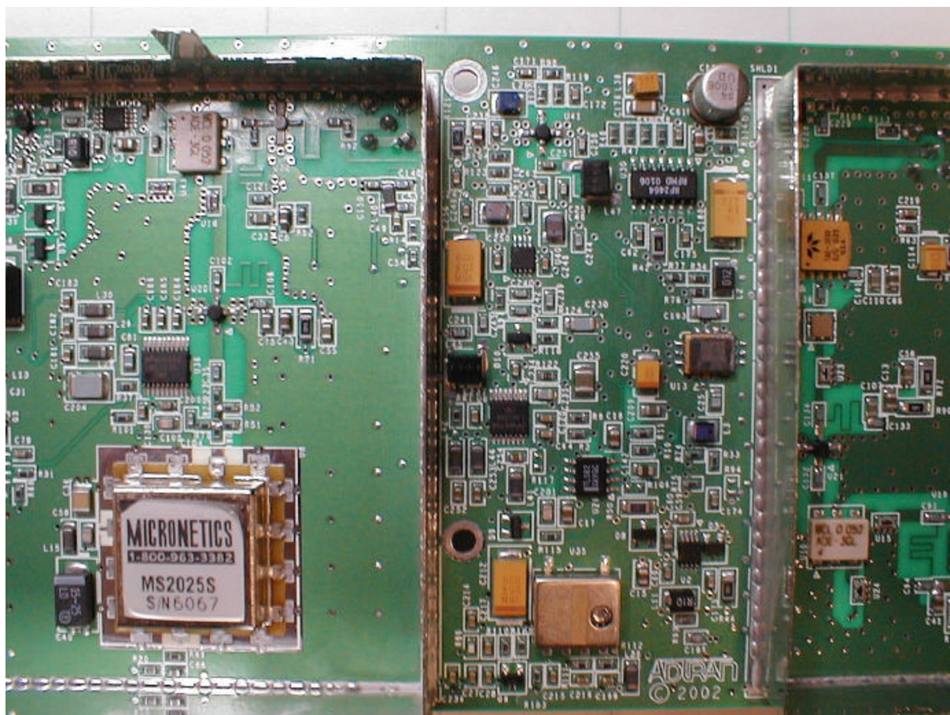
RFC Board Bottom Center Detail
