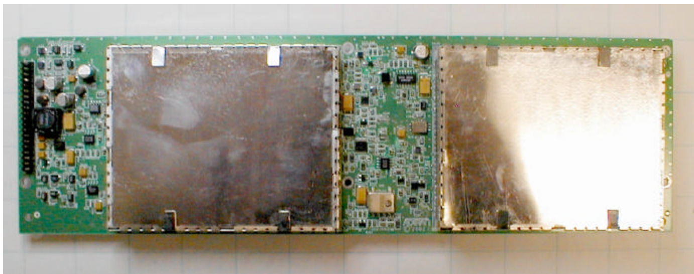
RFC Board Bottom Overview
