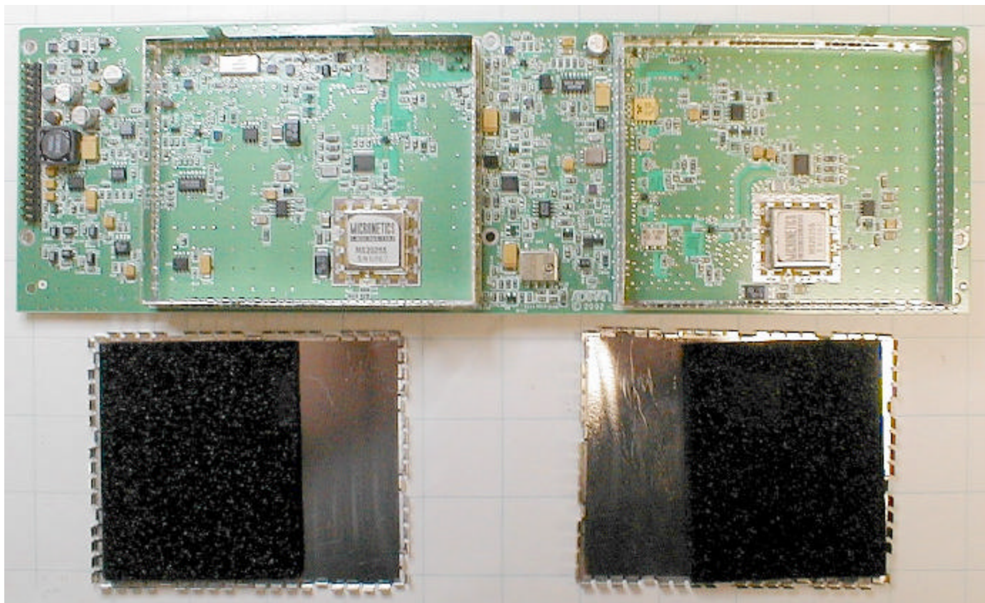
RFC Board Bottom, Covers Removed
