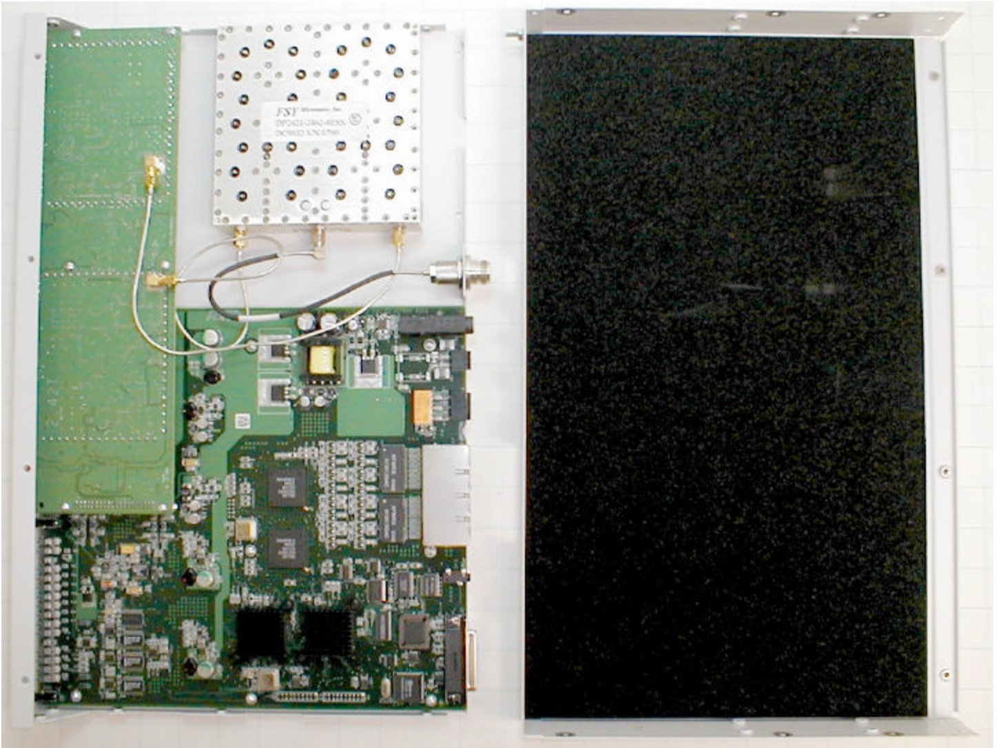
Top Cover Removed
