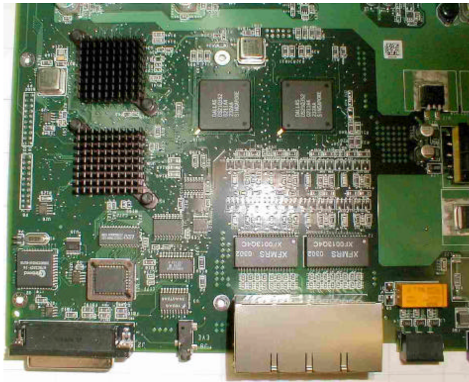
Baseband Board Top, Quadrant 4
