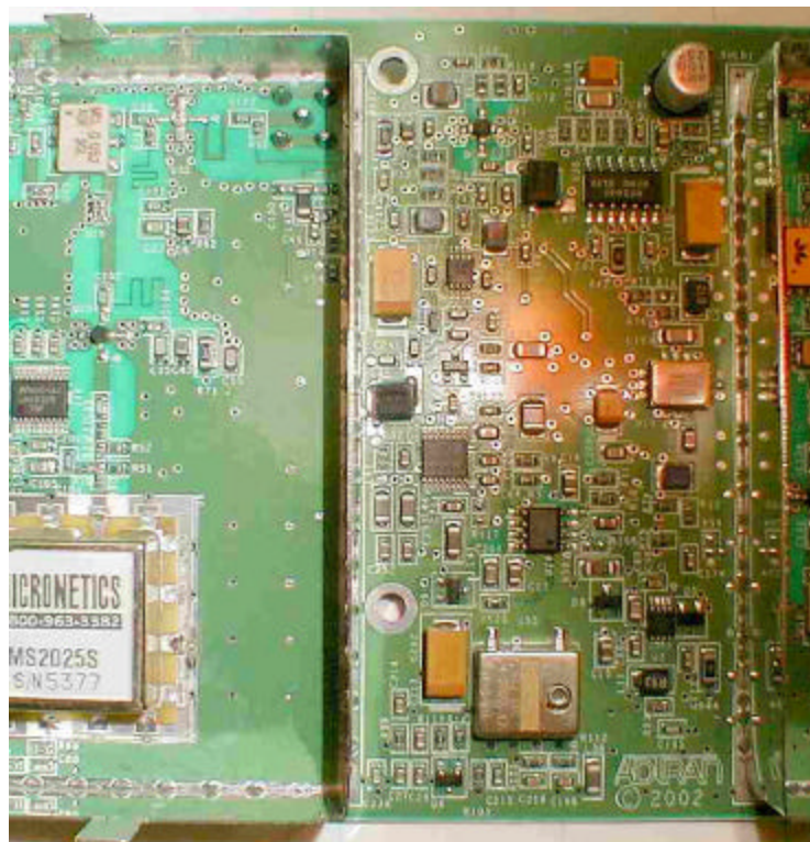
RFC Board Bottom Mid
