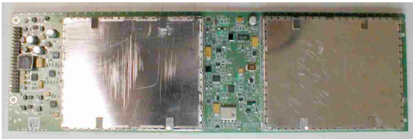
RFC Board Bottom, Shields In Place
