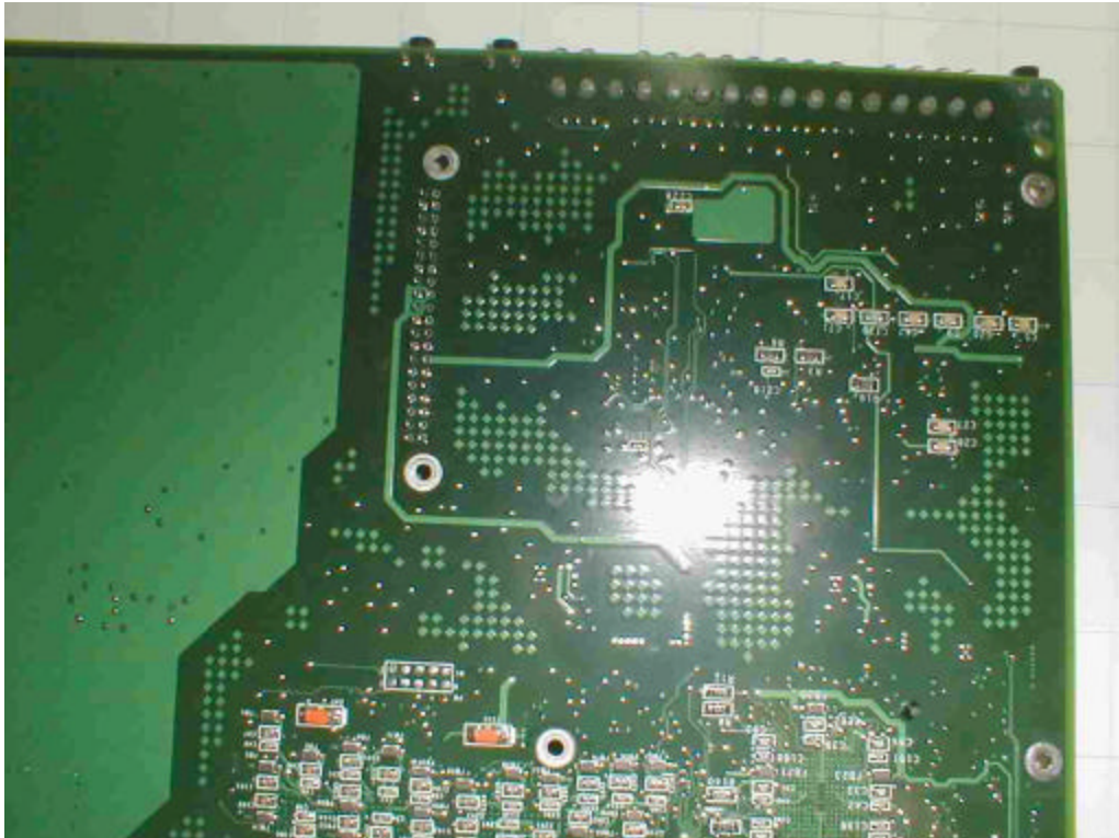
Baseband Board Bottom, Quadrant 1
