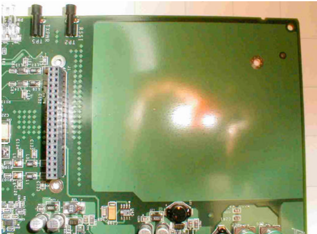
Baseband Board Top, Quadrant 2
