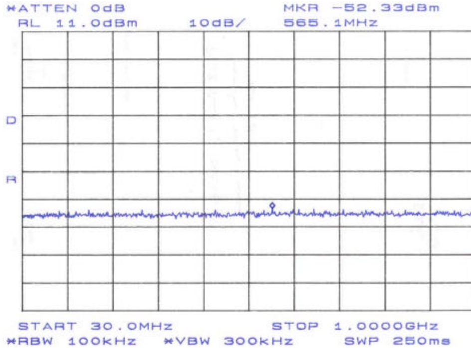
Figure 24. Conducted Spurious: Plan B Band 1 30MHz – 1GHz
