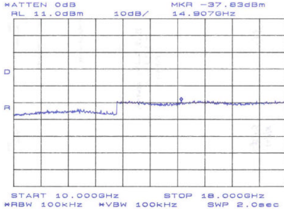
Figure 32. Conducted Spurious: Plan B Band 3 10GHz – 18GHz
