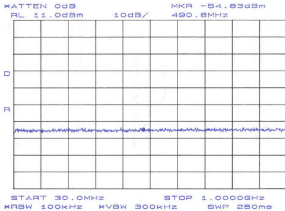
Figure 19. Conducted Spurious: Plan A Band 3 30MHz – 1GHz
