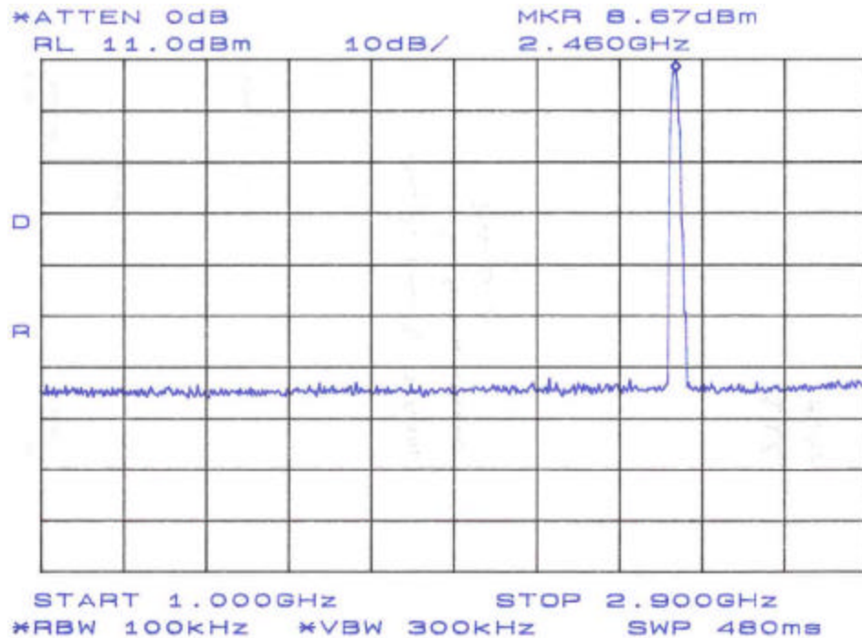
Figure 25. Conducted Spurious: Plan B Band 1 1GHz – 2.9GHz
