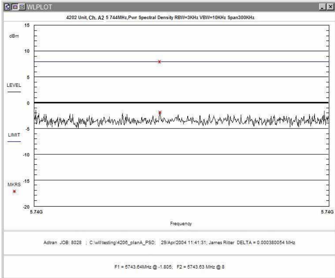
Figure 3. Power Spectral Density Plan A, Band 2
