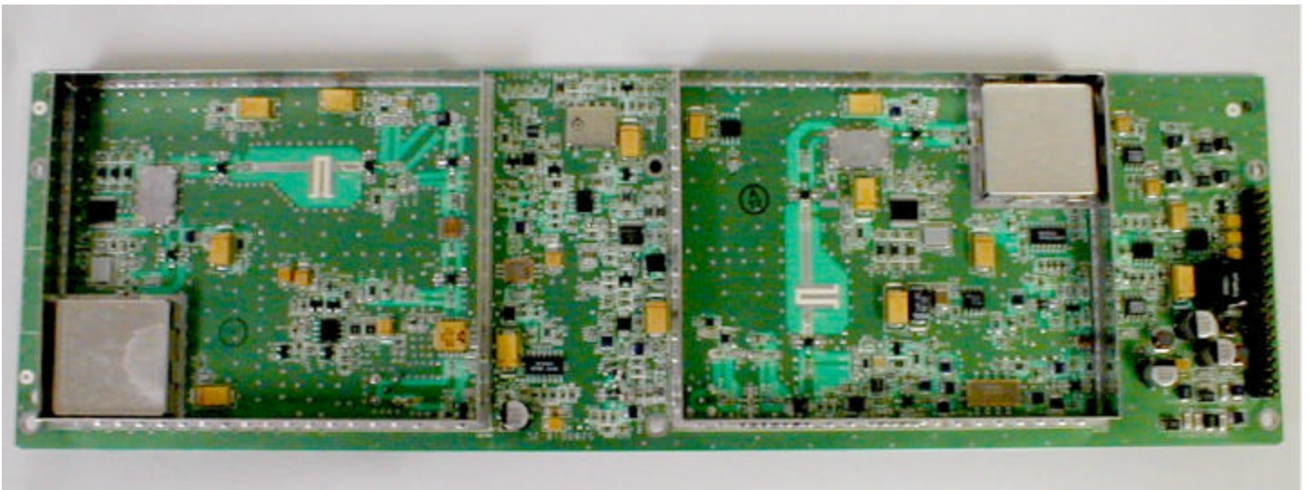
RF Converter Shields Removed
