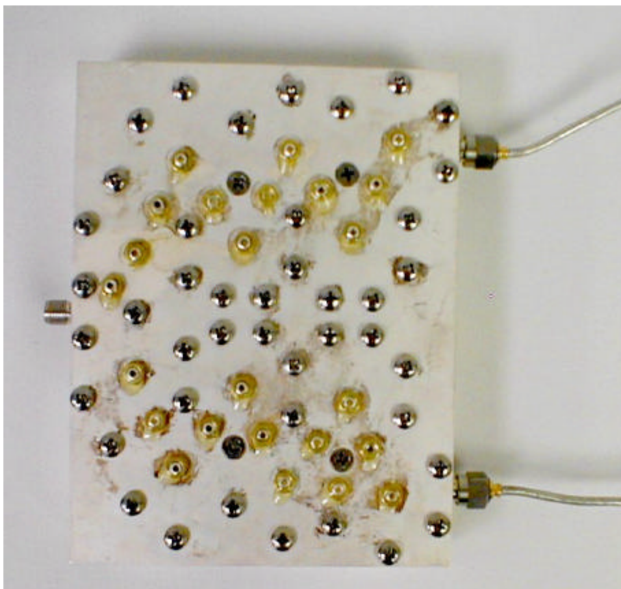
Power Amplifier Module Bottom View
