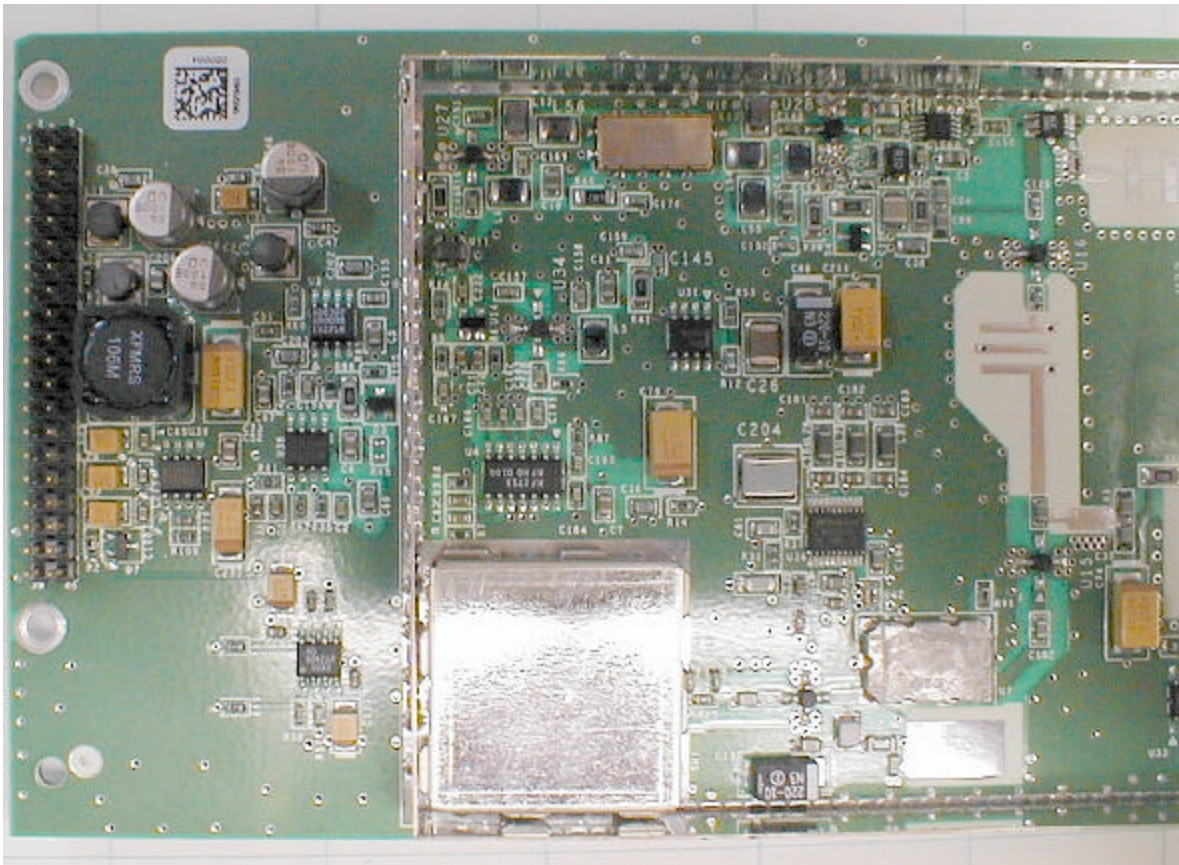
RFC Board Bottom Left Side, Large Shield Removed
