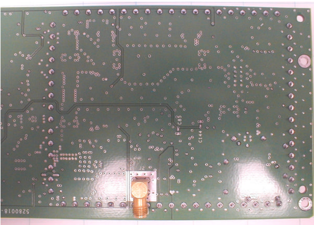
RFC Board Top Right
