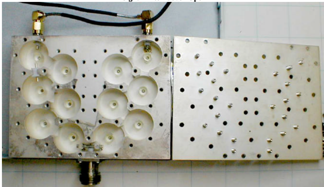
Signal Filter Cover Open
