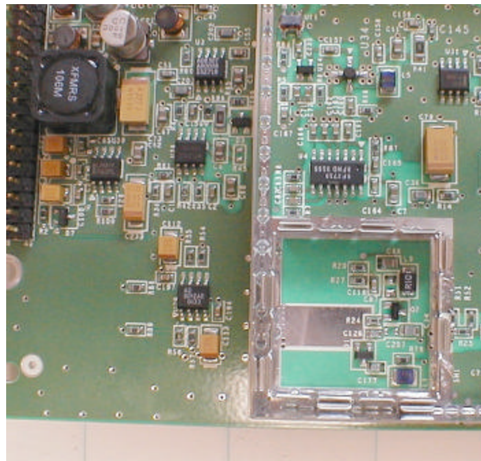
RFC Board Bottom Left Detail, Small Shield Removed
