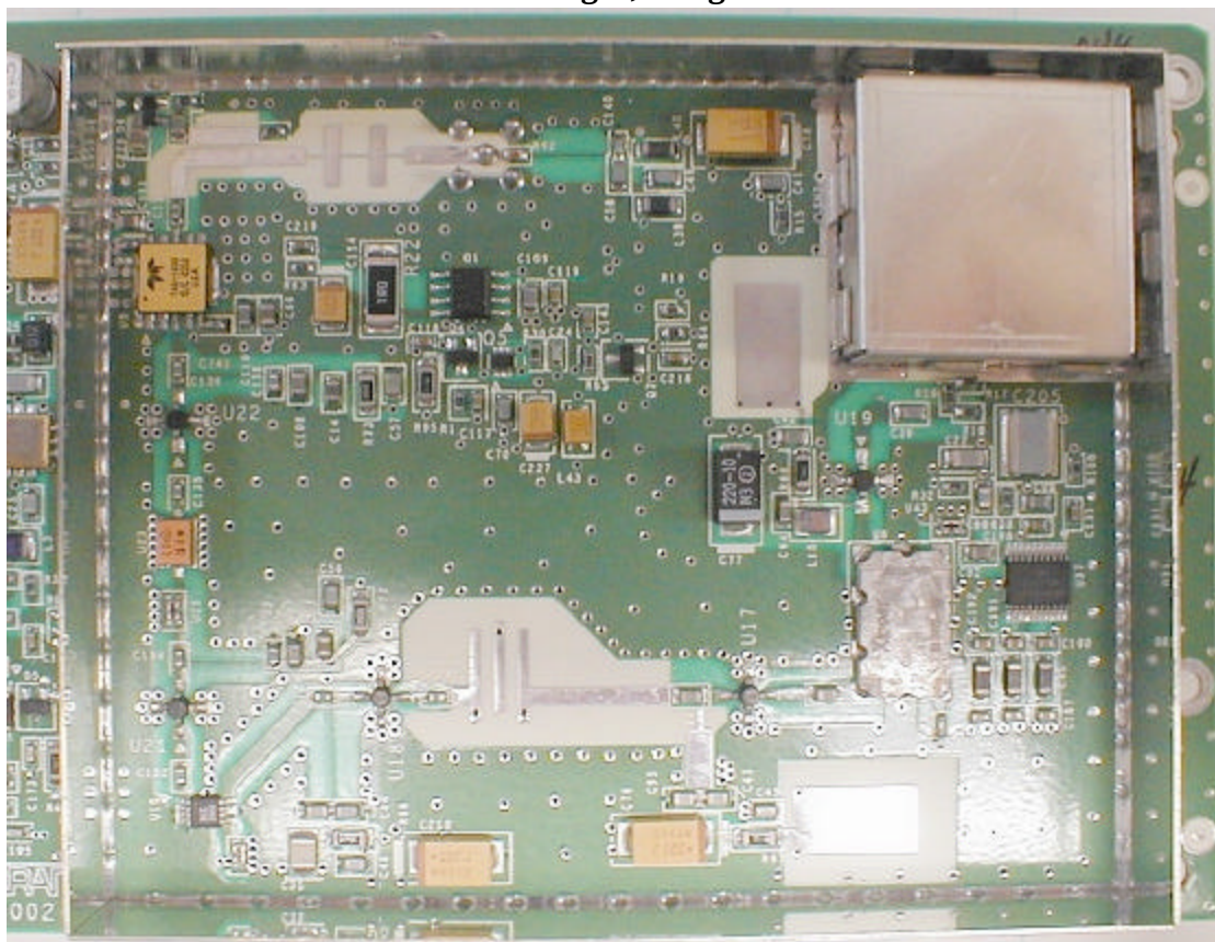
RFC Board Bottom Right, Large Shield Removed
