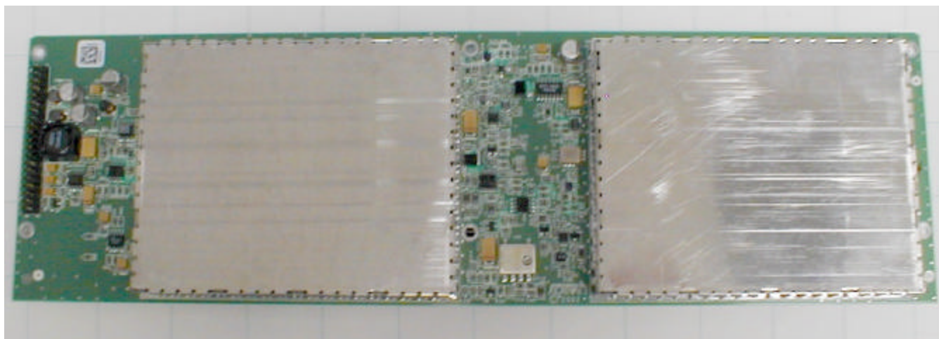
RFC Board Bottom Overview
