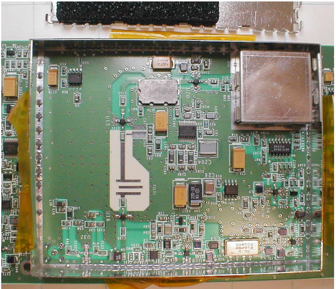
RFC Board Bottom Right Small Cover Removed Detail
