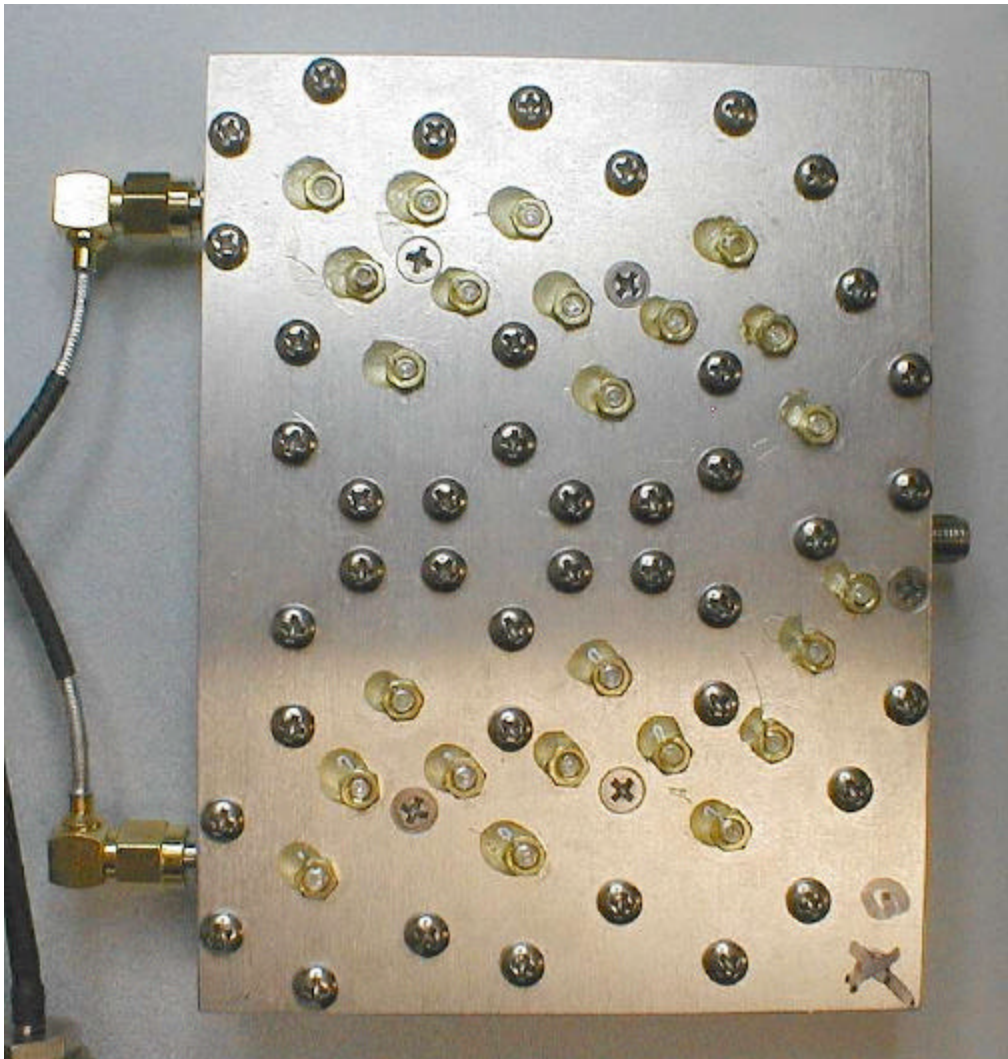
Signal Filter Connector Detail
