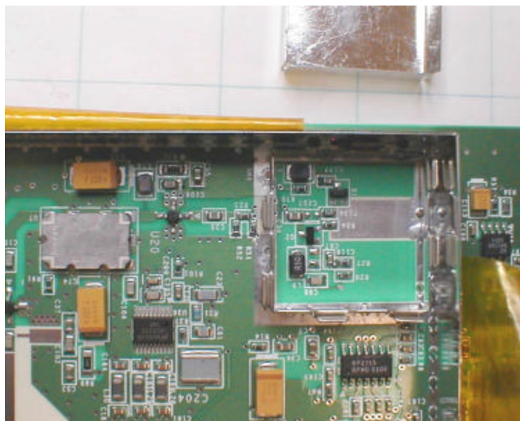
RFC Board Bottom Right Small Cover Removed Detail
