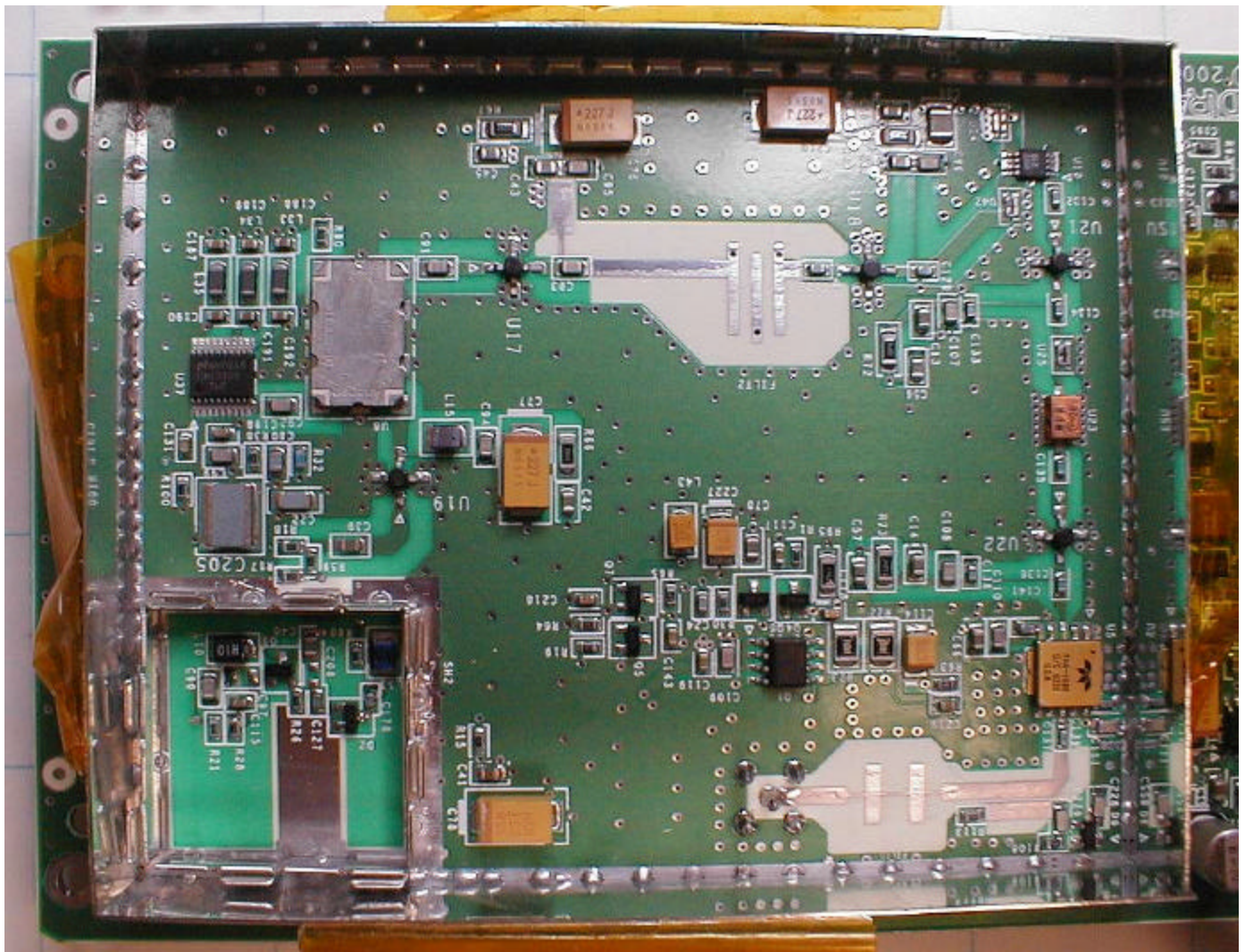
RFC Board Bottom Left, Main and Small Cover Removed
