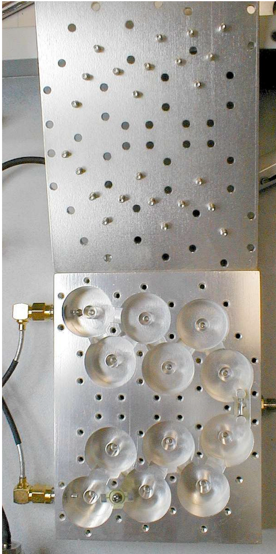
Signal Filter Cover Removed
