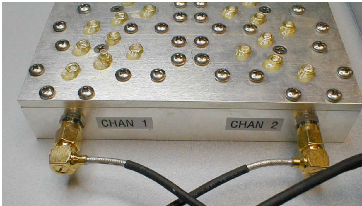
Signal Filter Connector Detail
