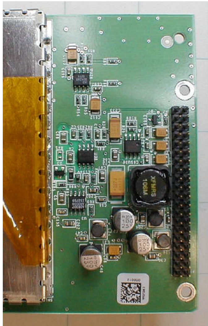
RFC Board Bottom, Far Right Side
