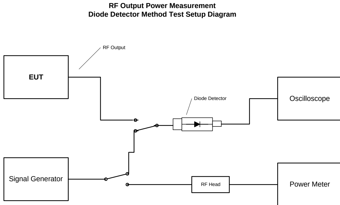
Figure 1: RF Power Measurement Test Setup Diagram
