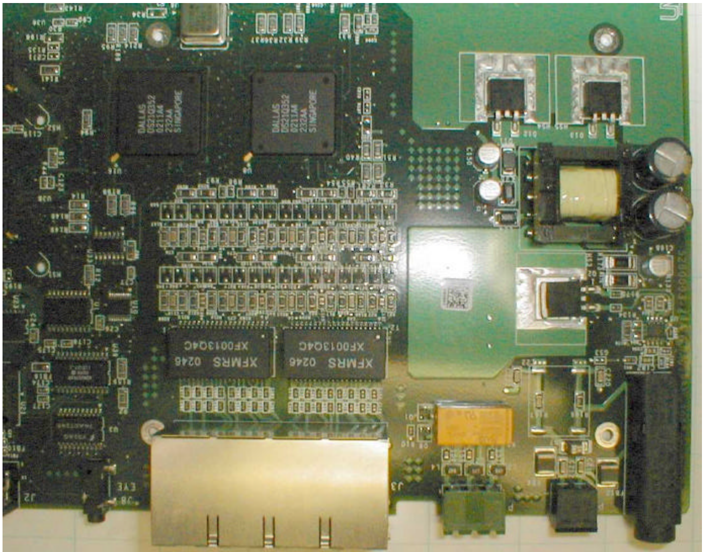
Baseband Board Top, Detail C
