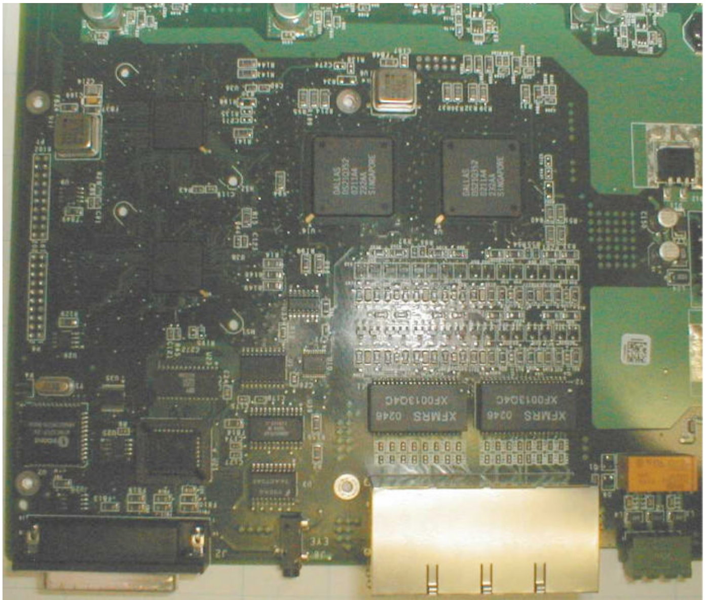
Baseband Board Top, Detail D
