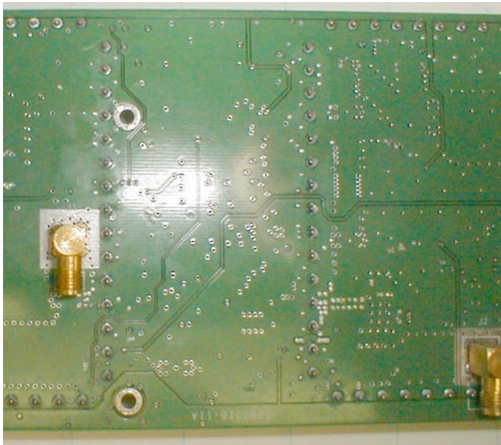
RFC Board Top Center
