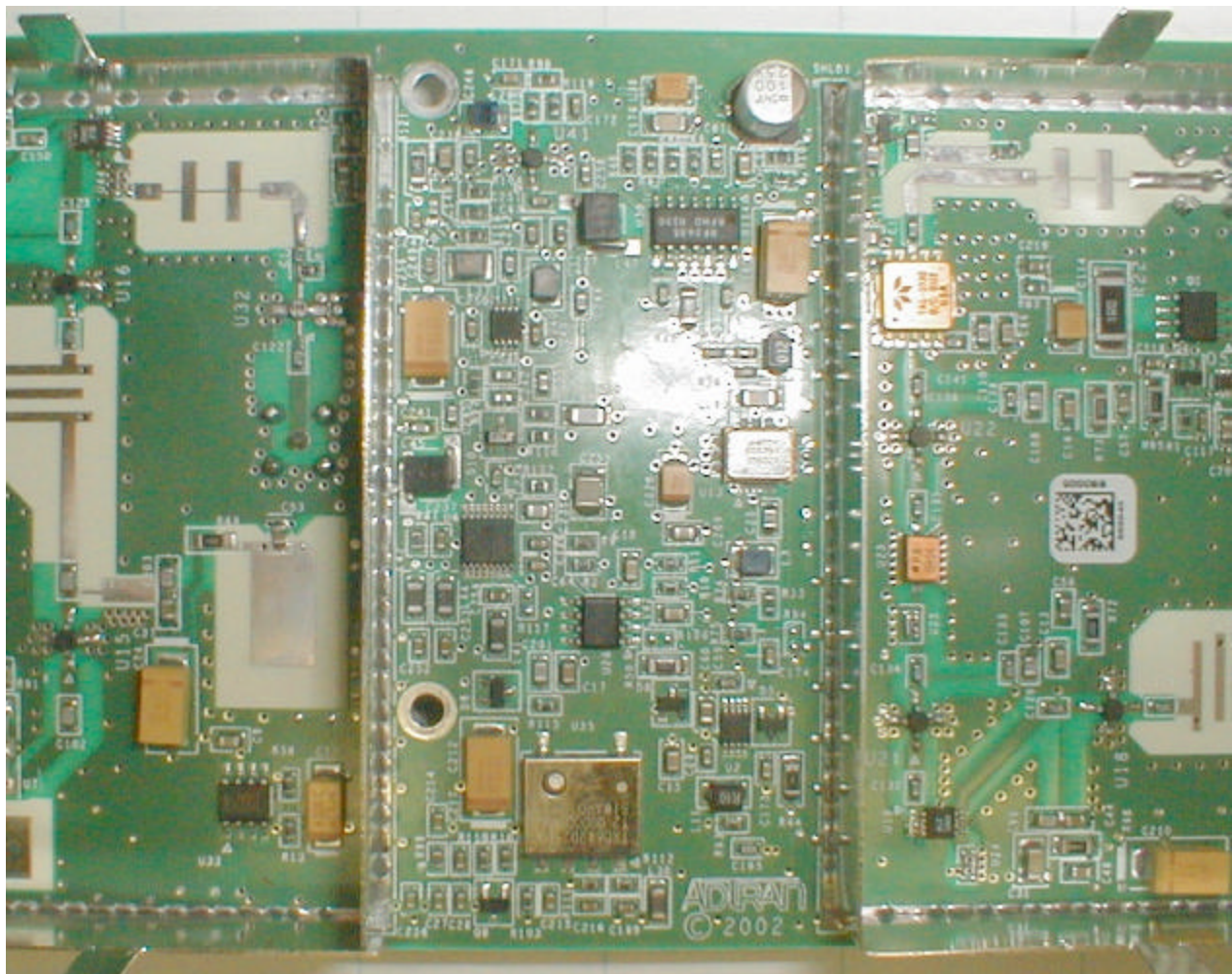
RFC Board Bottom Center Detail
