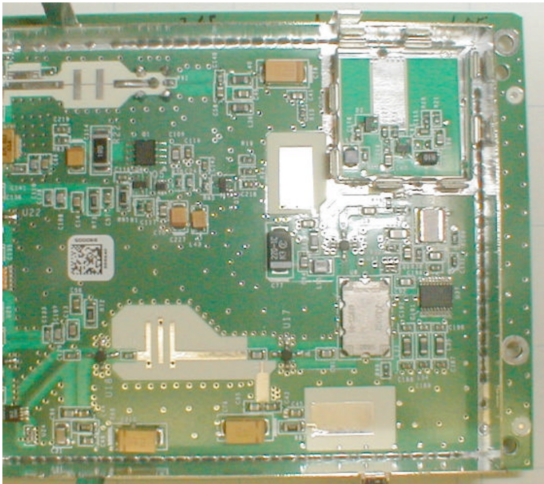
RF Board Bottom Right Detail
