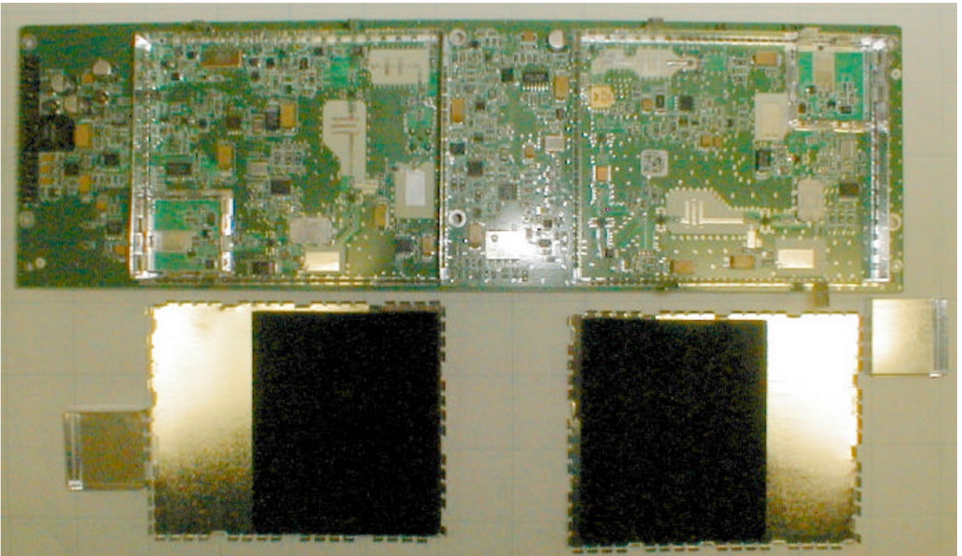
RFC Board Bottom Overview Shields Removed
