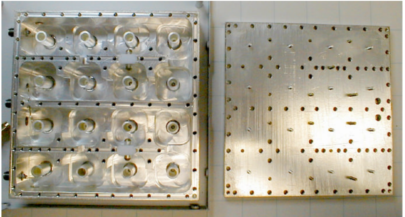
Typical Interior View of Signal Filter
