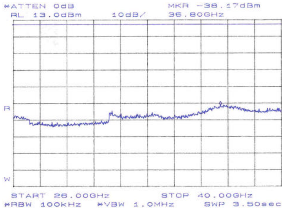
Figure 30. Conducted Spurious Emissions, Plan B Band 1, 26GHz-40GHz
