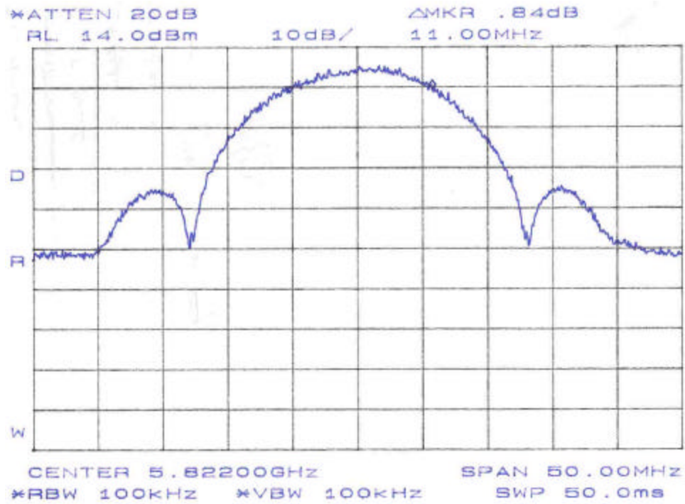
Figure 8. Occupied Bandwidth - Plan B, Band 1
