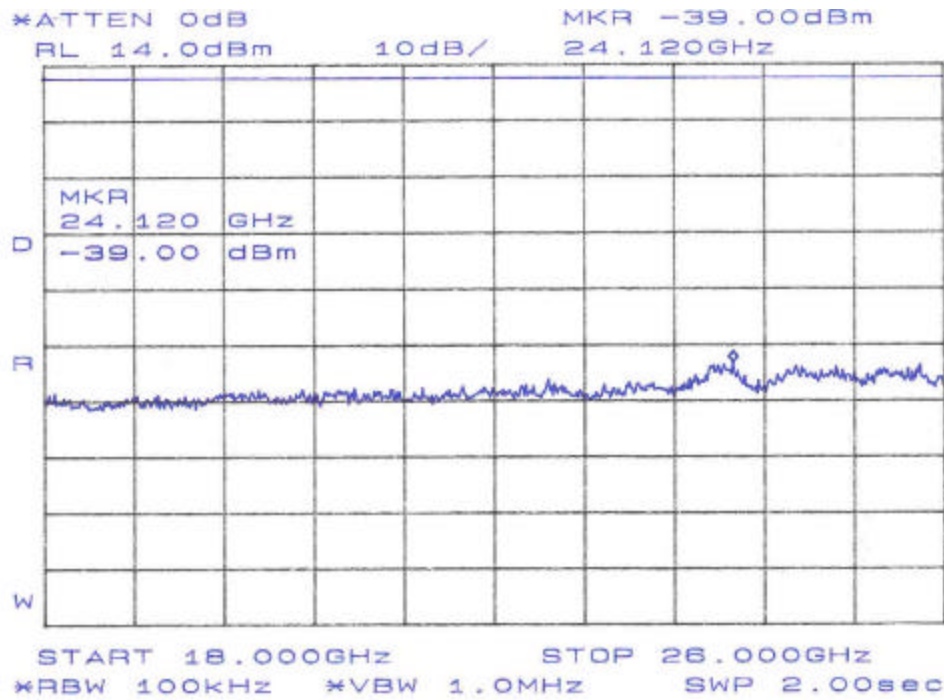
Figure 17. Conducted Spurious Emissions, Plan A Band 1, 18GHz-26GHz
