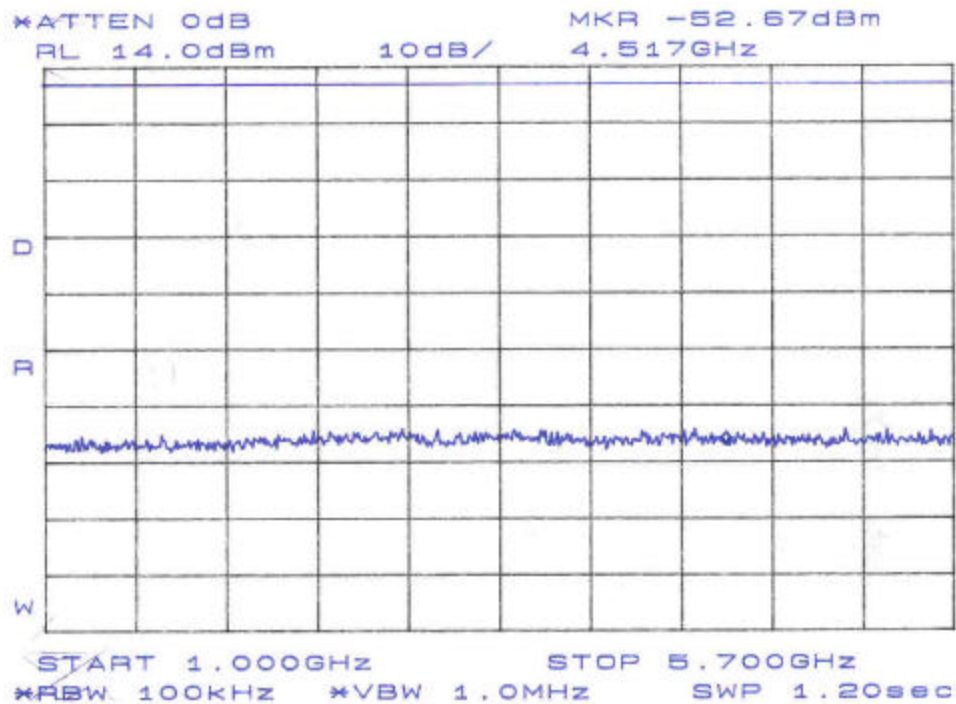
Figure 20. Conducted Spurious Emissions, Plan A Band 3, 1GHz-5.7GHz
