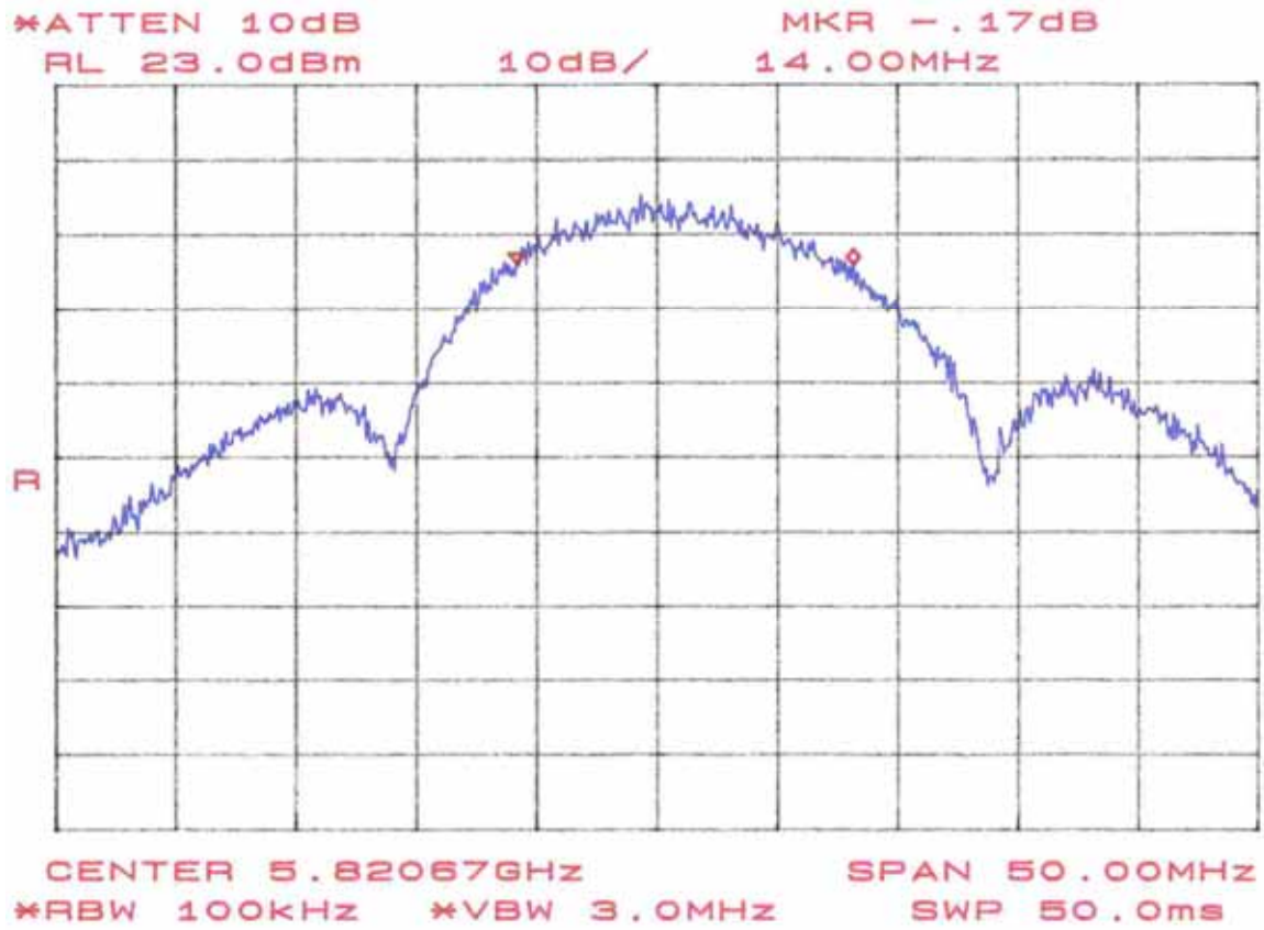
Figure 10. Occupied Bandwidth - Plan B, Band 1
