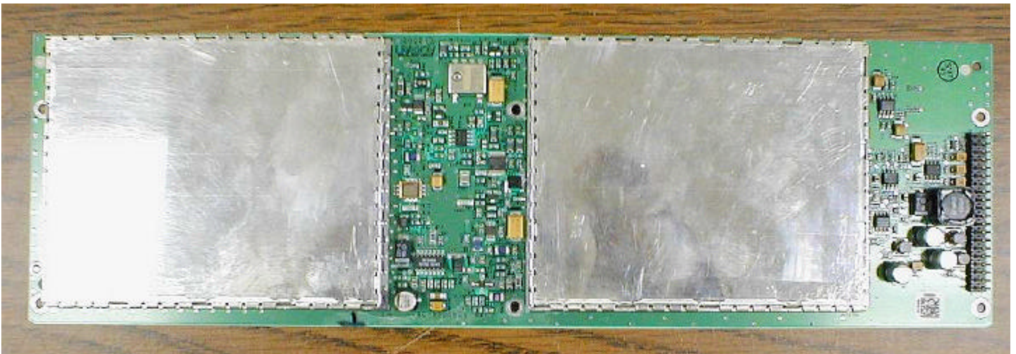
RFC Board, Bottom
