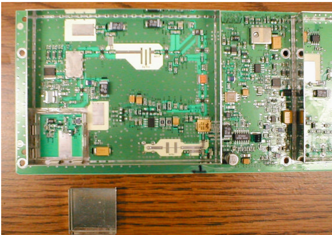
RFC Board, Left Side Detail, Small Shield Removed
