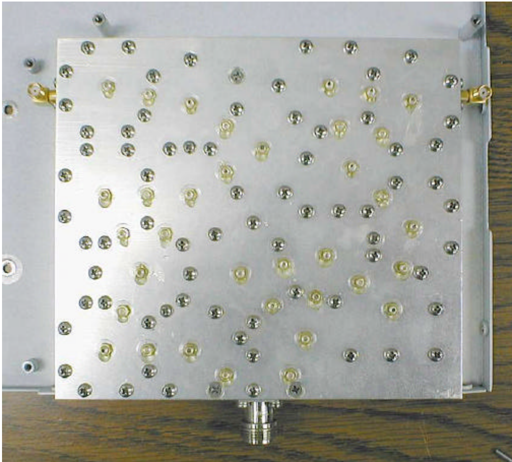
Signal Filter, Top View
