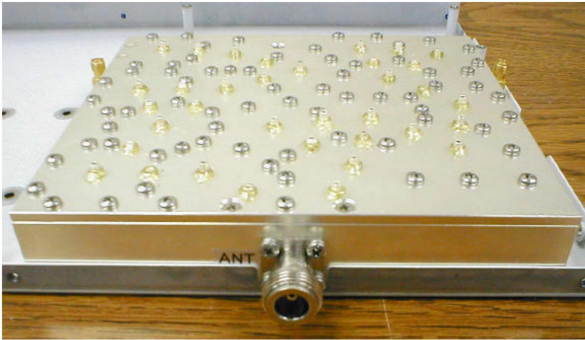
Signal Filter, Internal View
