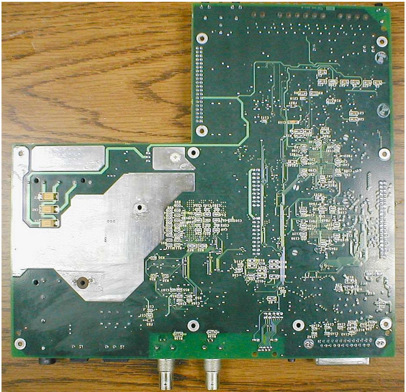
Baseband PCB Bottom
