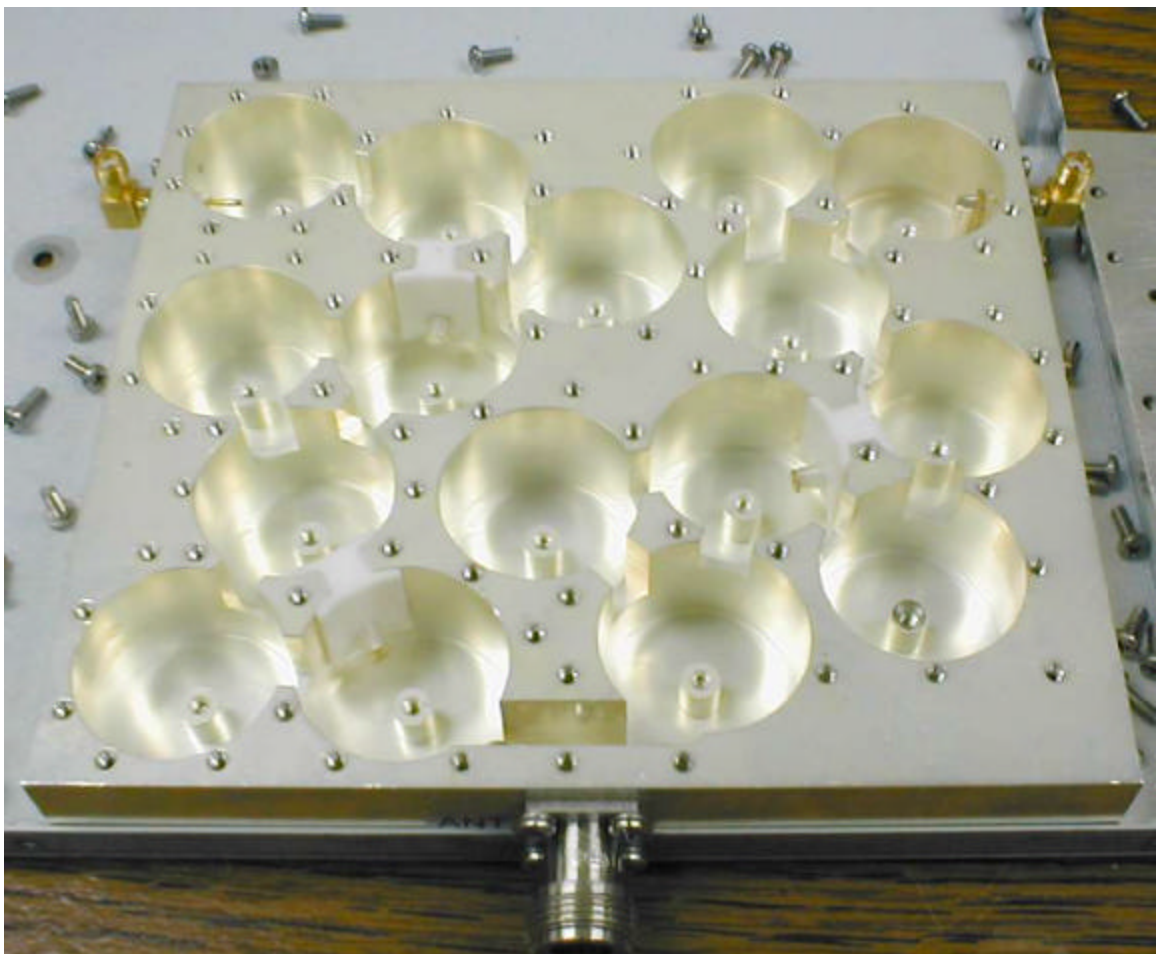
Signal Filter, Internal View
