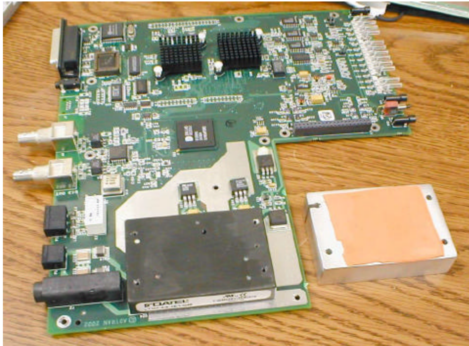
Datel Module, Cover Removed
