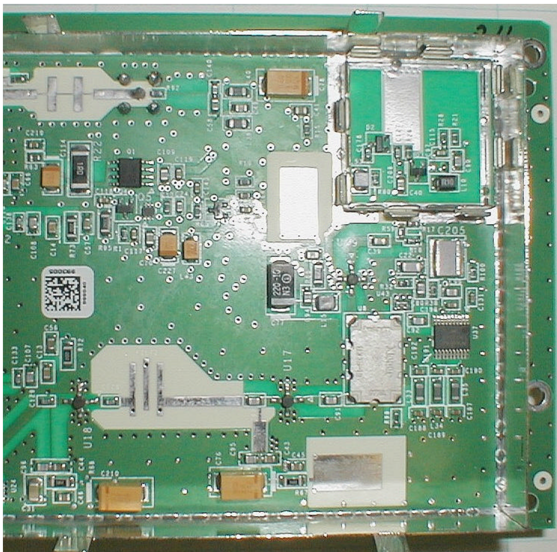
RFC Board Bottom Right Detail
