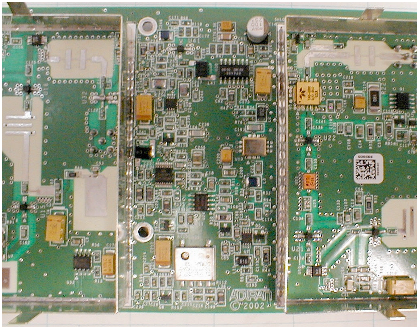
RFC Board Bottom Center Detail
