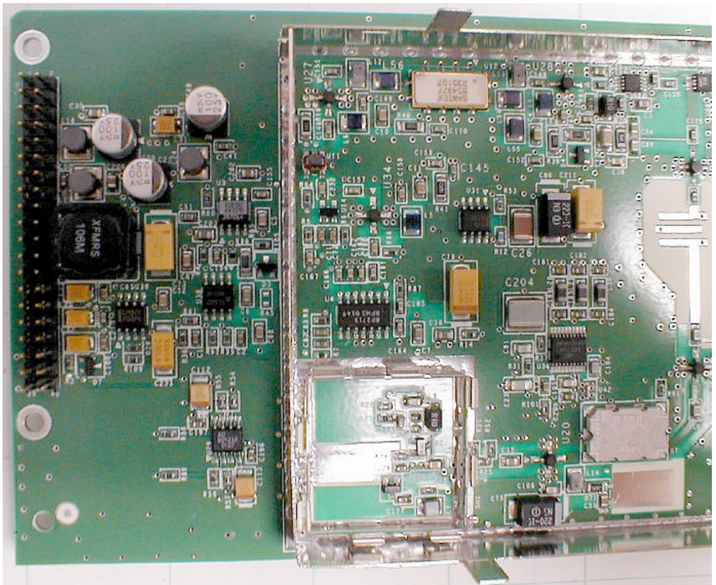
RFC Board Bottom Left Detail
