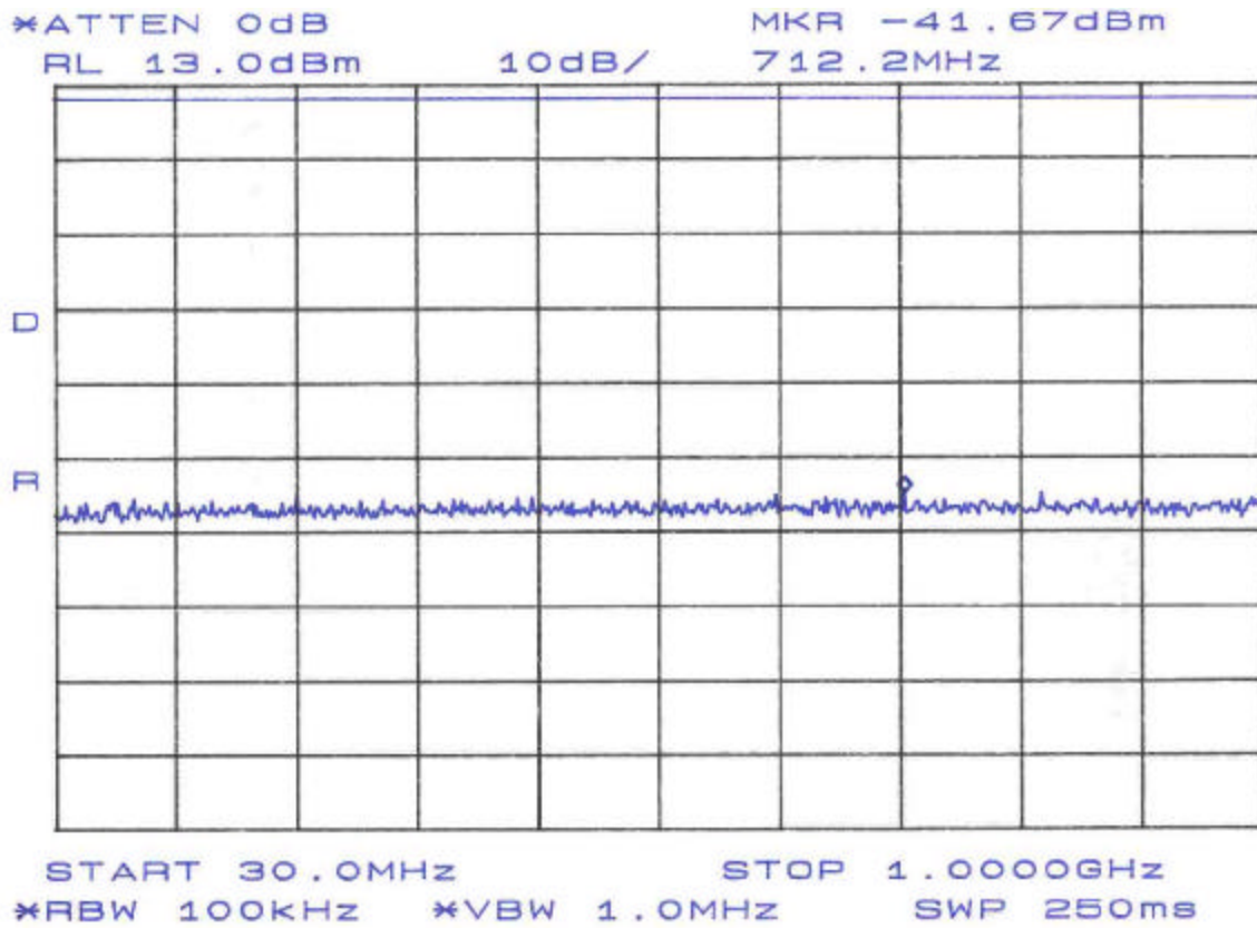
Figure 3. Conducted Spurious Emissions, Plan A, 30MHz-1GHz
