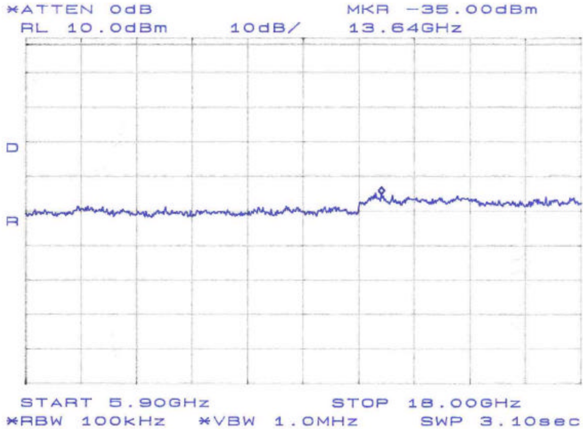
Figure 12. Conducted Spurious Emissions, Plan B, 5.9GHz-18GHz
