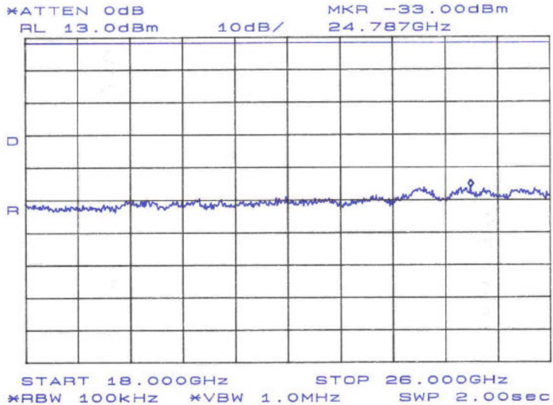
Figure 7. Conducted Spurious Emissions, Plan A, 18GHZ-26GHz
