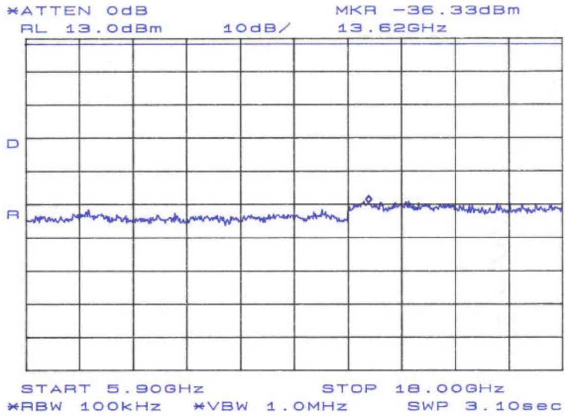
Figure 6. Conducted Spurious Emissions, Plan A, 5.9GHz-18GHz
