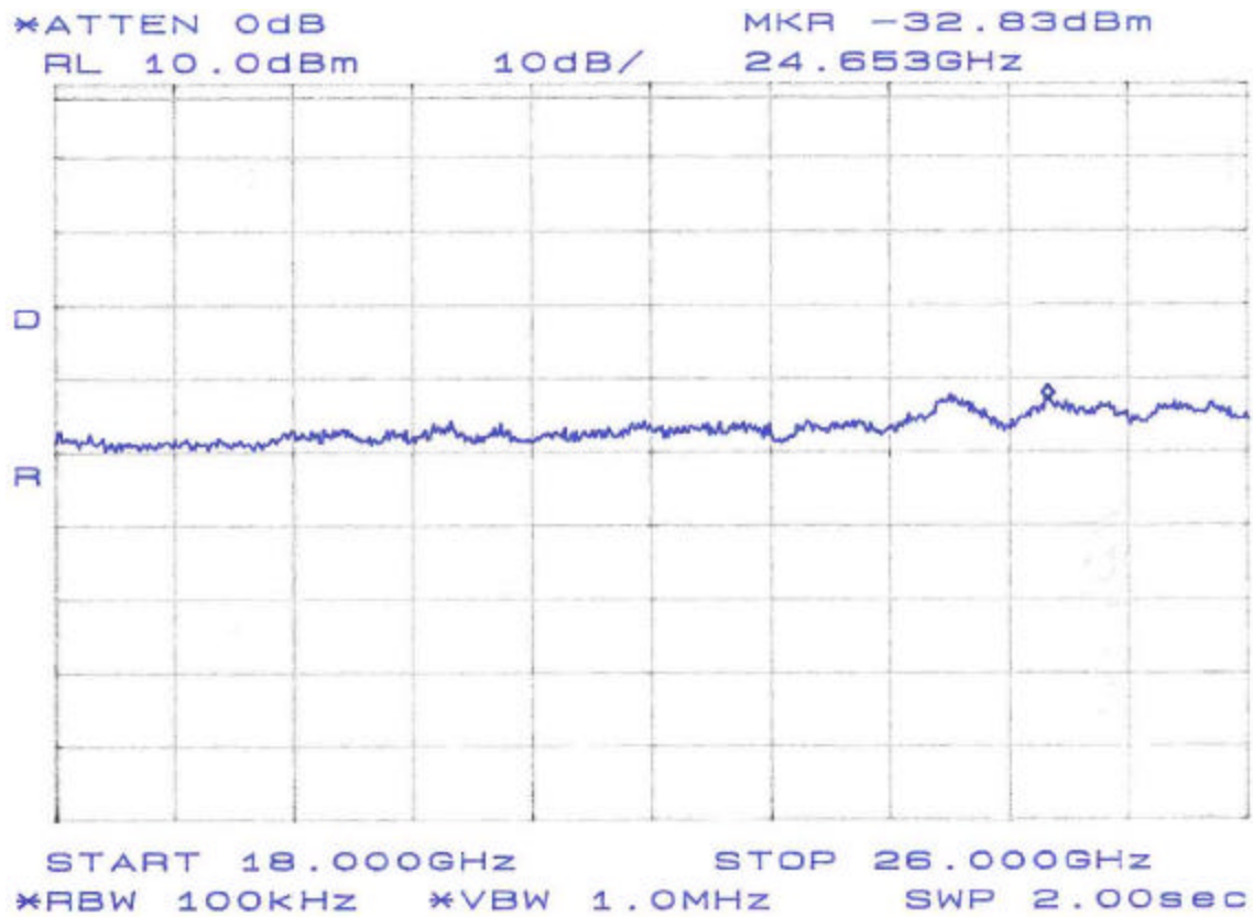
Figure 13. Conducted Spurious Emissions, Plan B, 18GHZ-26GHz
