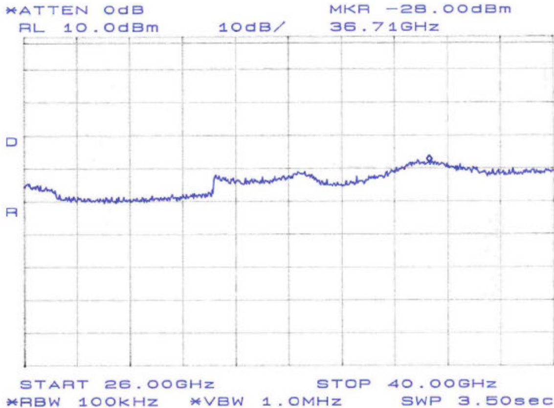
Figure 14. Conducted Spurious Emissions, Plan B, 26GHz-40GHz
