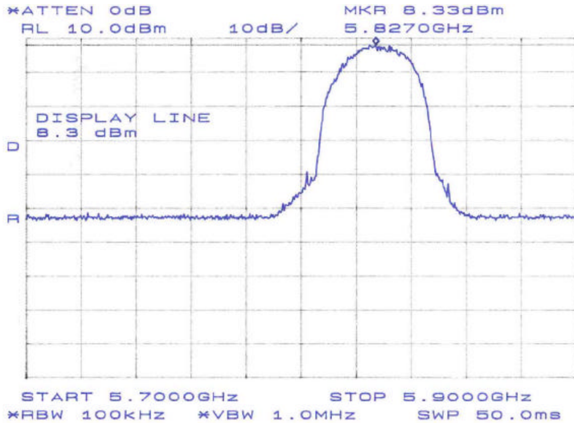
Figure 11. Conducted Spurious Emissions, Plan B, 5.7GHz-5.9GHz
