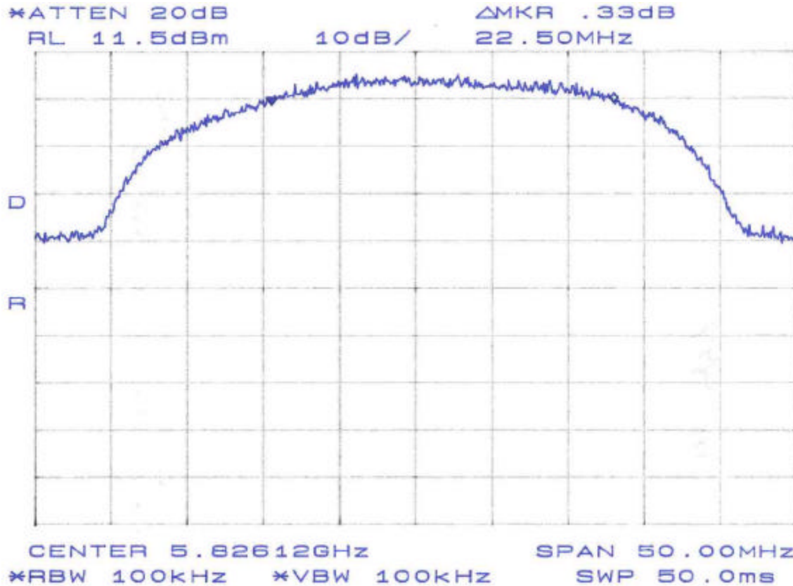
Figure 2. Occupied Bandwidth - Plan B
