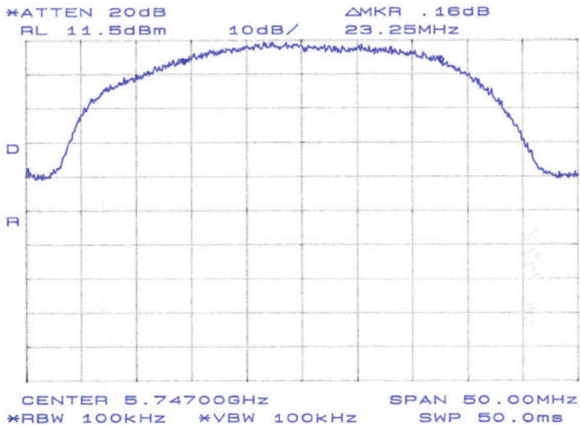
Figure 1. Occupied Bandwidth - Plan A
