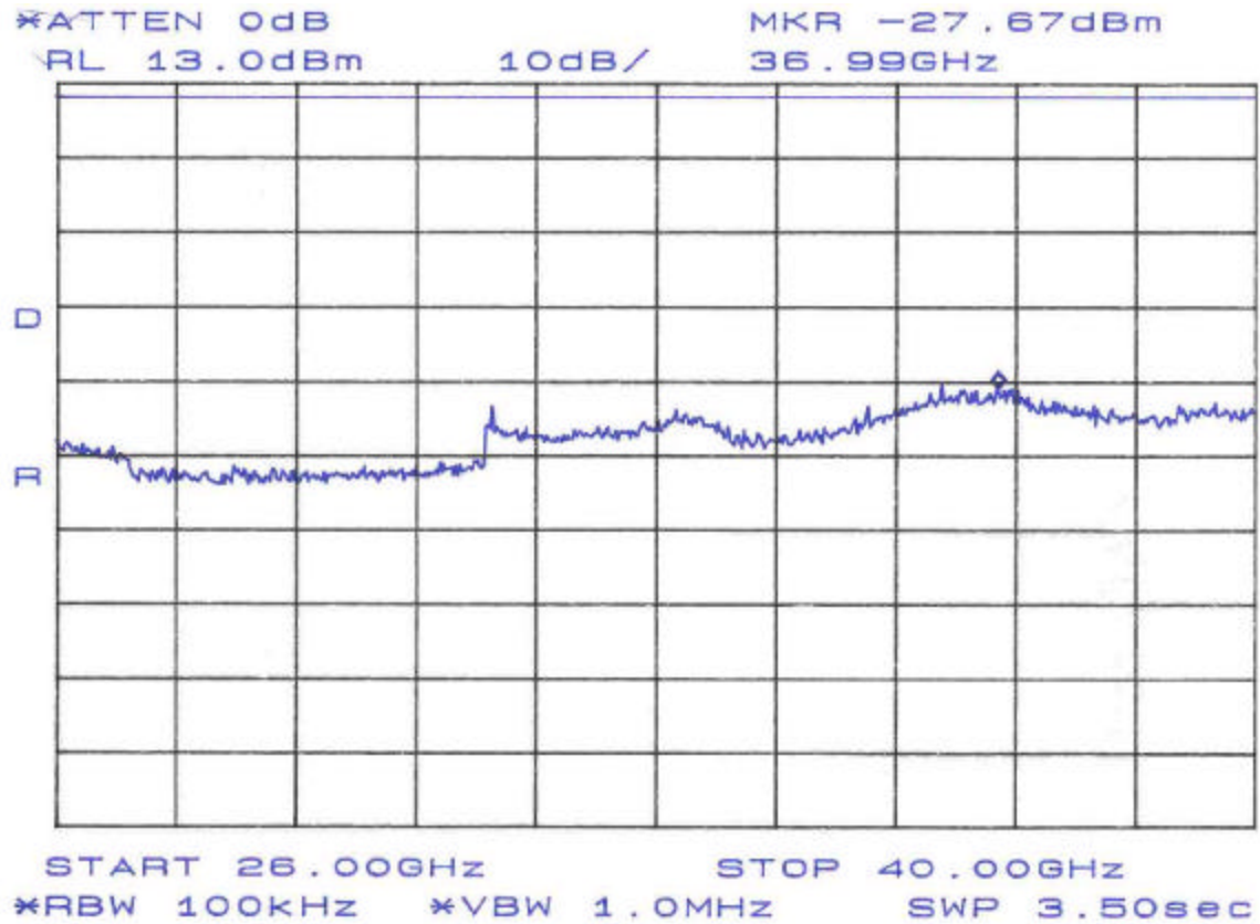
Figure 8. Conducted Spurious Emissions, Plan A, 26GHz-40GHz
