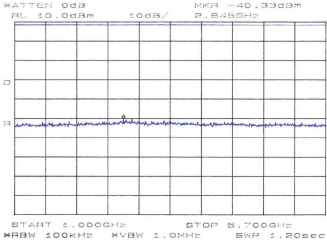
Figure 10. Conducted Spurious Emissions, Plan B, 1GHz-5.7GHz
