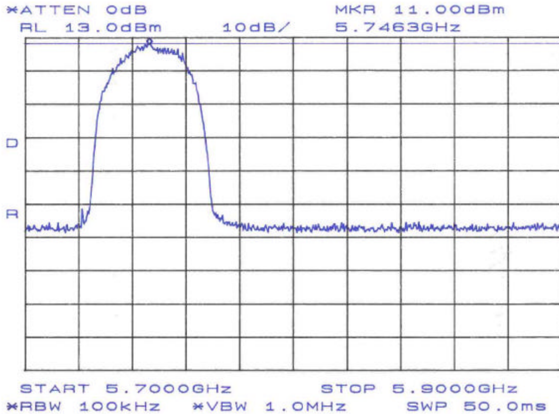
Figure 5. Conducted Spurious Emissions, Plan A, 5.7GHz-5.9GHz
