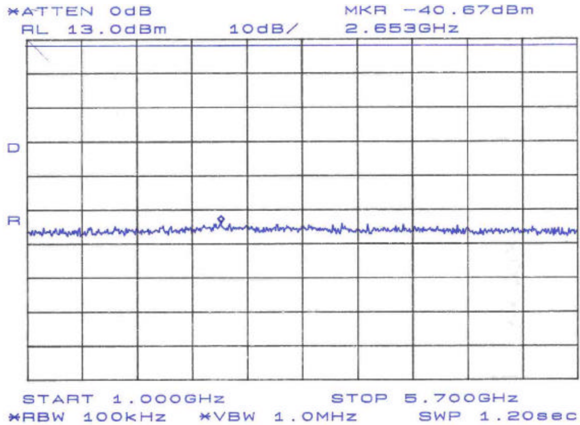
Figure 4. Conducted Spurious Emissions, Plan A, 1GHz-5.7GHz
