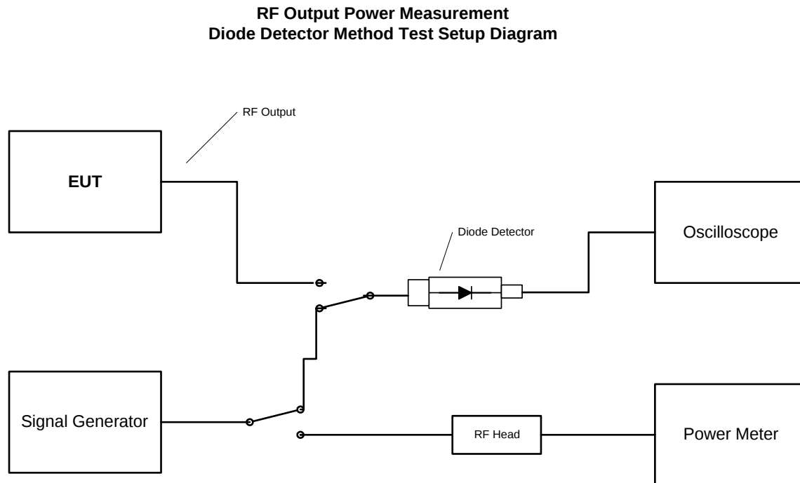
Figure 4-1: RF Power Measurement Test Setup Diagram
