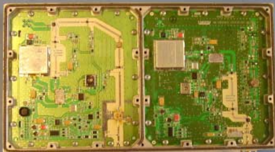
RF ASSY - TOP VIEW
