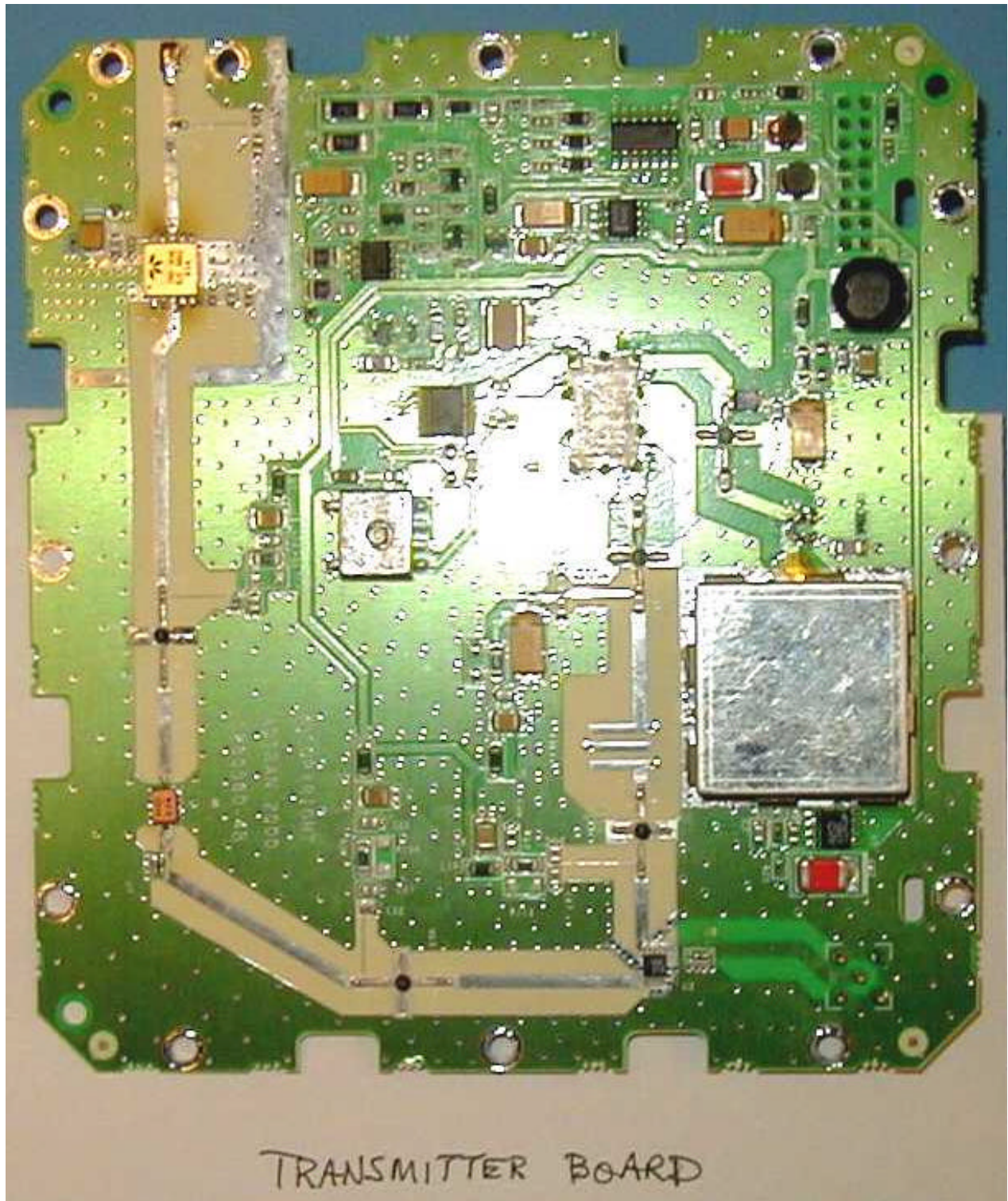
Transmitter PCB, Top
