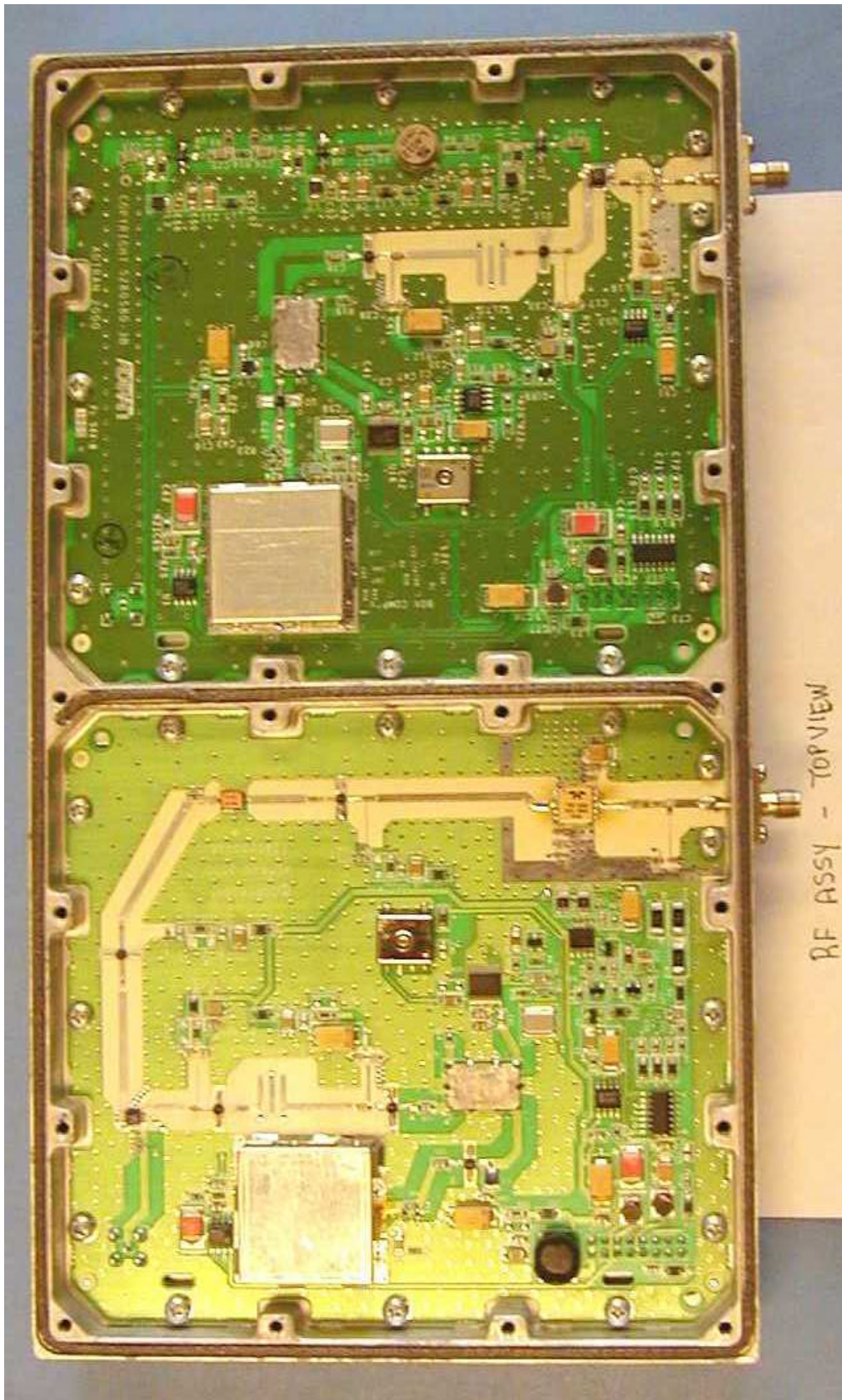
RF Top View
