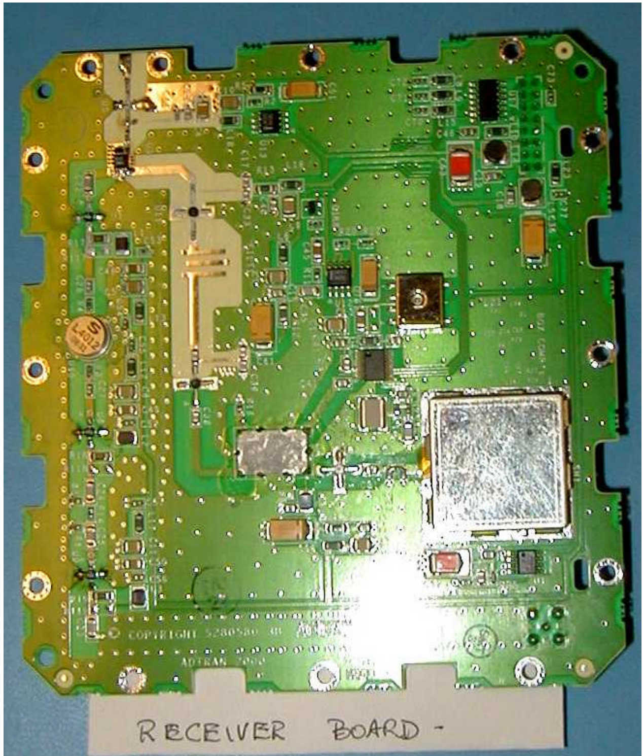
Receiver PCB, Top
