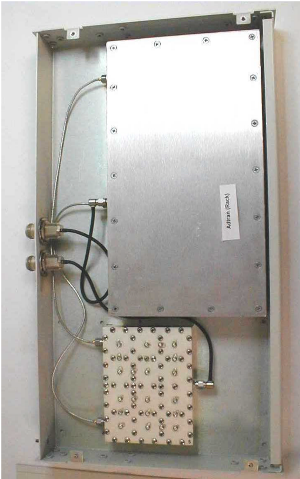
Rack Mount, Cover Off
