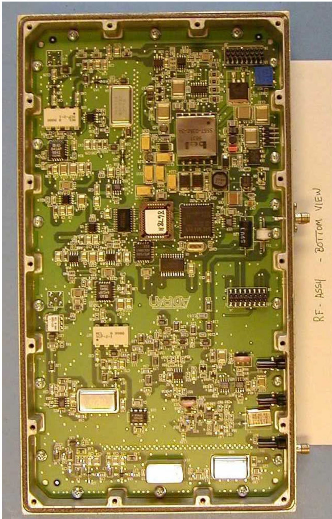
RF Bottom View
