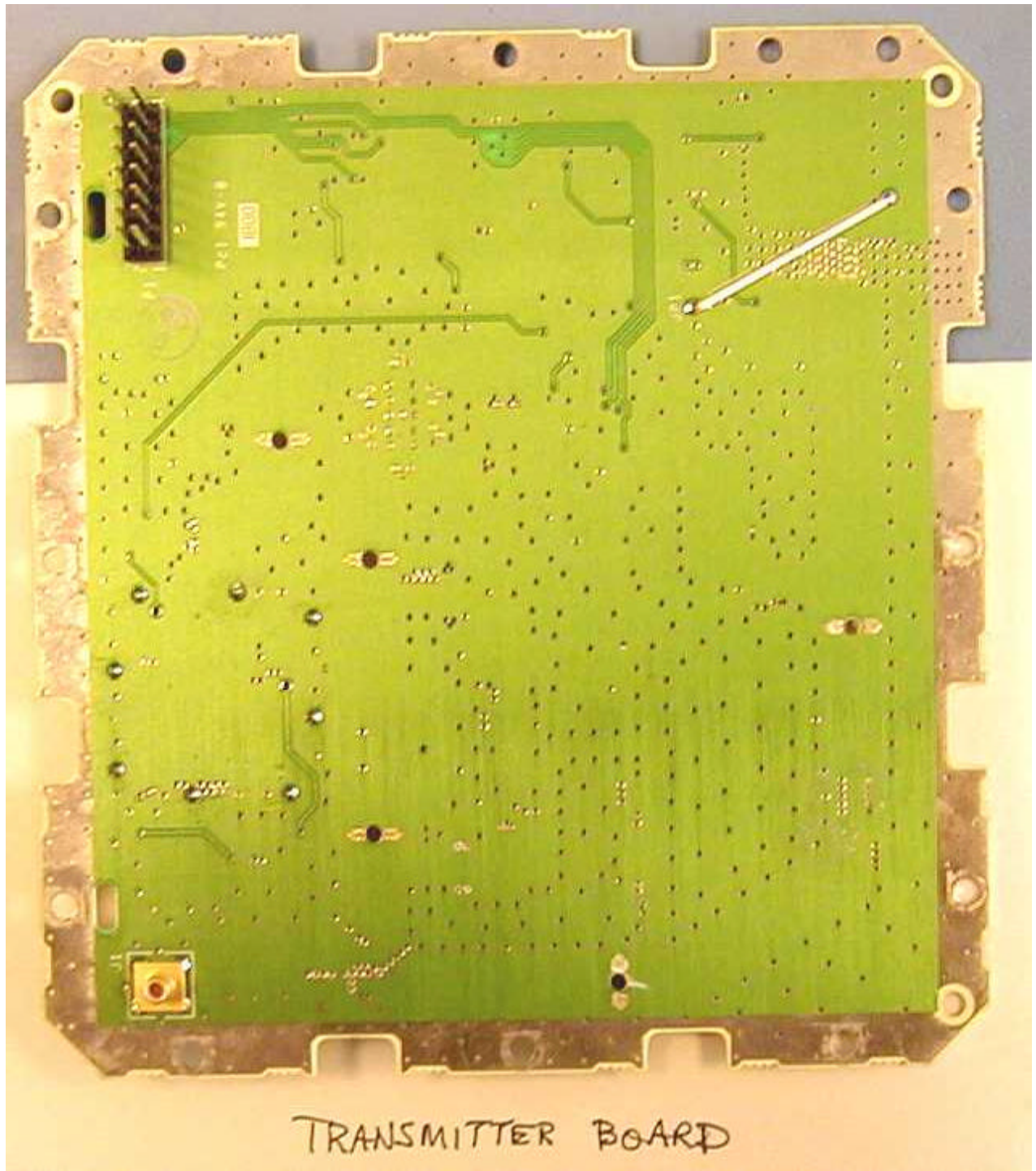
Transmitter PCB, Bottom
