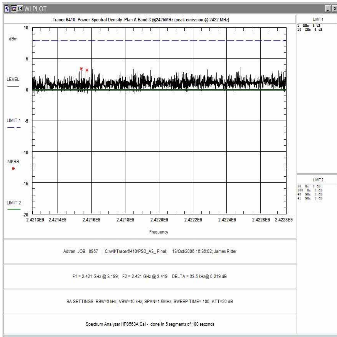
Figure 10. Power Spectral Density Plan A, Band 3
