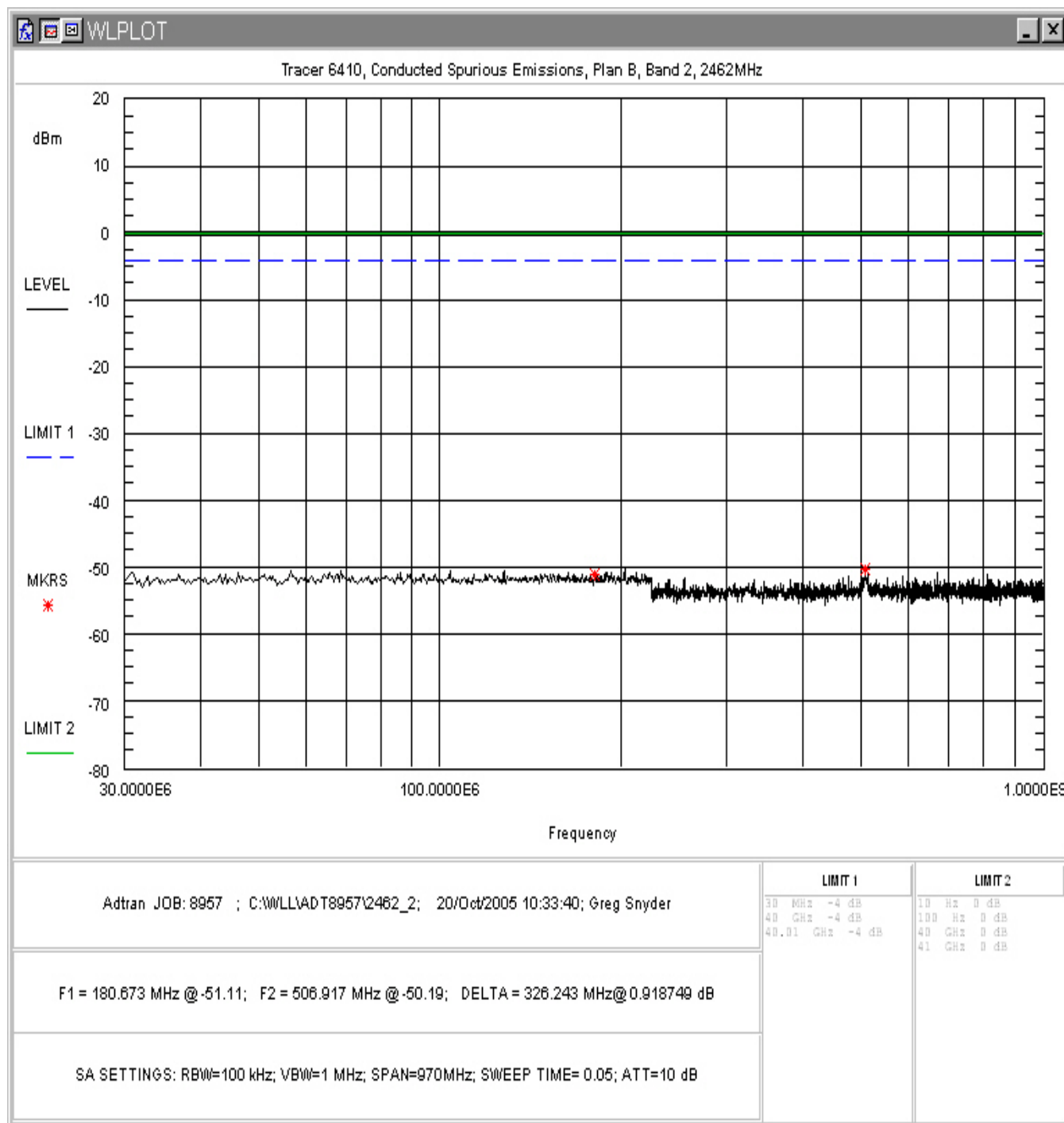
Figure 30. Conducted Spurious Emissions, Plan B Band 2, 30MHz - 1GHz
