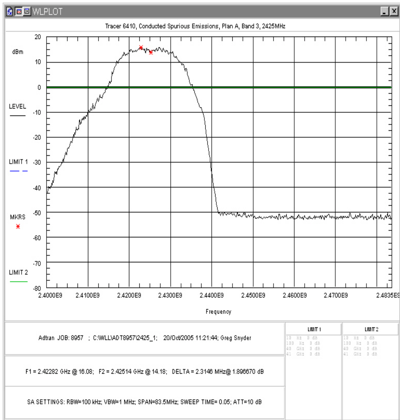
Figure 24. Conducted Spurious Emissions, Plan A Band 3, Inband
