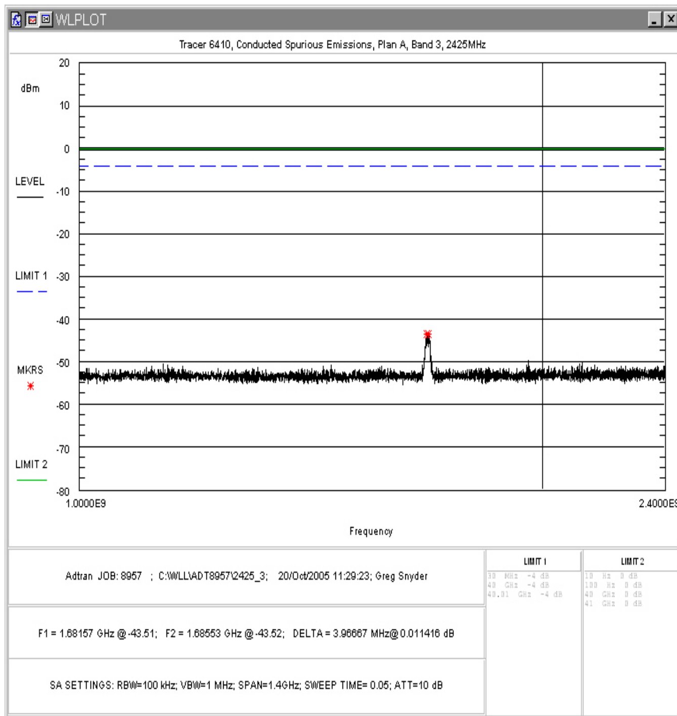
Figure 23. Conducted Spurious Emissions, Plan A Band 3, 1GHz – 2.4GHz
