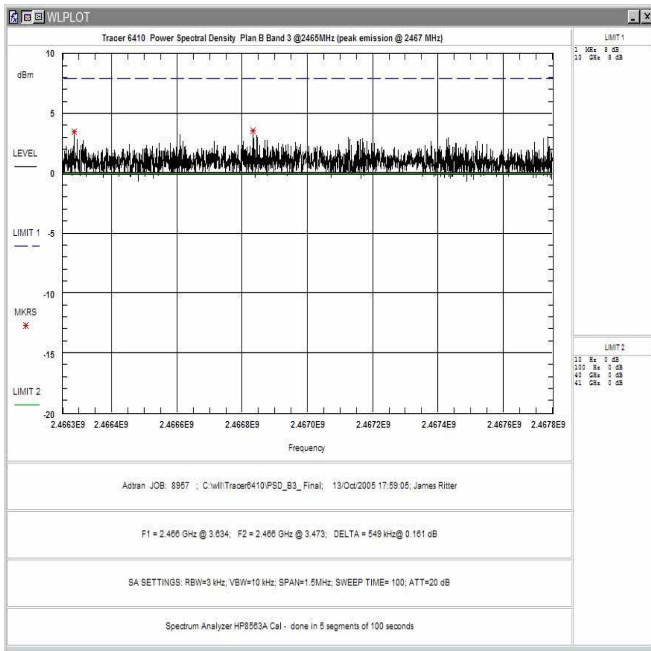
Figure 13. Power Spectral Density Plan B, Band 3
