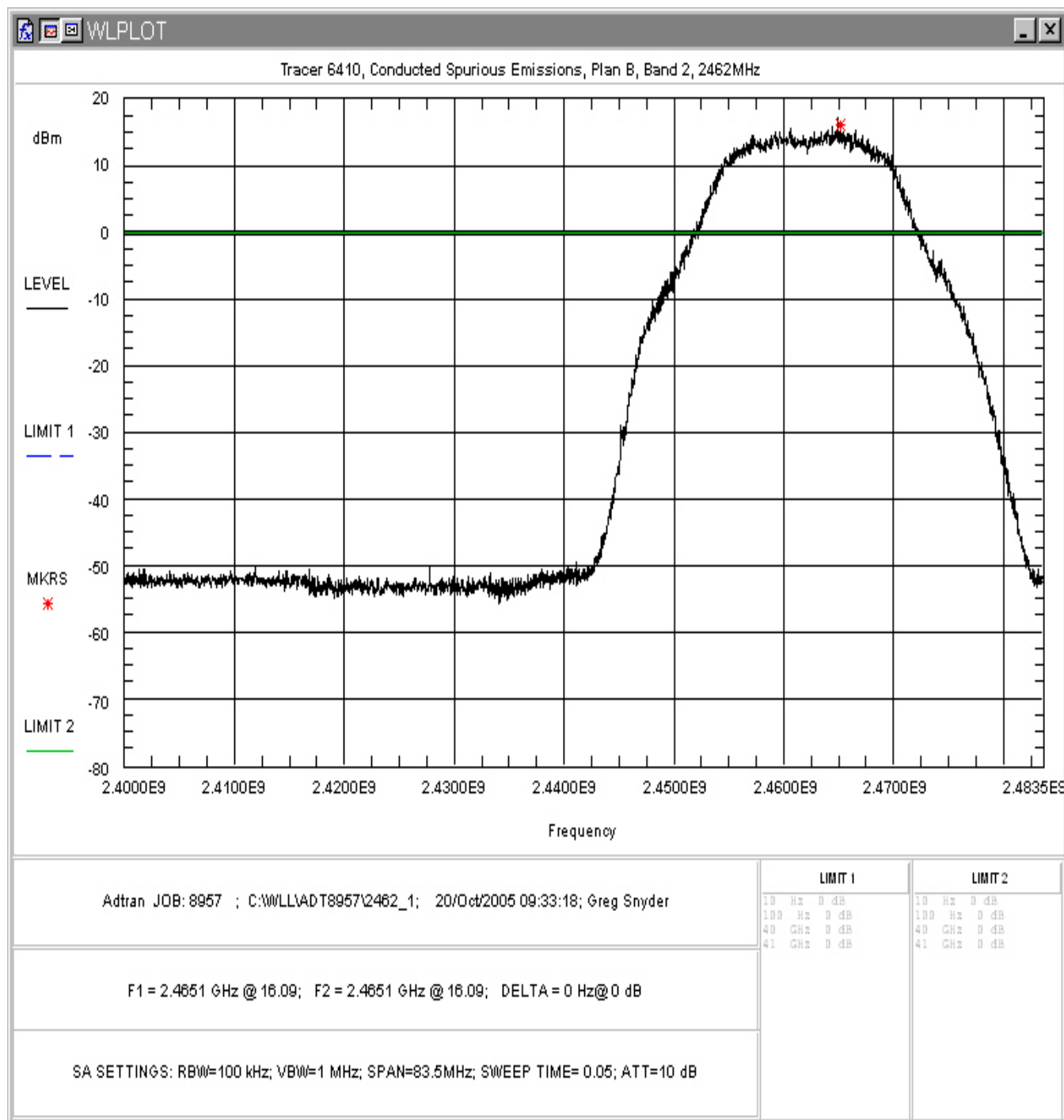
Figure 32. Conducted Spurious Emissions, Plan B Band 2, Inband
