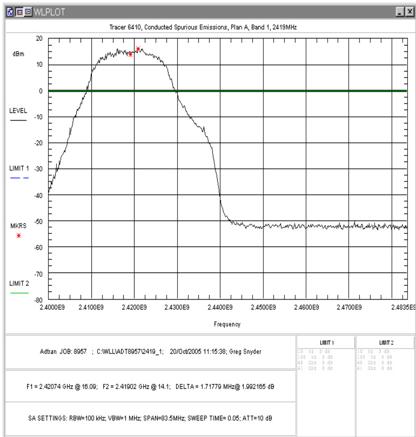
Figure 16. Conducted Spurious Emissions, Plan A Band 1, Inband
