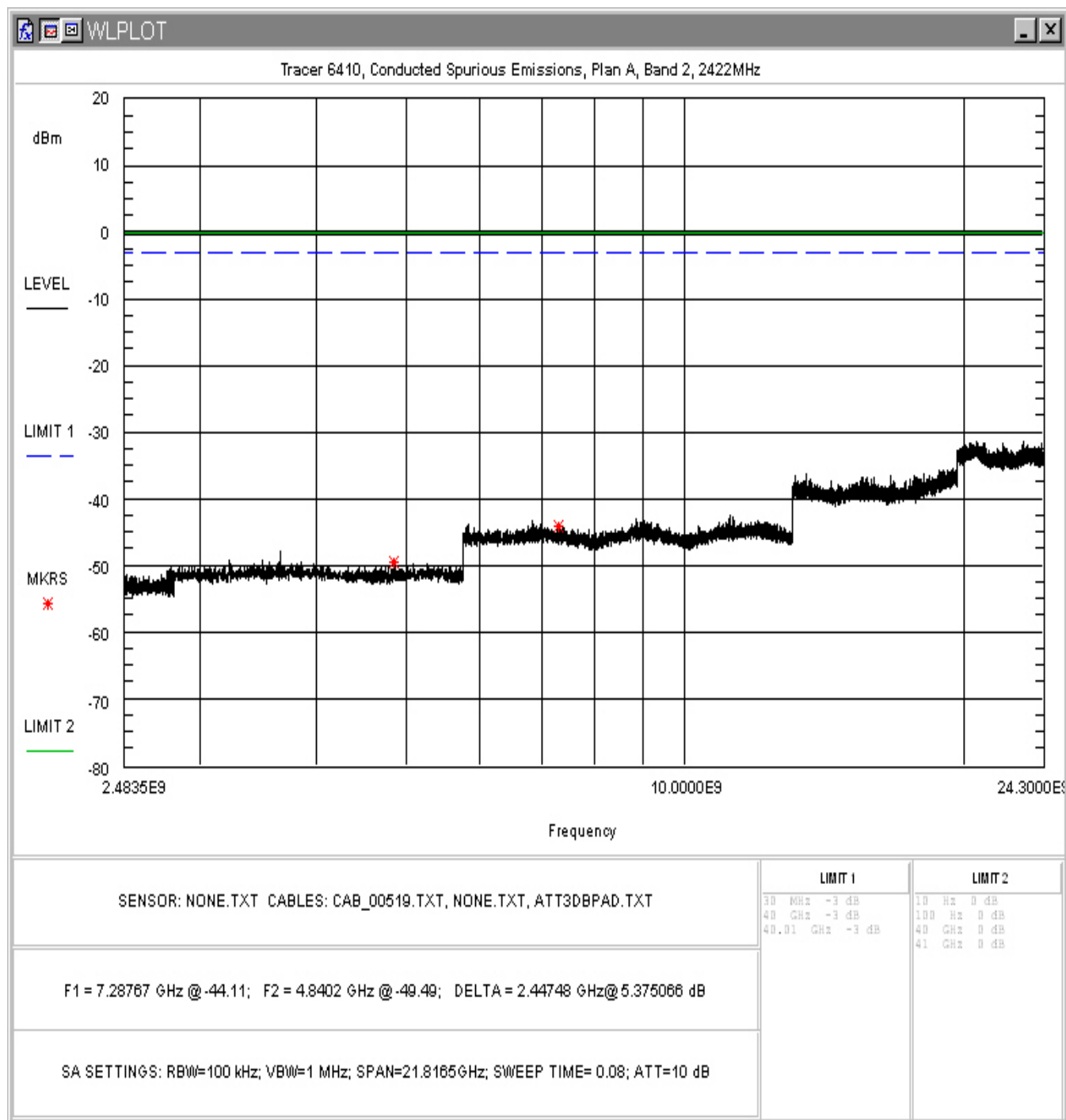
Figure 21. Conducted Spurious Emissions, Plan A Band 2, 2.4835 – 24.3GHz
