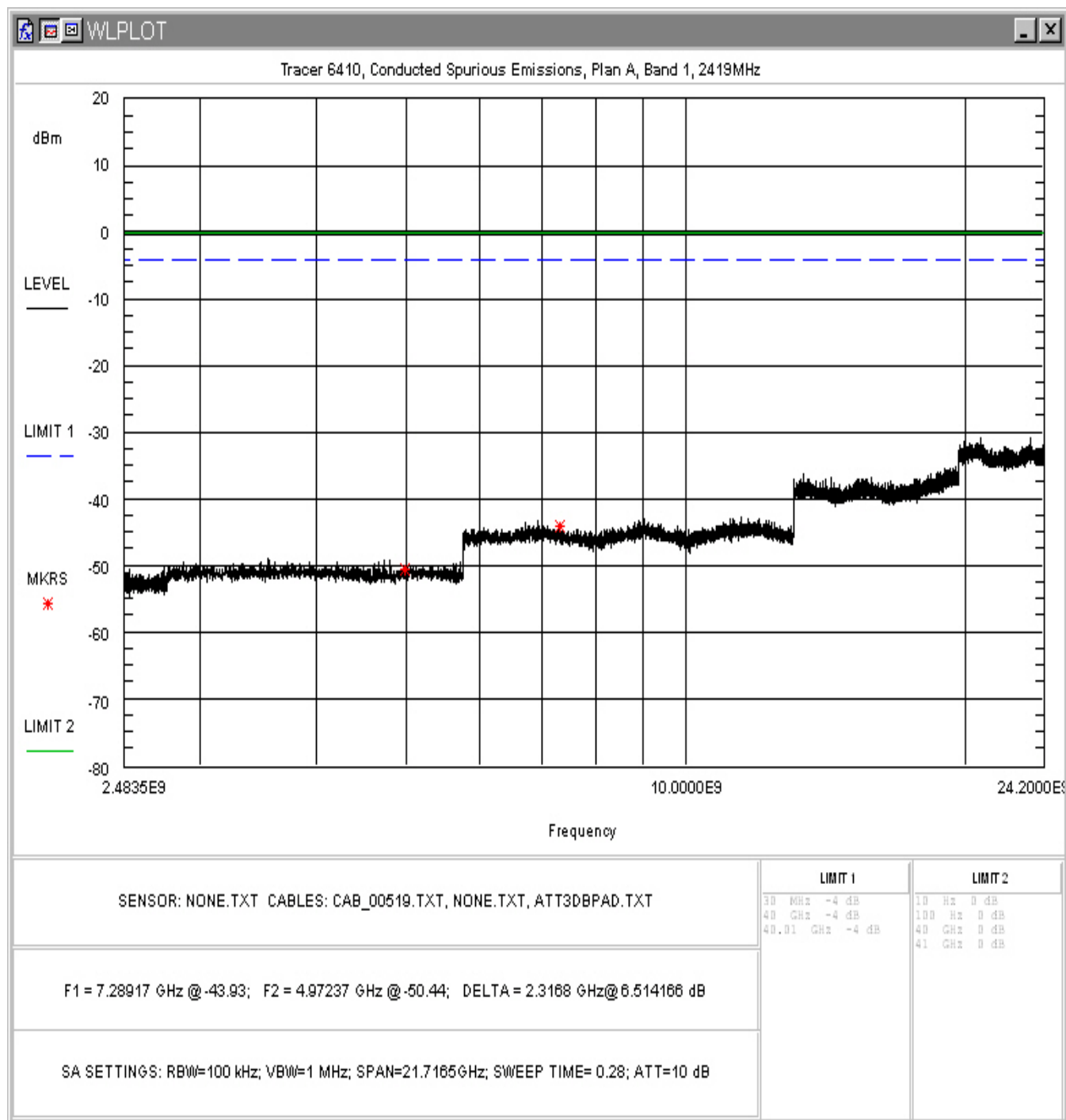
Figure 17. Conducted Spurious Emissions, Plan A Band 1, 2.4835 – 24.2GHz
