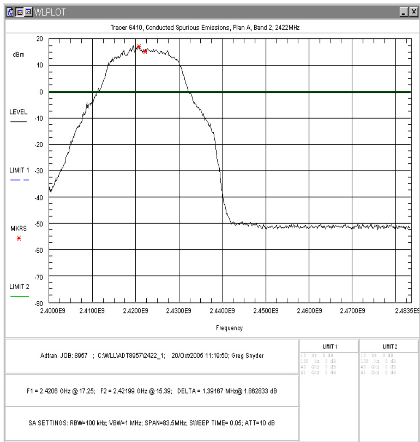
Figure 20. Conducted Spurious Emissions, Plan A Band 2, Inband
