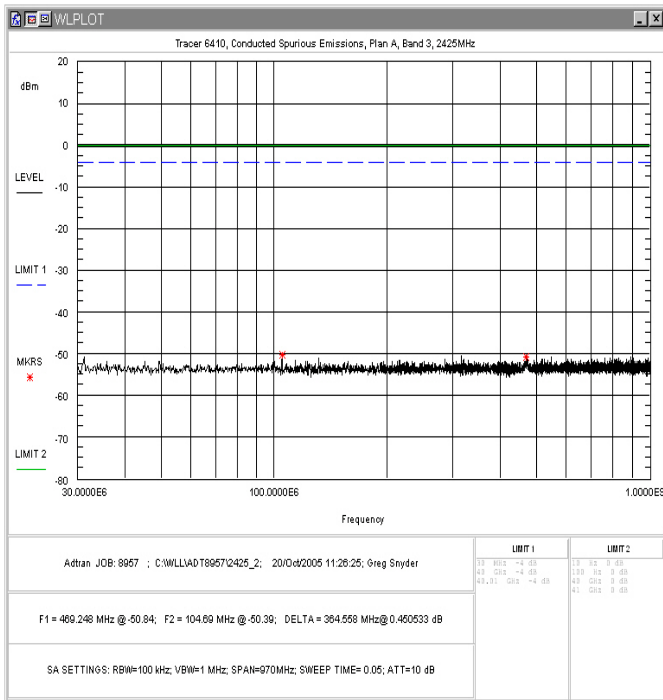
Figure 22. Conducted Spurious Emissions, Plan A Band 3, 30MHz - 1GHz
