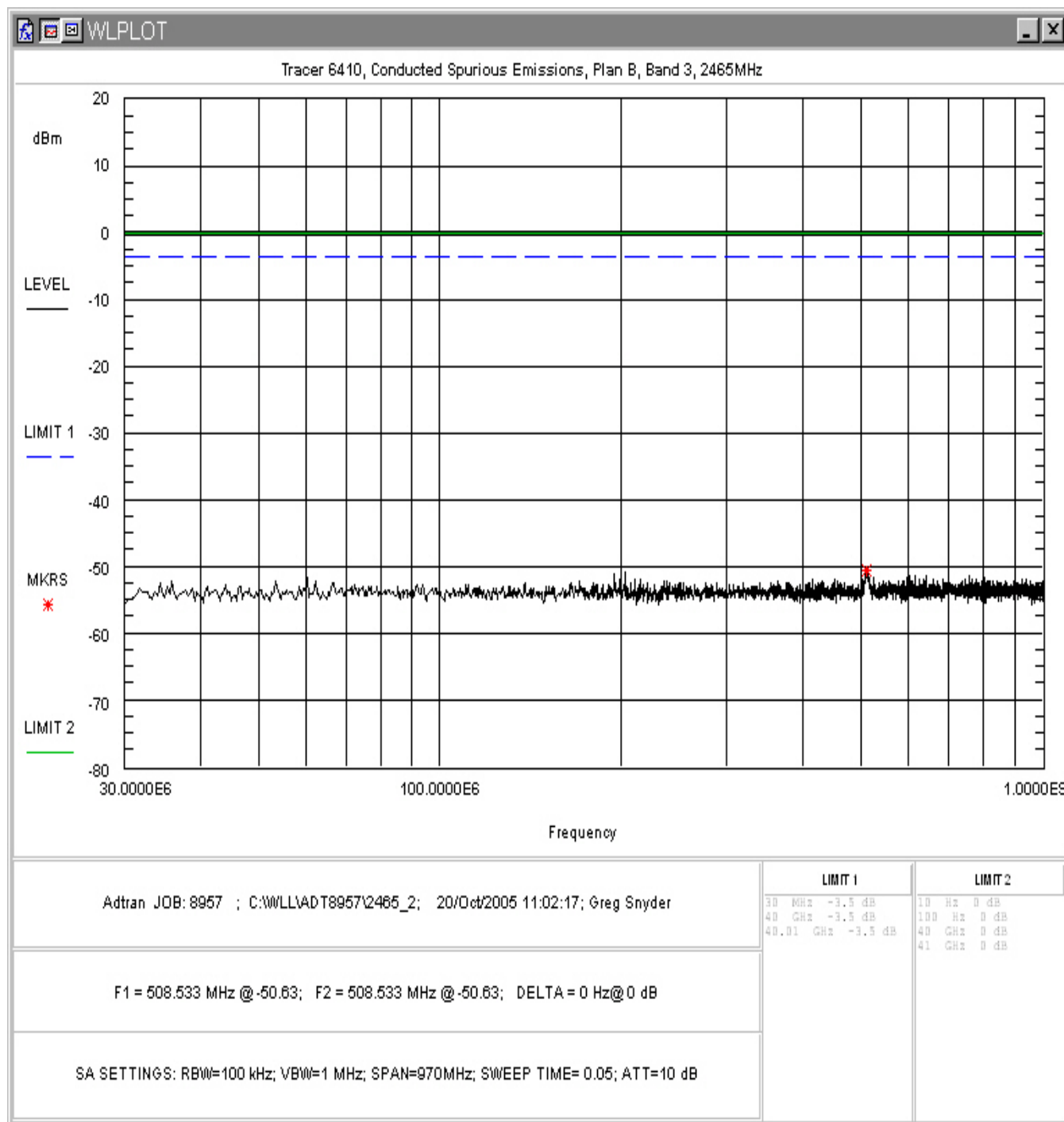
Figure 34. Conducted Spurious Emissions, Plan B Band 3, 30MHz - 1GHz
