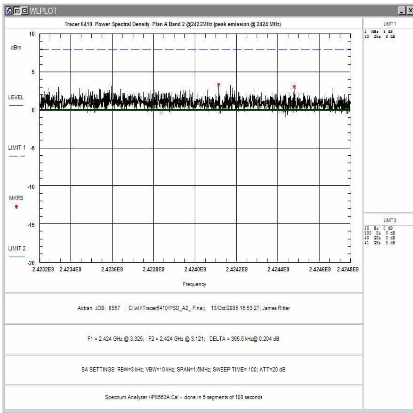
Figure 9. Power Spectral Density Plan A, Band 2
