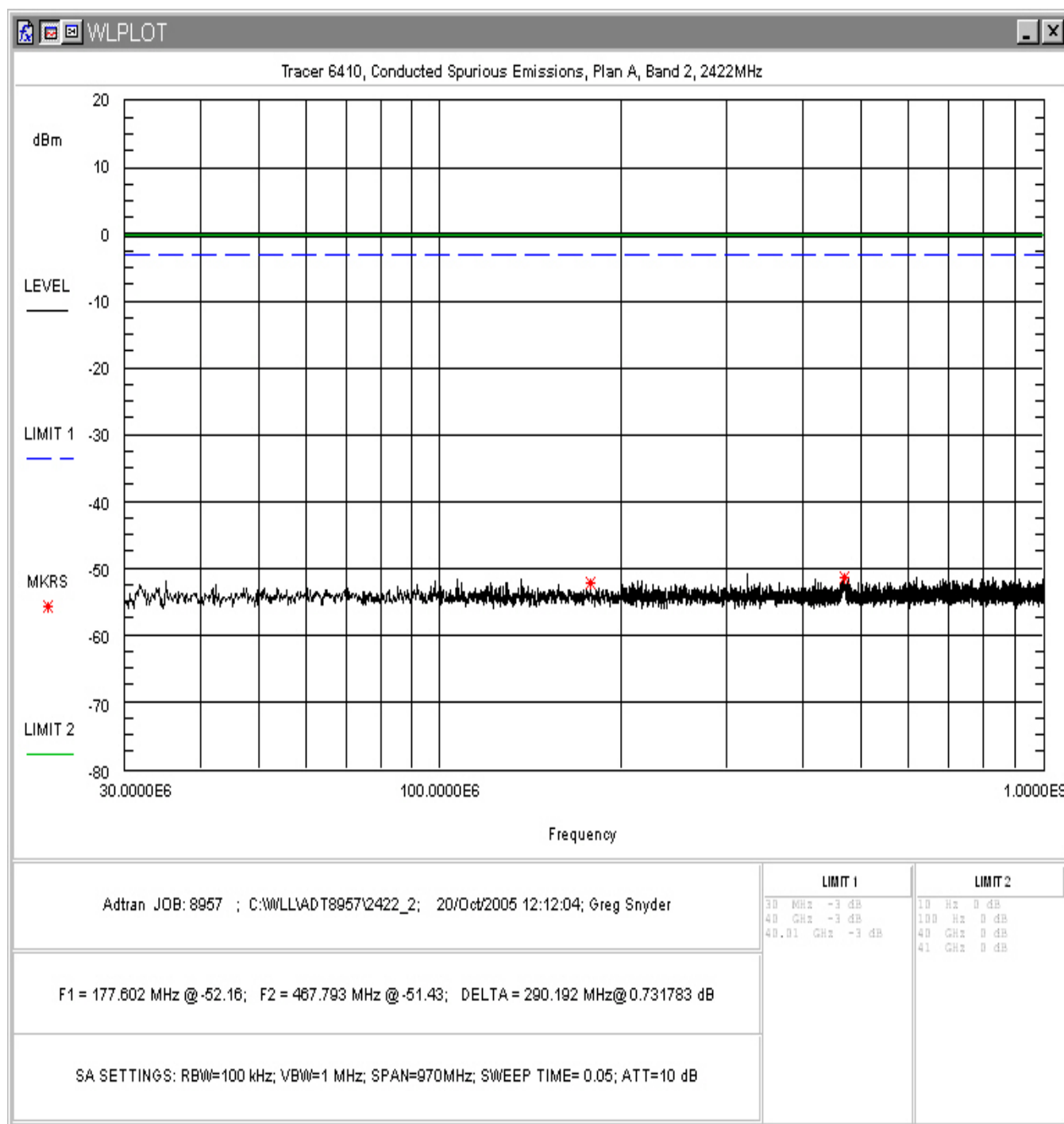
Figure 18. Conducted Spurious Emissions, Plan A Band 2, 30MHz - 1GHz
