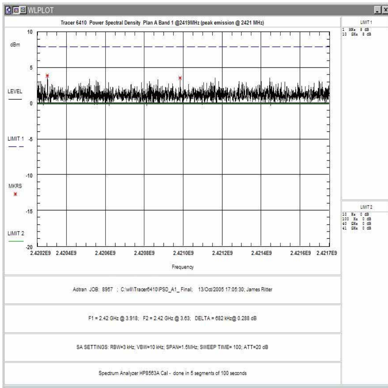
Figure 8. Power Spectral Density Plan A, Band 1
