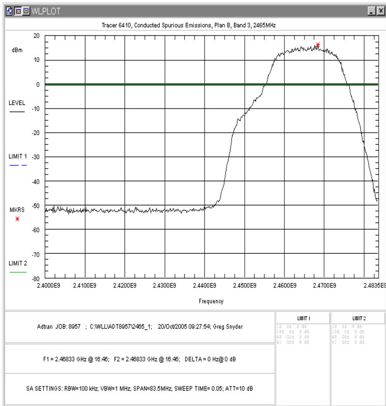
Figure 36. Conducted Spurious Emissions, Plan B Band 3, Inband
