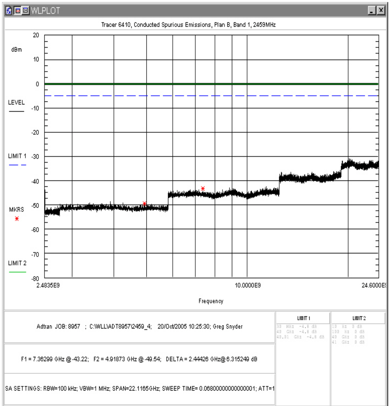
Figure 29. Conducted Spurious Emissions, Plan B Band 1, 2.4835 – 24.6GHz
