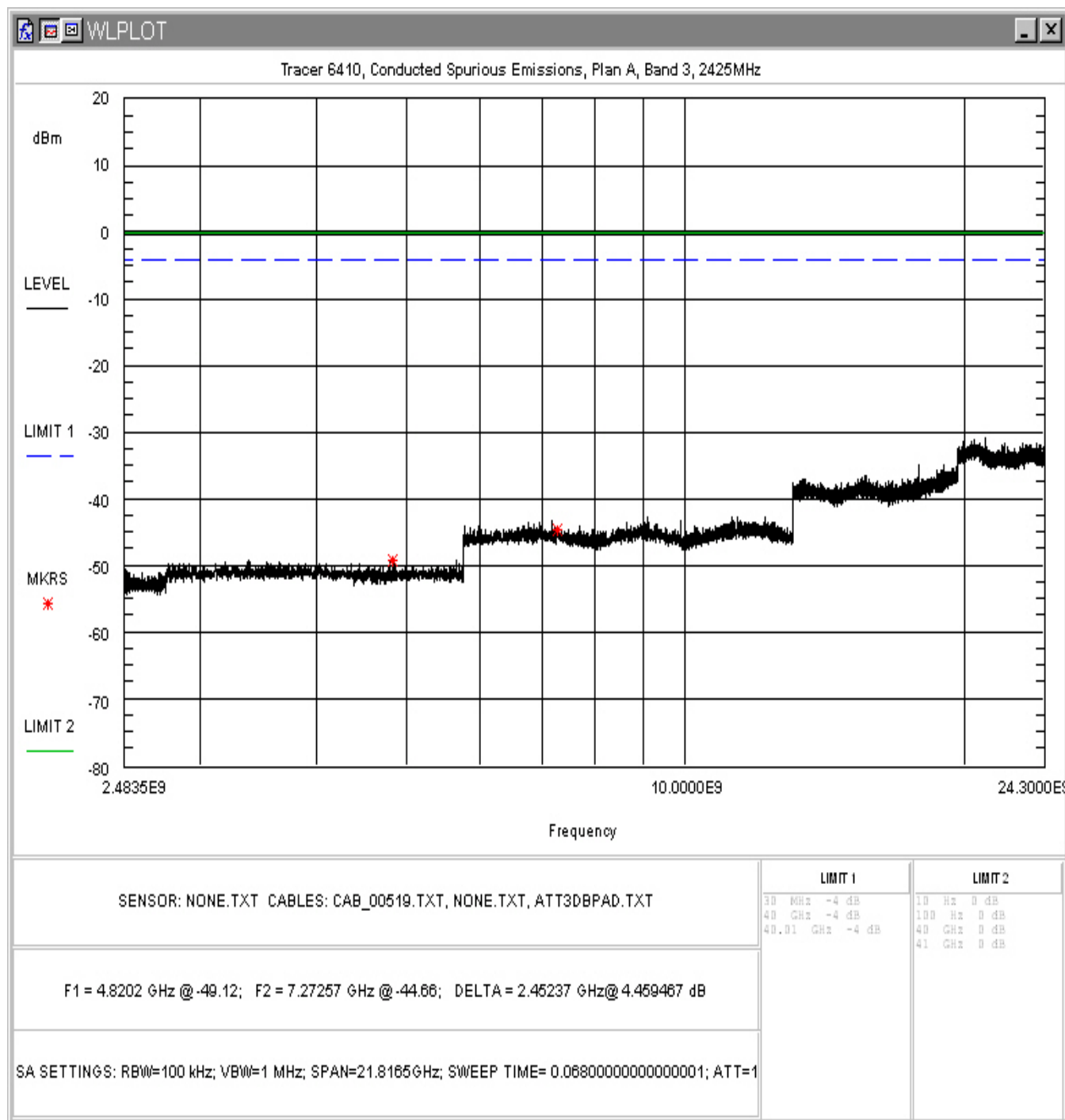
Figure 25. Conducted Spurious Emissions, Plan A Band 3, 2.4835 – 24.3GHz
