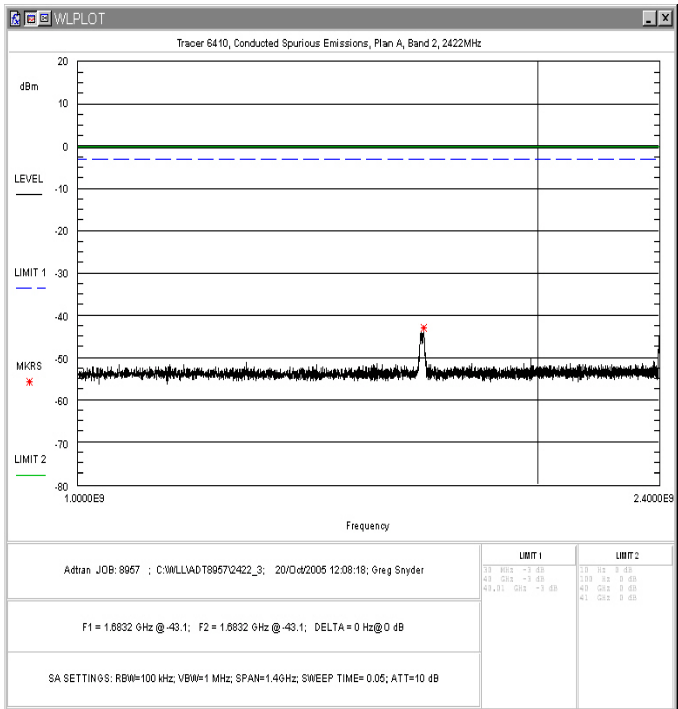
Figure 19. Conducted Spurious Emissions, Plan A Band 2, 1GHz – 2.4GHz
