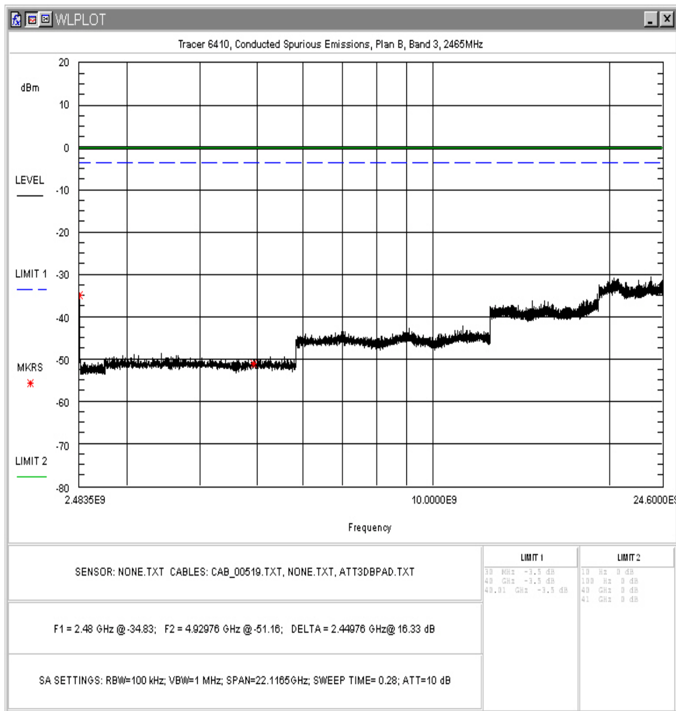
Figure 37. Conducted Spurious Emissions, Plan B Band 3, 2.4835 – 24.6GHz
