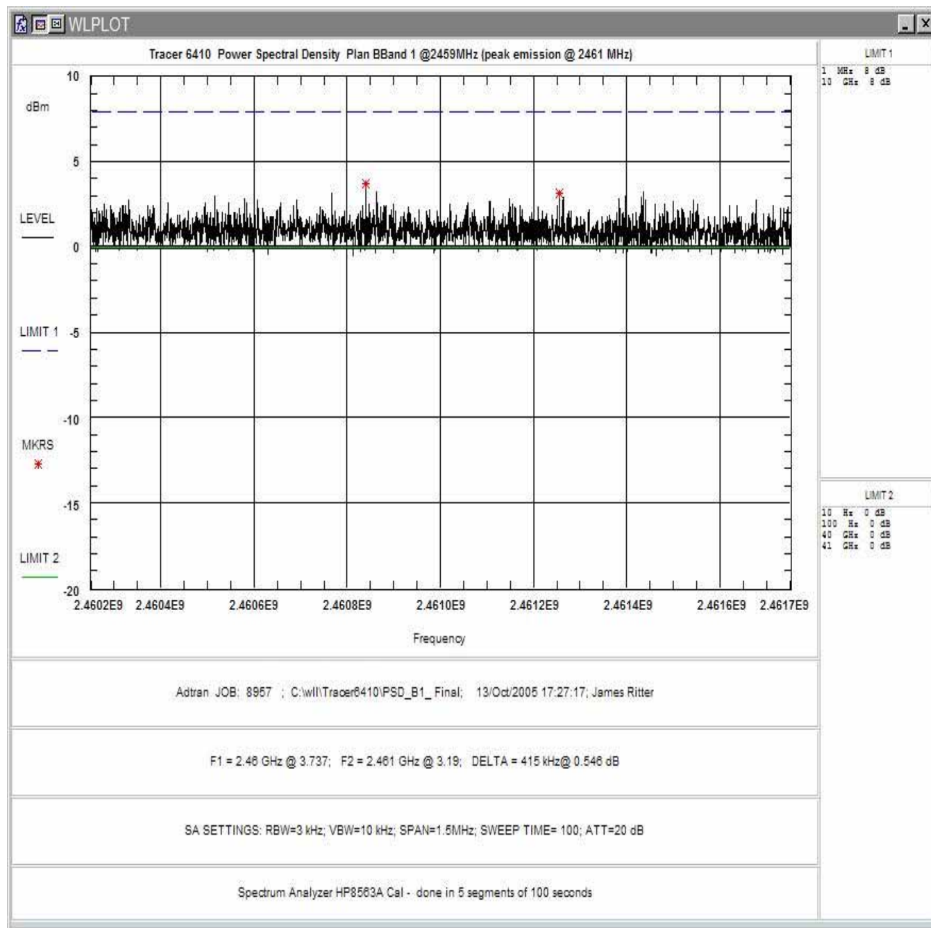
Figure 11. Power Spectral Density Plan B, Band 1
