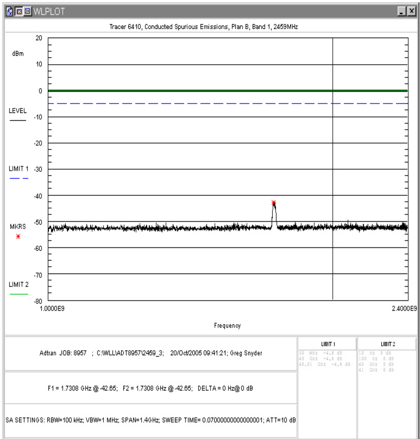
Figure 27. Conducted Spurious Emissions, Plan B Band 1, 1GHz – 2.4GHz
