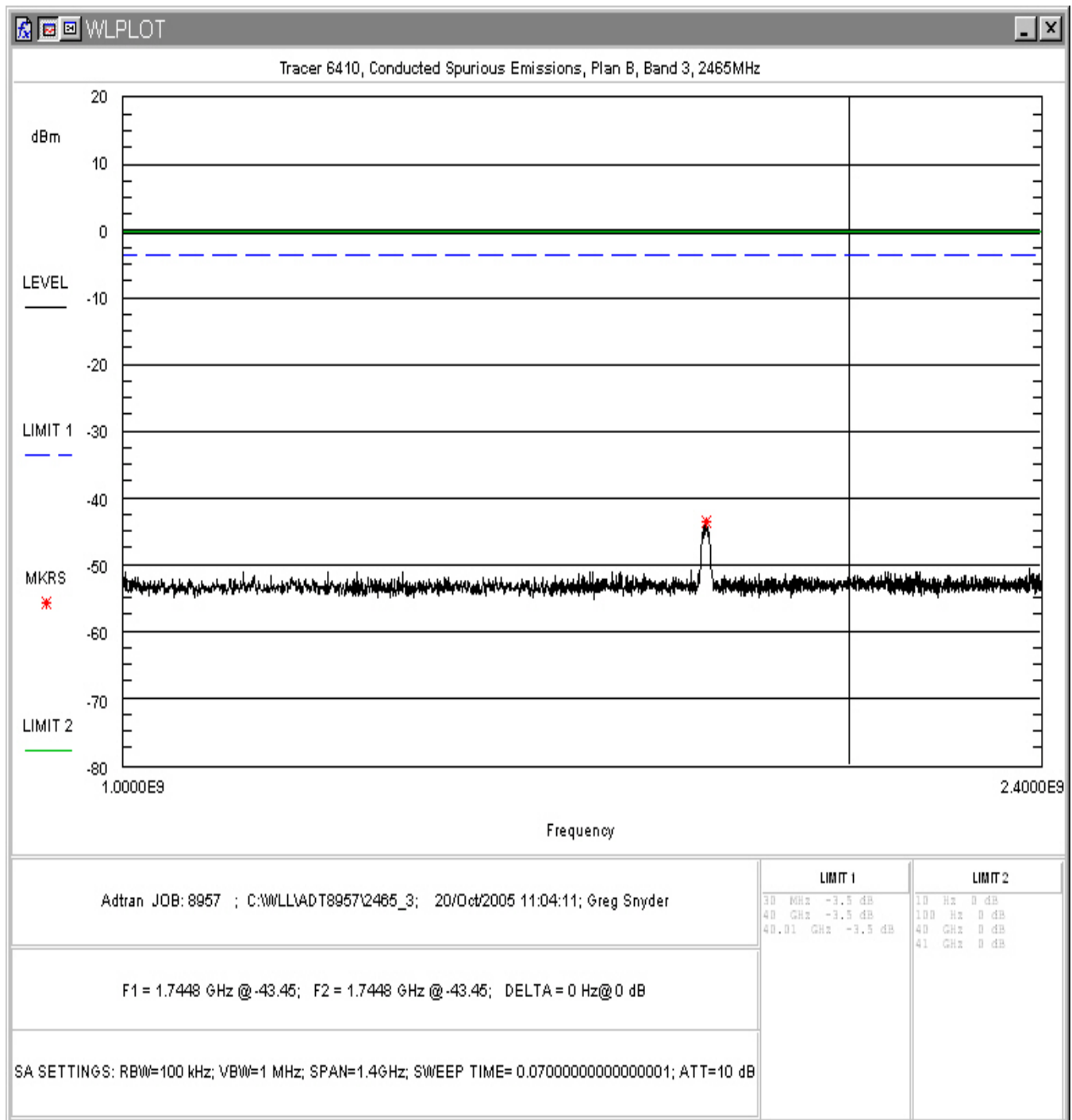
Figure 35. Conducted Spurious Emissions, Plan B Band 3, 1GHz – 2.4GHz
