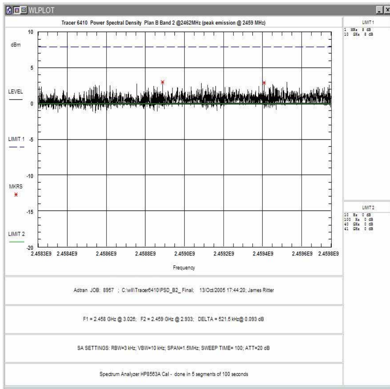
Figure 12. Power Spectral Density Plan B, Band 2
