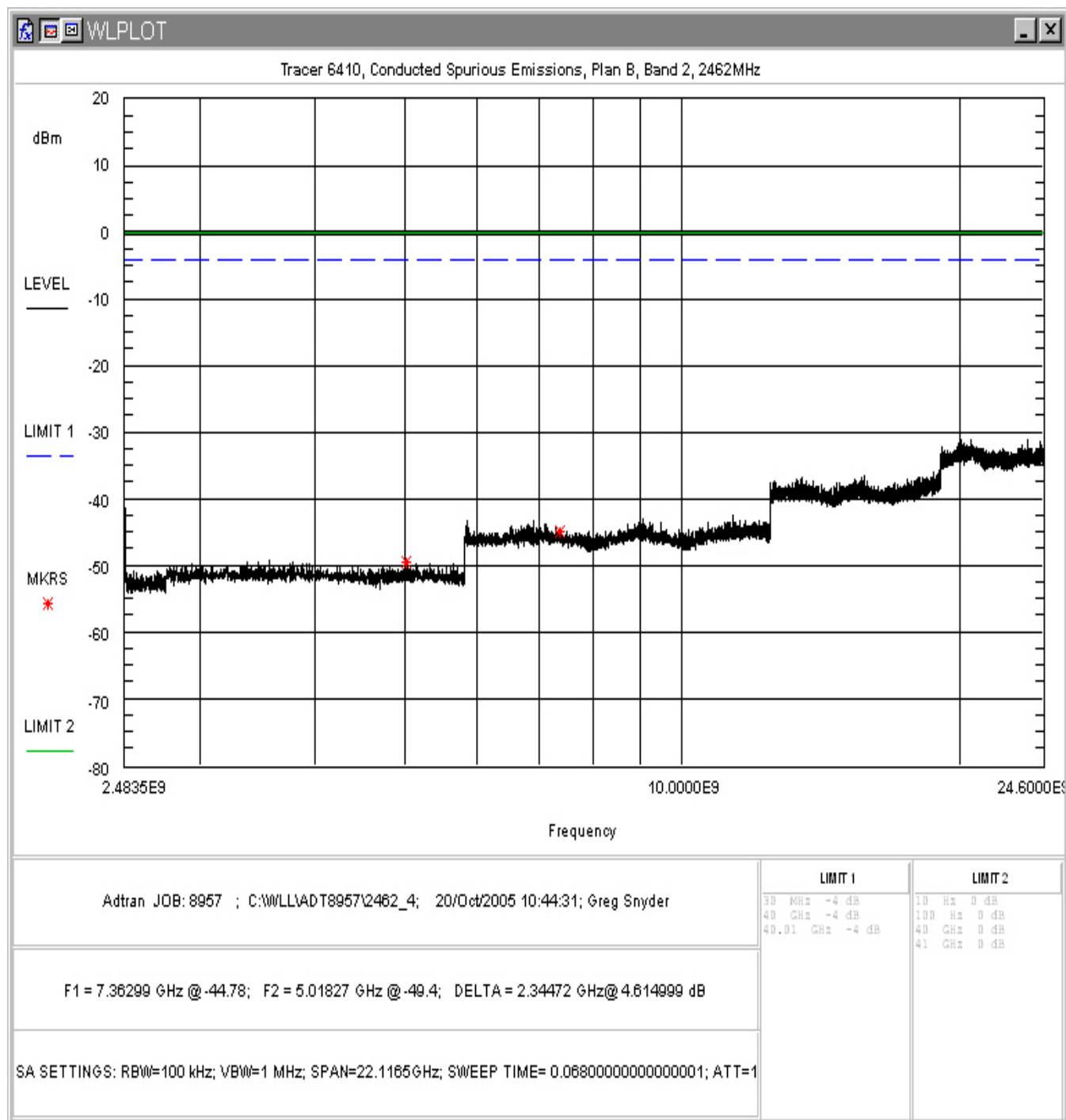
Figure 33. Conducted Spurious Emissions, Plan B Band 2, 2.4835 – 24.6GHz
