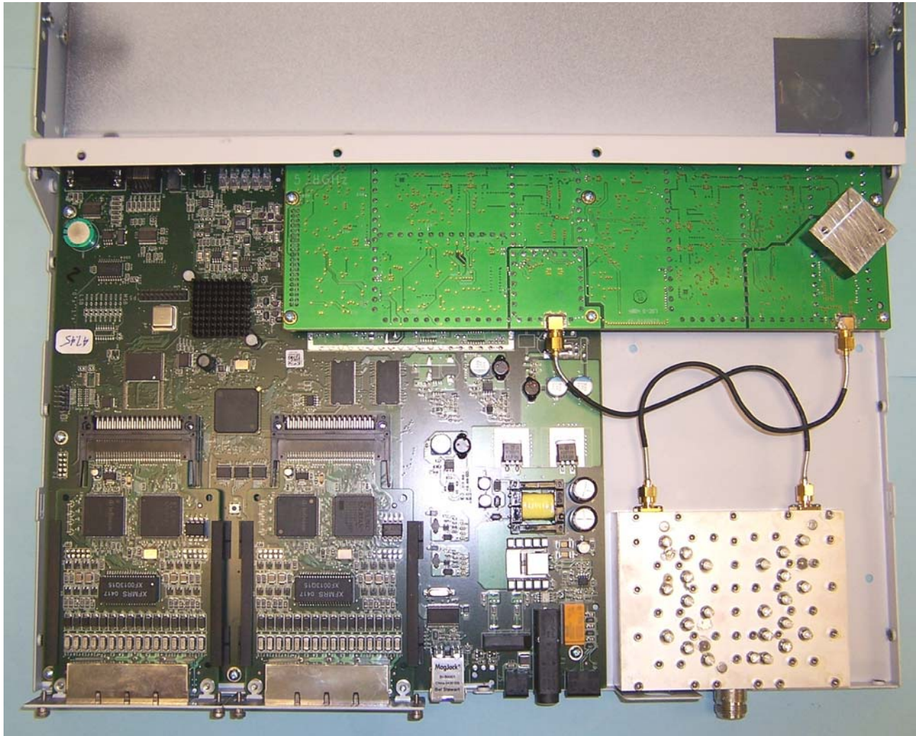
Cover Removed
