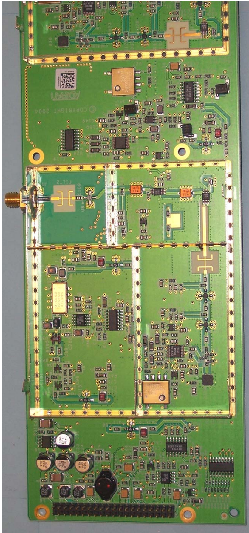
RF Board Bottom Left, No Shields
