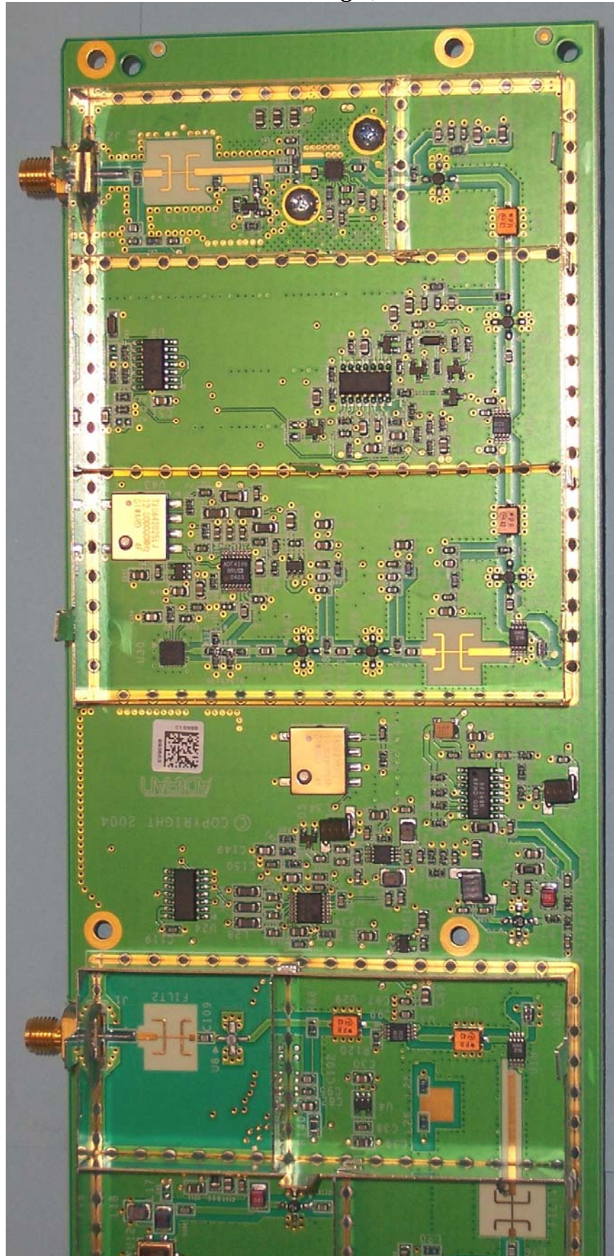
RF Board Bottom Right, No Shields
