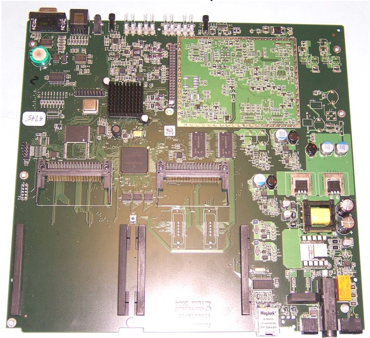
Baseboard Bottom
