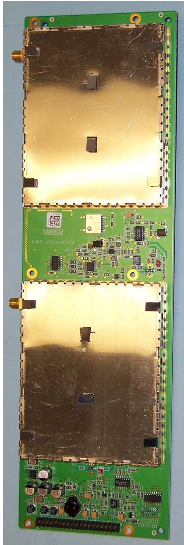
RF Board Bottom with Shields
