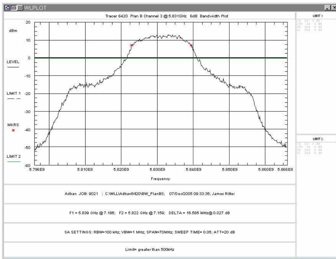
Figure 5. Occupied Bandwidth - Plan B, Band 3
