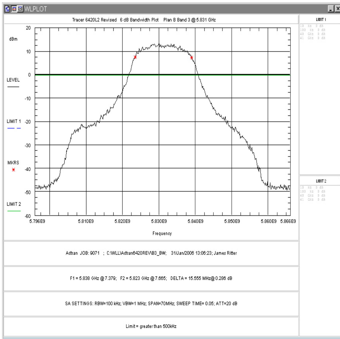
Figure 5. Occupied Bandwidth - Plan B, Band 3
