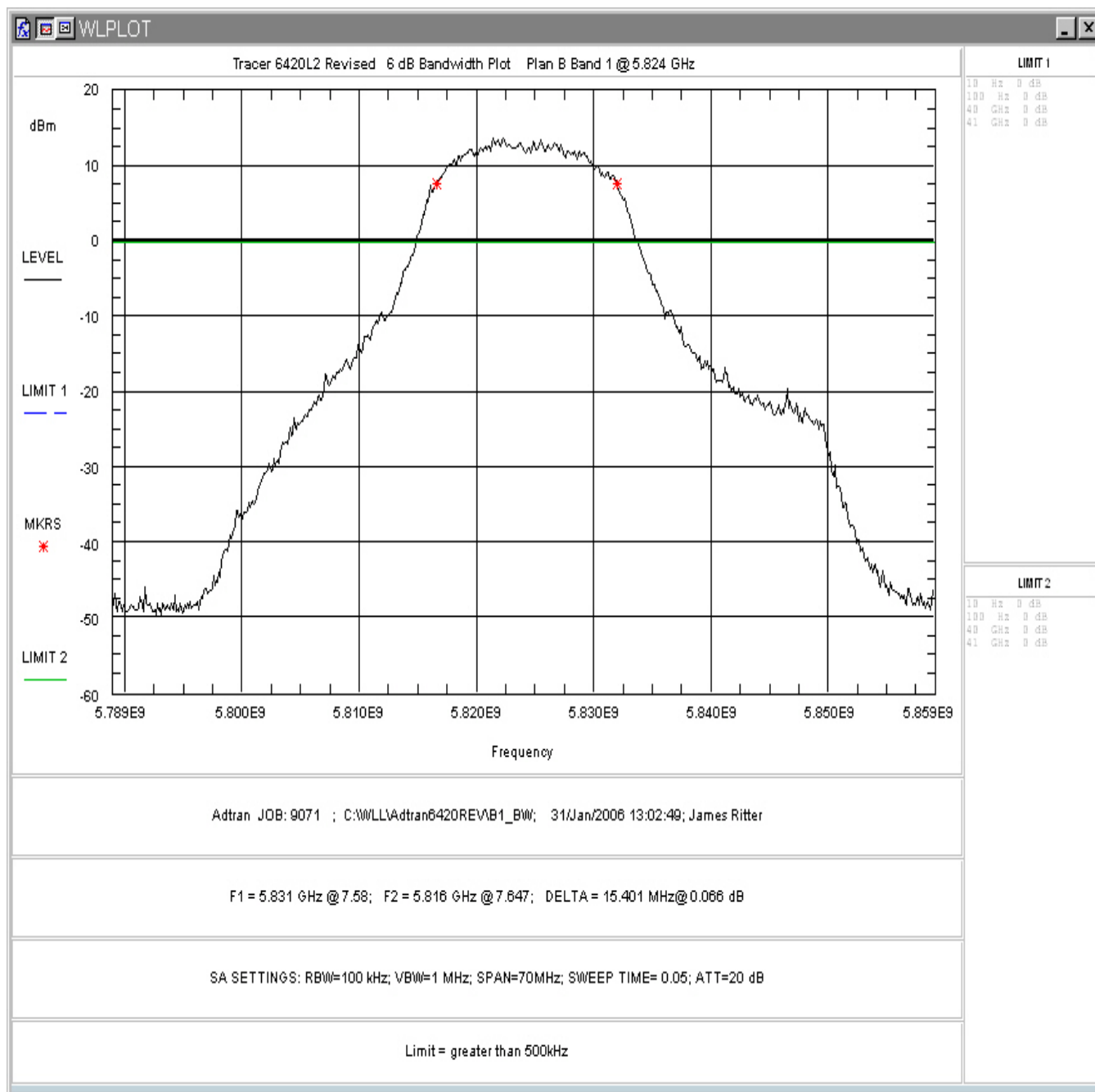
Figure 4. Occupied Bandwidth - Plan B, Band 1
