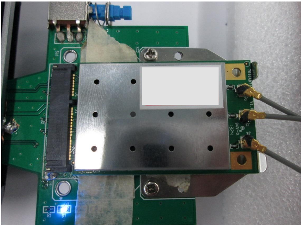
Conducted Test_Ant 2
