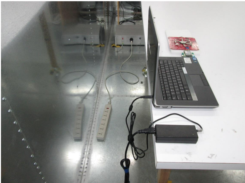
Conducted Test_Ant 2
