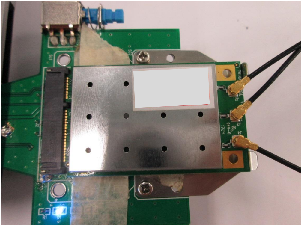
Conducted Test_Ant 1
