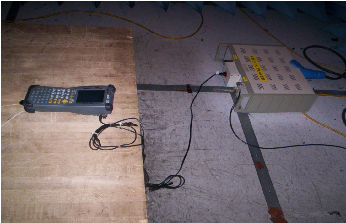
Power line conducted emissions
