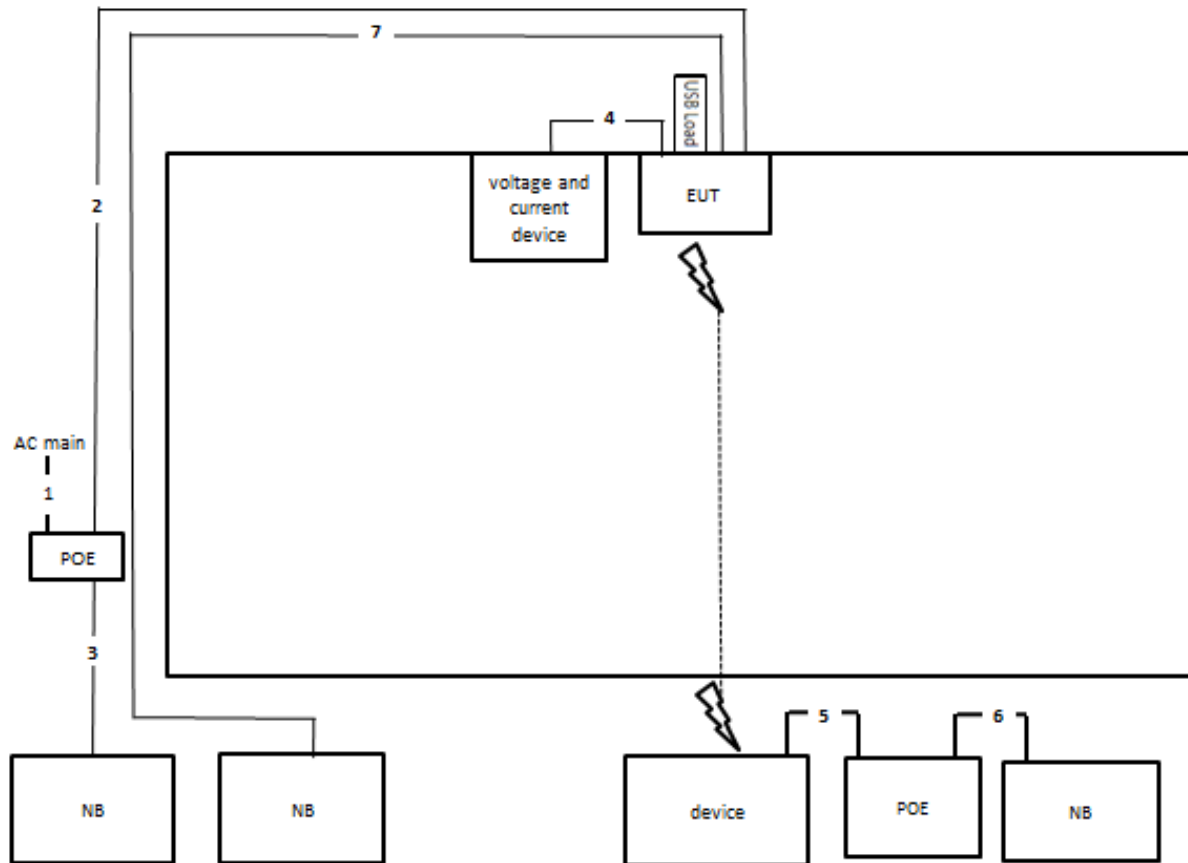
Test Setup Diagram - Transmitter Spurious Emissions below 1 GHz
