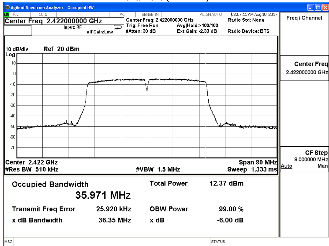
Channel 3 (2422MHz)
