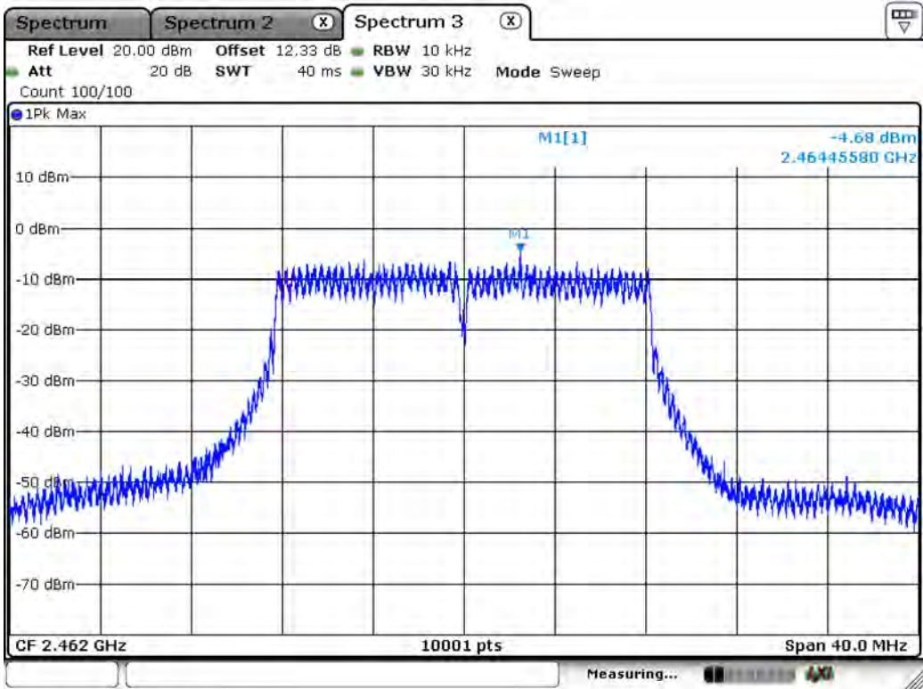
Channel 11 (2462MHz)
