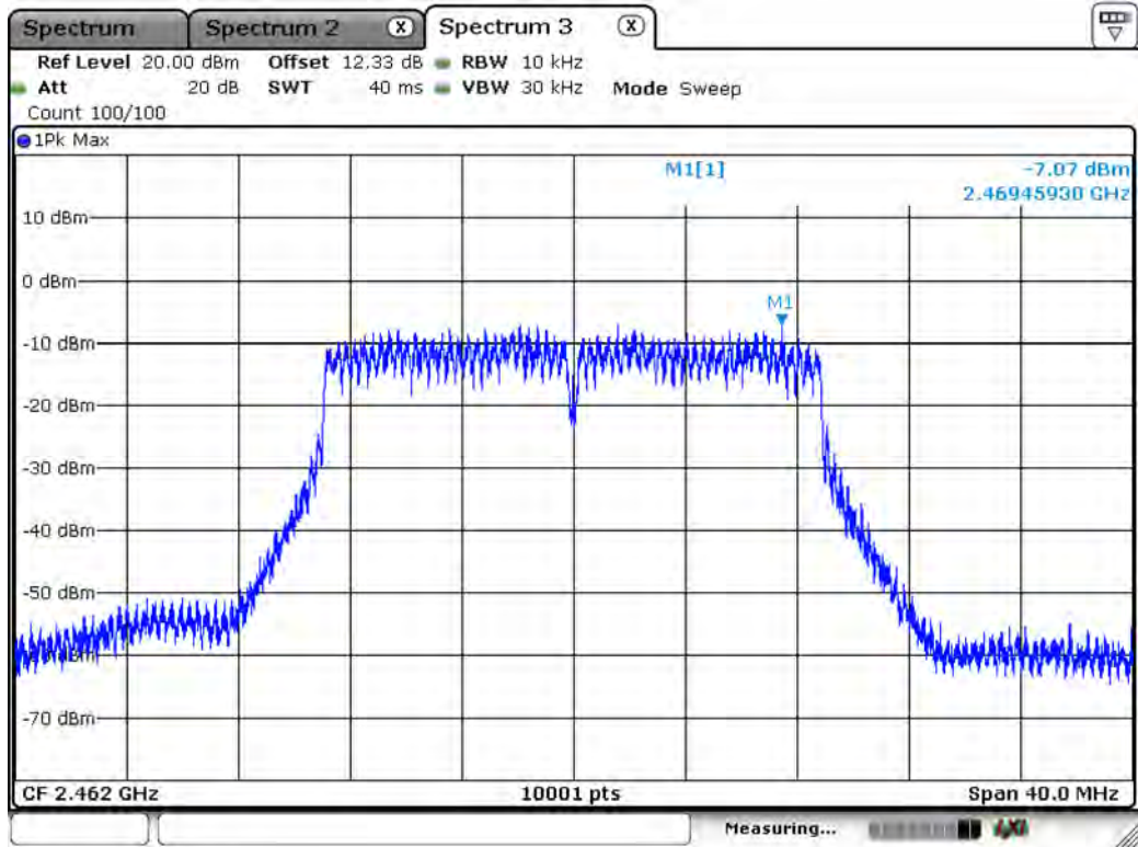
Channel 11 (2462MHz)
