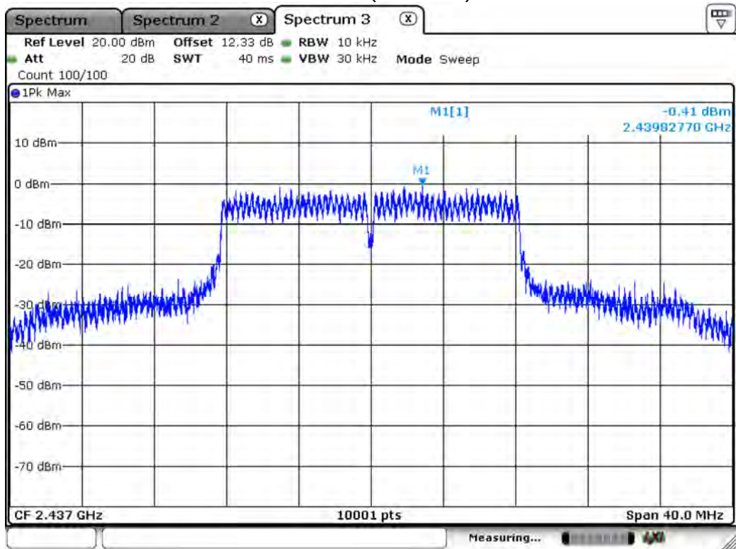
Channel 6 (2437MHz)
