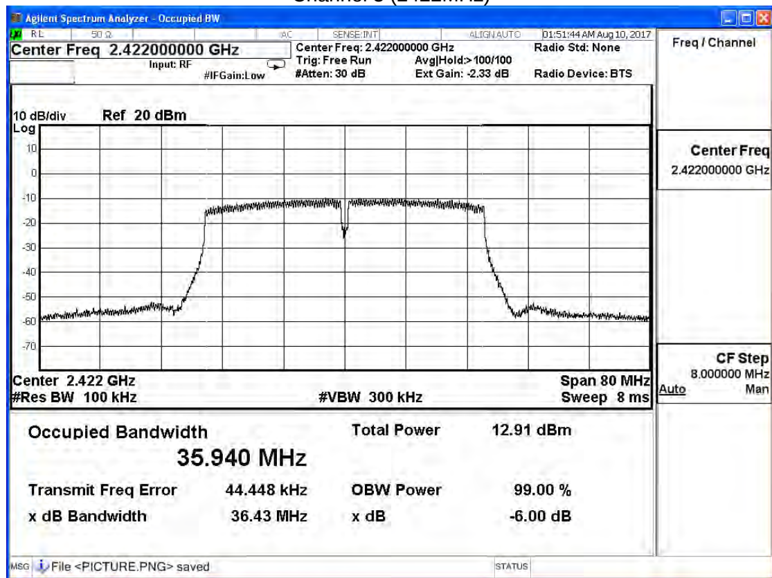
Channel 3 (2422MHz)
