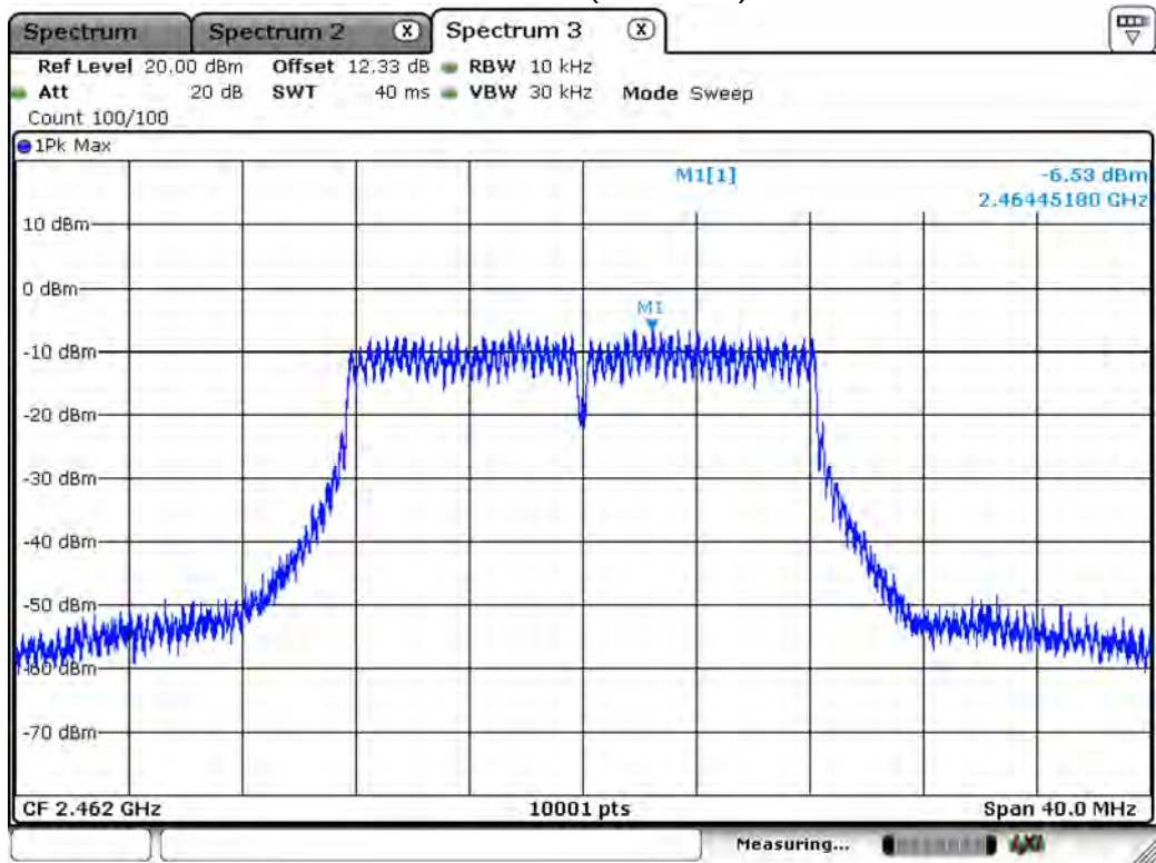
Channel 11 (2462MHz)
