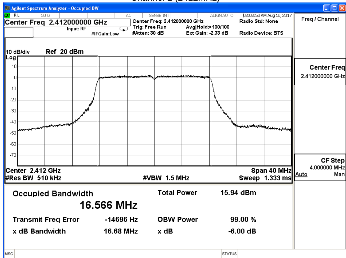
Channel 1 (2412MHz)
