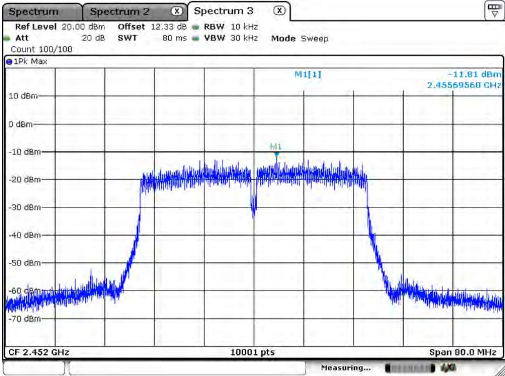
Channel 9 (2452MHz)
