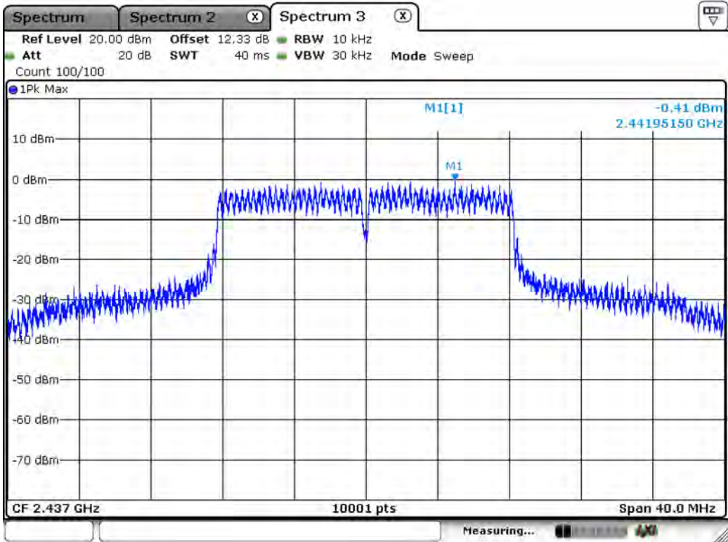
Channel 6 (2437MHz)
