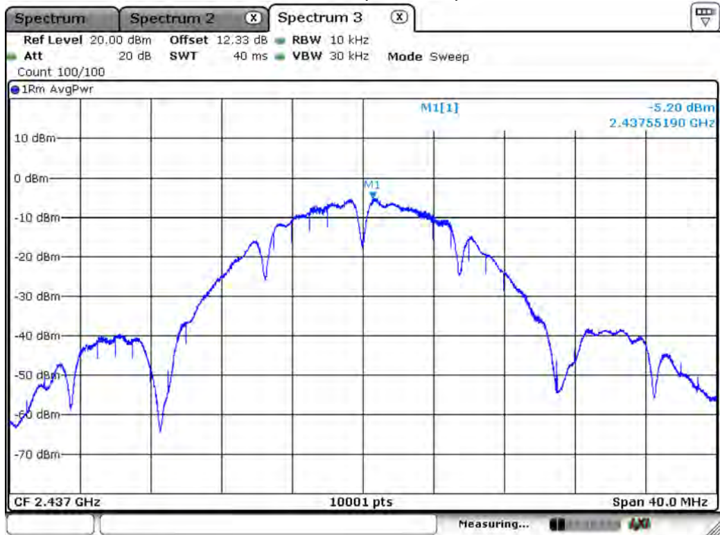
Channel 6 (2437MHz)
