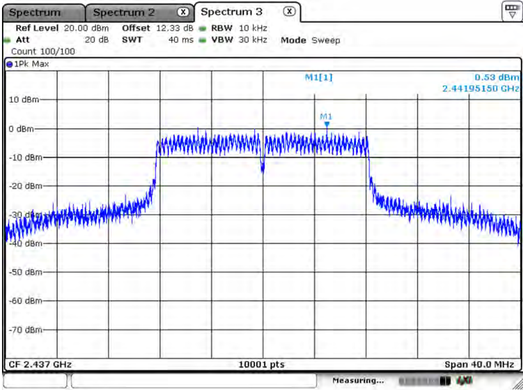
Channel 6 (2437MHz)
