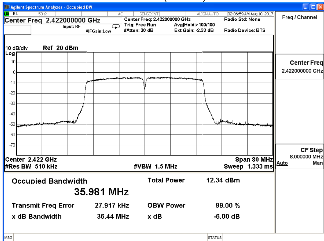
Channel 3 (2422MHz)
